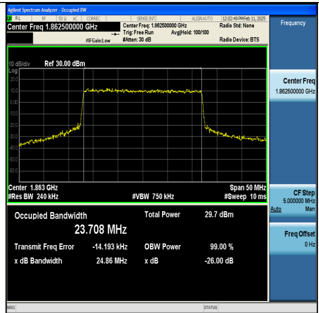
NTNV-n25-PC3-15-25-L-CP-QPSK-Outer_Full-Ant1-PASS
