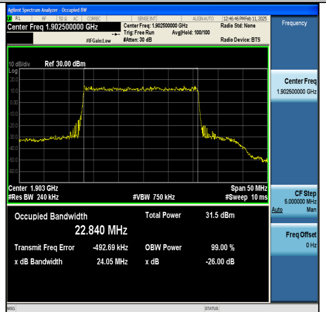
NTNV-n25-PC3-15-25-H-DFT-QPSK-Outer_Full-Ant1- PASS
