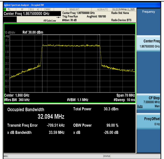
NTNV-n25-PC3-15-35-L-DFT-64QAM-Outer_Full-Ant1- PASS
