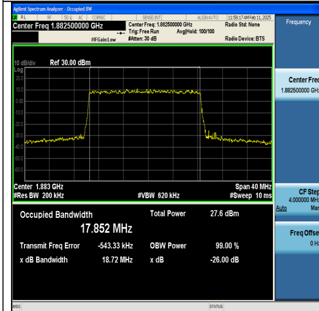
NTNV-n25-PC3-15-20-M-DFT-256QAM-Outer_Full-Ant1- PASS
