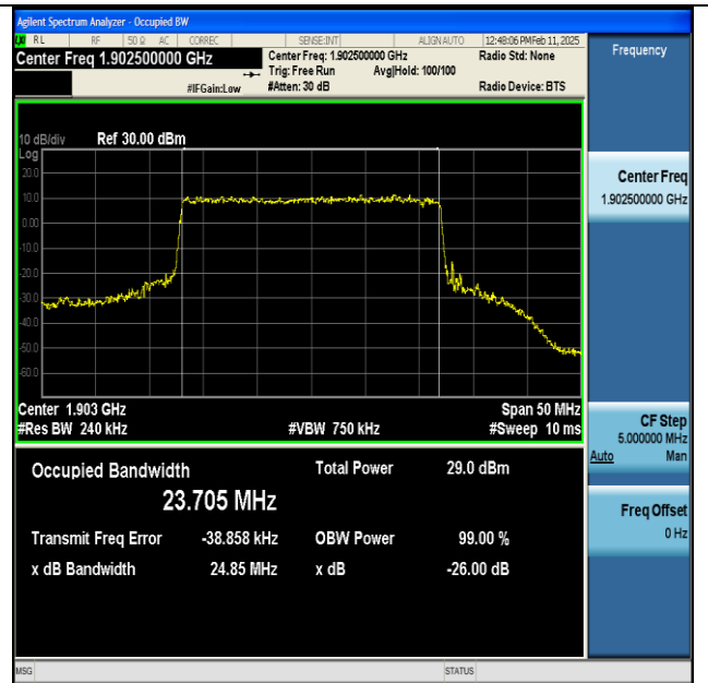
NTNV-n25-PC3-15-25-H-CP-64QAM-Outer_Full-Ant1- PASS
