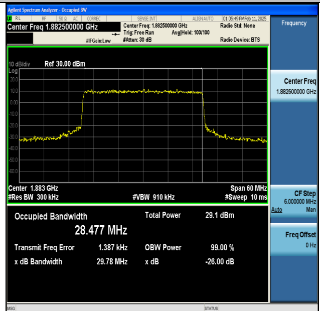
NTNV-n25-PC3-15-30-M-CP-64QAM-Outer_Full-Ant1-PASS
