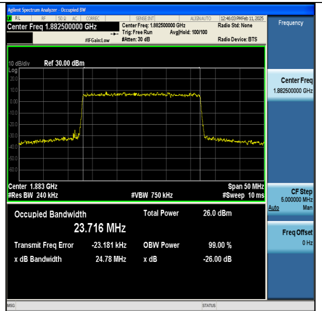
NTNV-n25-PC3-15-25-M-CP-256QAM-Outer_Full-Ant1- PASS
