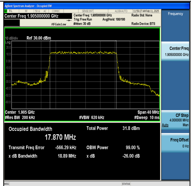
NTNV-n25-PC3-15-20-H-DFT-BPSK-Outer_Full-Ant1- PASS
