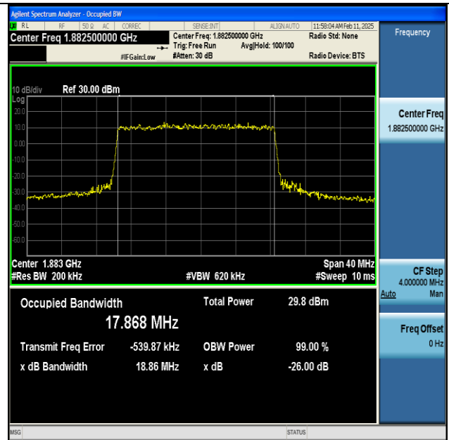
NTNV-n25-PC3-15-20-M-DFT-64QAM-Outer_Full-Ant1- PASS
