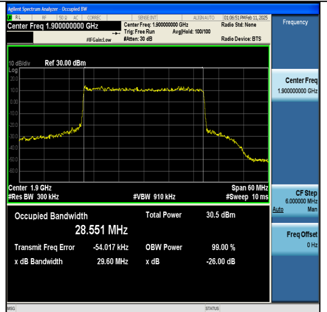
NTNV-n25-PC3-15-30-H-DFT-16QAM-Outer_Full-Ant1- PASS
