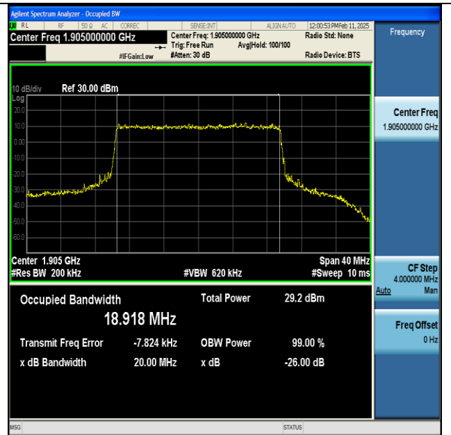
NTNV-n25-PC3-15-20-H-CP-16QAM-Outer_Full-Ant1-PASS
