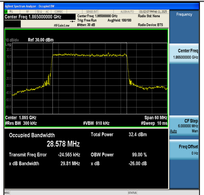
NTNV-n25-PC3-15-30-L-DFT-BPSK-Outer_Full-Ant1- PASS
