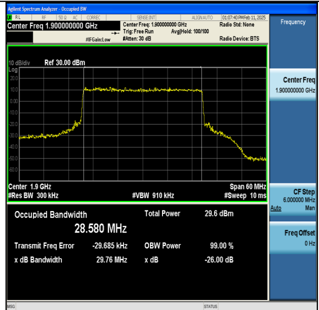
NTNV-n25-PC3-15-30-H-CP-16QAM-Outer_Full-Ant1- PASS
