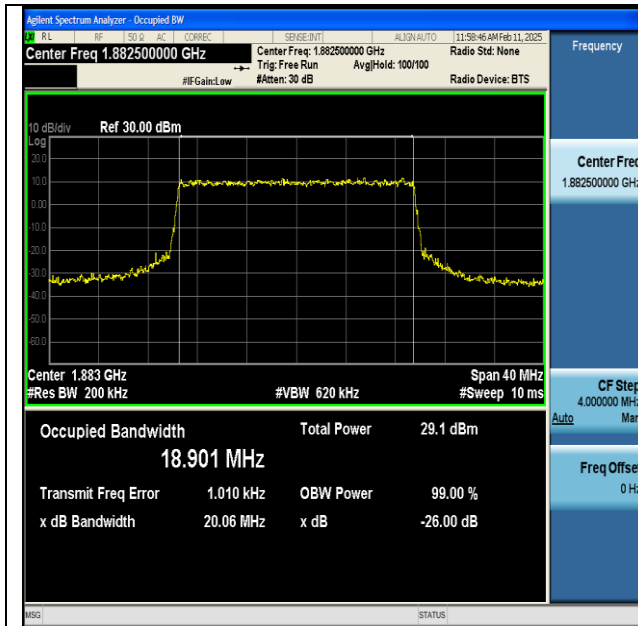
NTNV-n25-PC3-15-20-M-CP-16QAM-Outer_Full-Ant1- PASS
