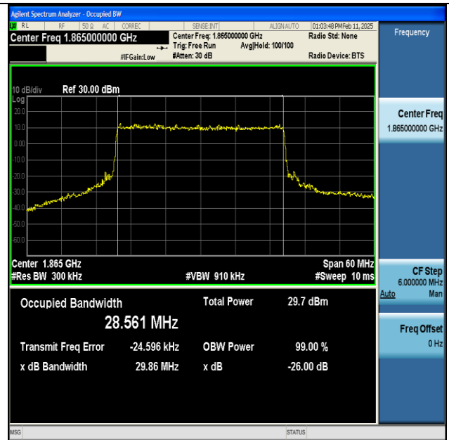
NTNV-n25-PC3-15-30-L-CP-16QAM-Outer_Full-Ant1-PASS
