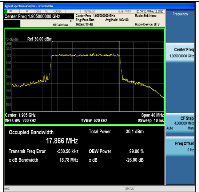
NTNV-n25-PC3-15-20-H-DFT-16QAM-Outer_Full-Ant1- PASS
