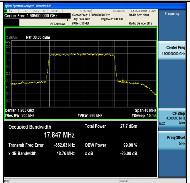
NTNV-n25-PC3-15-20-H-DFT-256QAM-Outer_Full-Ant1- PASS
