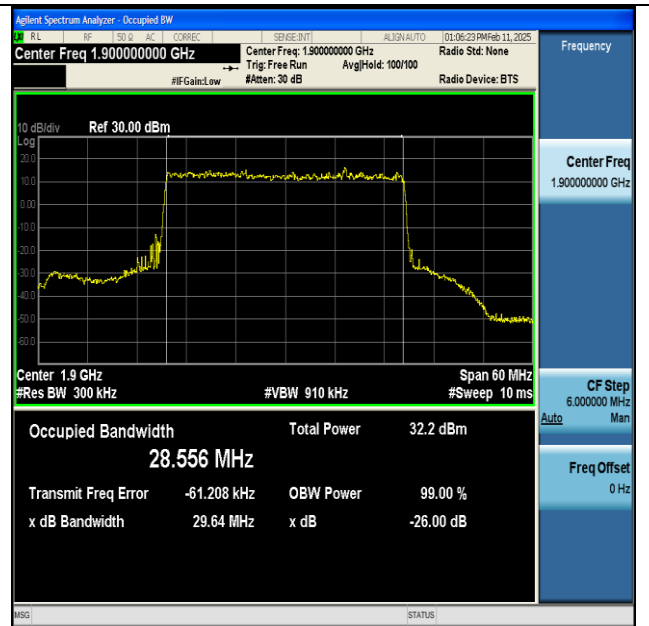
NTNV-n25-PC3-15-30-H-DFT-BPSK-Outer_Full-Ant1- PASS
