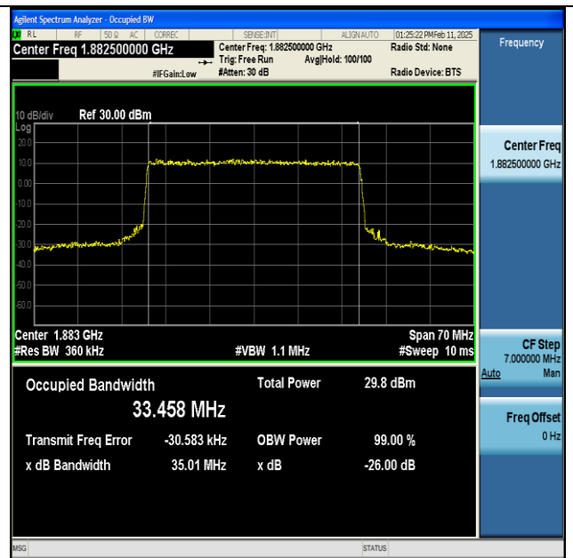
NTNV-n25-PC3-15-35-M-CP-16QAM-Outer_Full-Ant1-PASS
