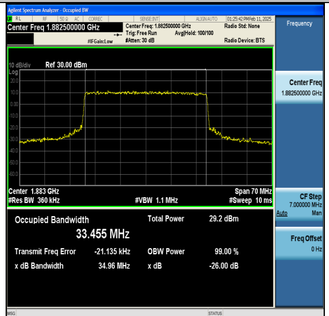
NTNV-n25-PC3-15-35-M-CP-256QAM-Outer_Full-Ant1-PASS
