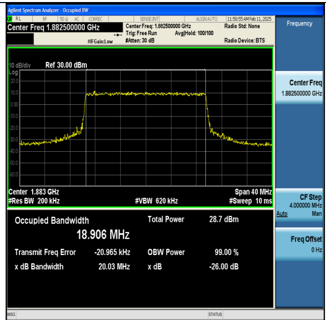
NTNV-n25-PC3-15-20-M-CP-64QAM-Outer_Full-Ant1- PASS
