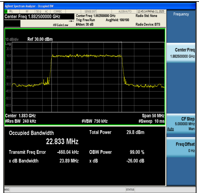
NTNV-n25-PC3-15-25-M-DFT-256QAM-Outer_Full-Ant1- PASS
