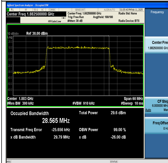
NTNV-n25-PC3-15-30-M-CP-16QAM-Outer_Full-Ant1-PASS
