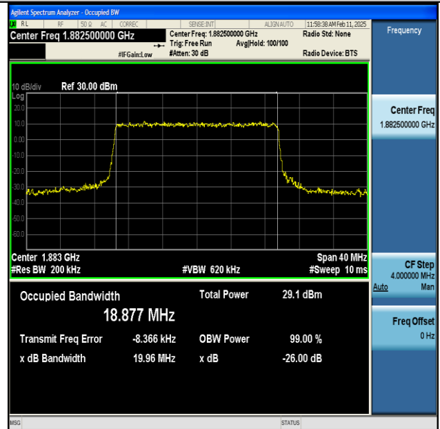
NTNV-n25-PC3-15-20-M-DFT-64QAM-Outer_Full-Ant1- PASS
