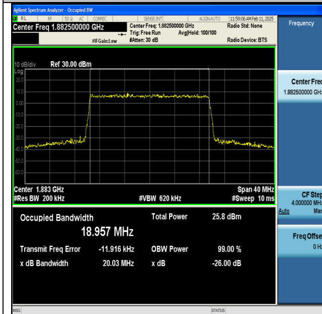
NTNV-n25-PC3-15-20-M-CP-256QAM-Outer_Full-Ant1- PASS
