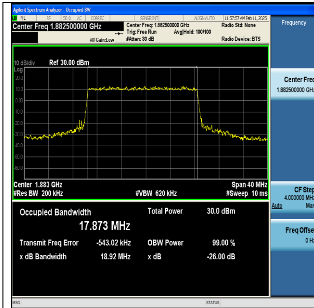
NTNV-n25-PC3-15-20-M-DFT-16QAM-Outer_Full-Ant1- PASS
