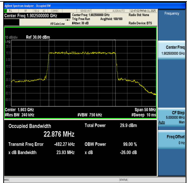
NTNV-n25-PC3-15-25-H-DFT-64QAM-Outer_Full-Ant1- PASS
