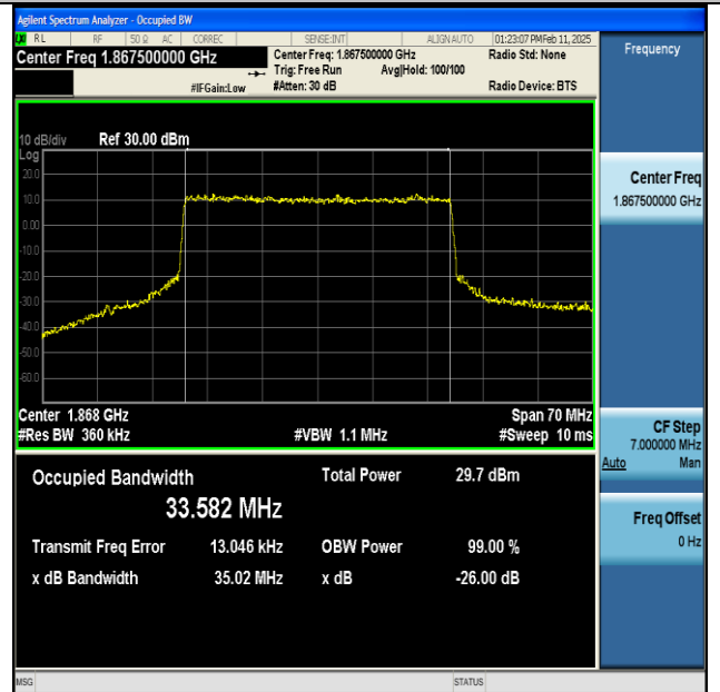
NTNV-n25-PC3-15-35-L-DFT-64QAM-Outer_Full-Ant1- PASS
