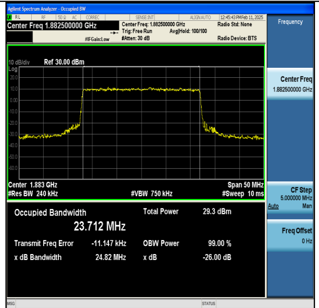
NTNV-n25-PC3-15-25-M-CP-16QAM-Outer_Full-Ant1- PASS
