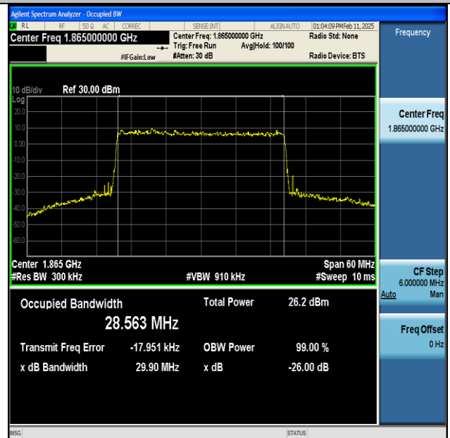
NTNV-n25-PC3-15-30-L-CP-256QAM-Outer_Full-Ant1-PASS
