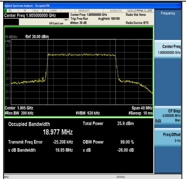
NTNV-n25-PC3-15-20-H-CP-256QAM-Outer_Full-Ant1-PASS
