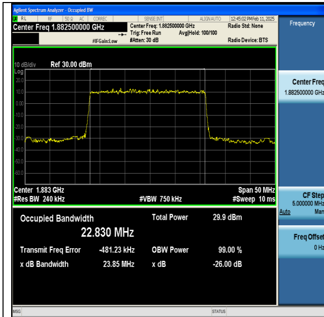
NTNV-n25-PC3-15-25-M-DFT-64QAM-Outer_Full-Ant1- PASS
