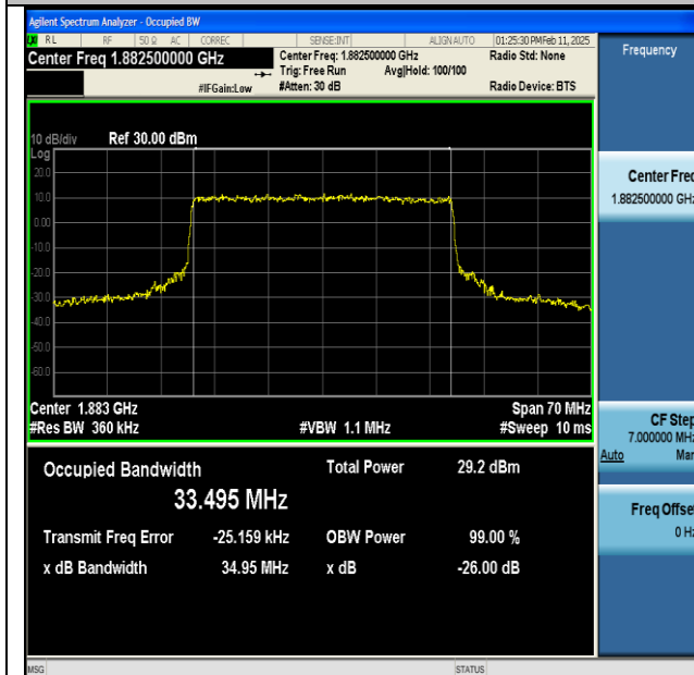
NTNV-n25-PC3-15-35-M-CP-64QAM-Outer_Full-Ant1-PASS
