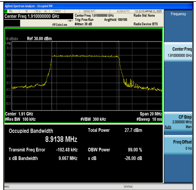
NTNV-n25-PC3-15-10-H-DFT-256QAM-Outer_Full-Ant1- PASS
