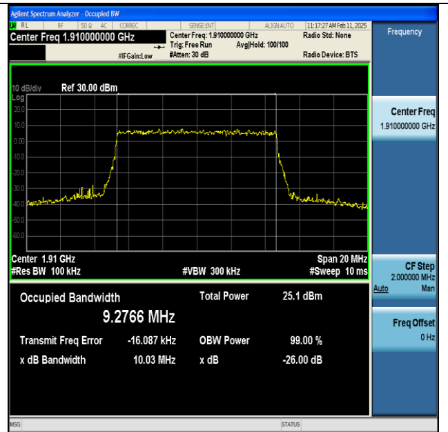
NTNV-n25-PC3-15-10-H-CP-256QAM-Outer_Full-Ant1- PASS
