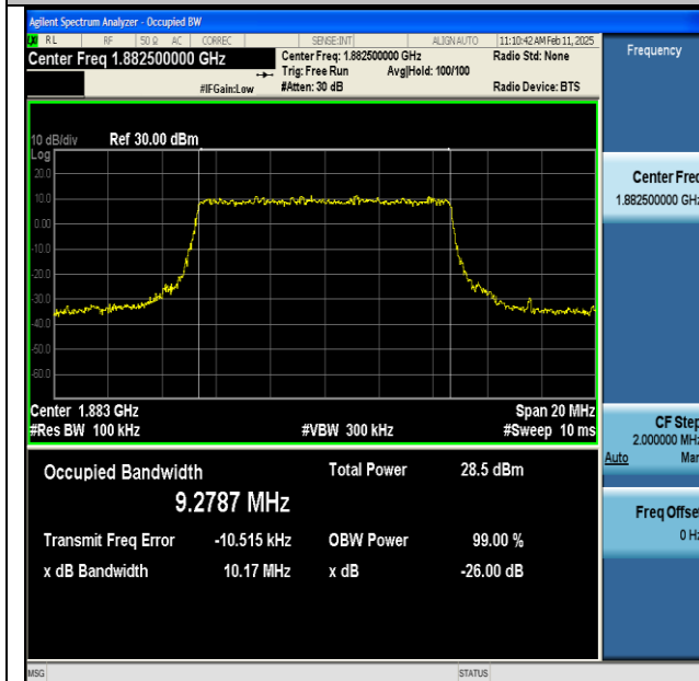
NTNV-n25-PC3-15-10-M-CP-16QAM-Outer_Full-Ant1-PASS
