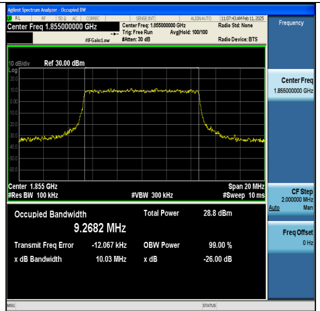
NTNV-n25-PC3-15-10-L-CP-16QAM-Outer_Full-Ant1-PASS
