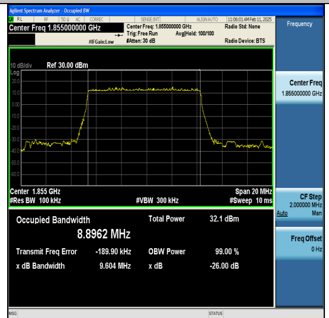
NTNV-n25-PC3-15-10-L-DFT-BPSK-Outer_Full-Ant1-PASS
