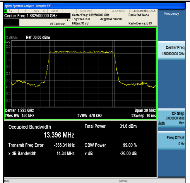
NTNV-n25-PC3-15-15-M-DFT-BPSK-Outer_Full-Ant1- PASS
