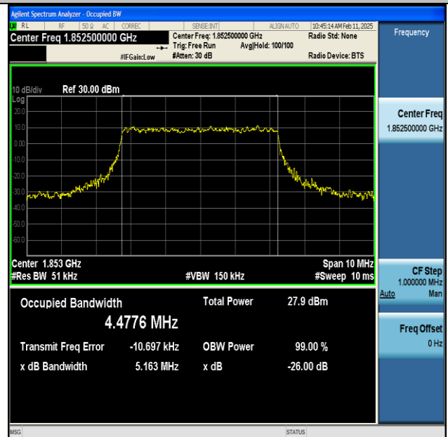
NTNV-n25-PC3-15-5-L-CP-64QAM-Outer_Full-Ant1-PASS
