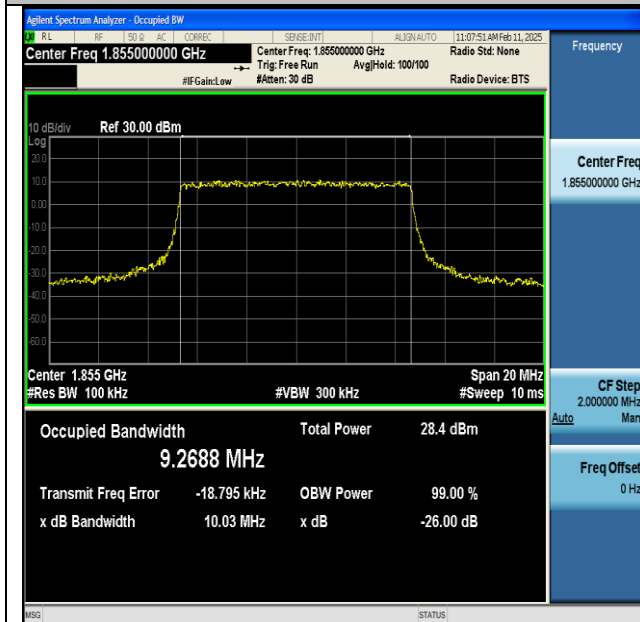
NTNV-n25-PC3-15-10-L-CP-64QAM-Outer_Full-Ant1-PASS
