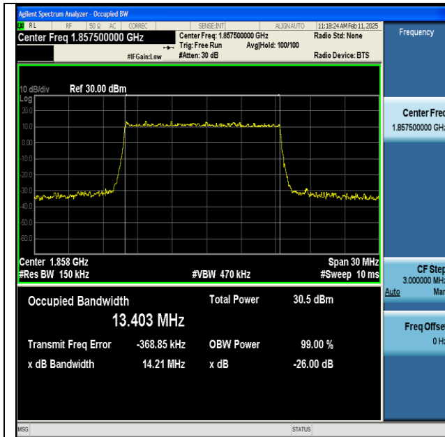
NTNV-n25-PC3-15-15-L-DFT-16QAM-Outer_Full-Ant1- PASS
