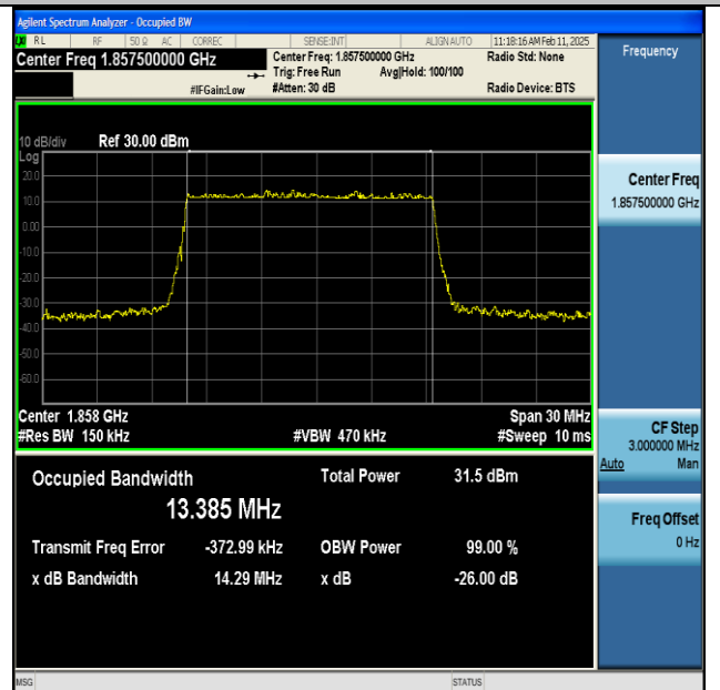
NTNV-n25-PC3-15-15-L-DFT-QPSK-Outer_Full-Ant1- PASS
