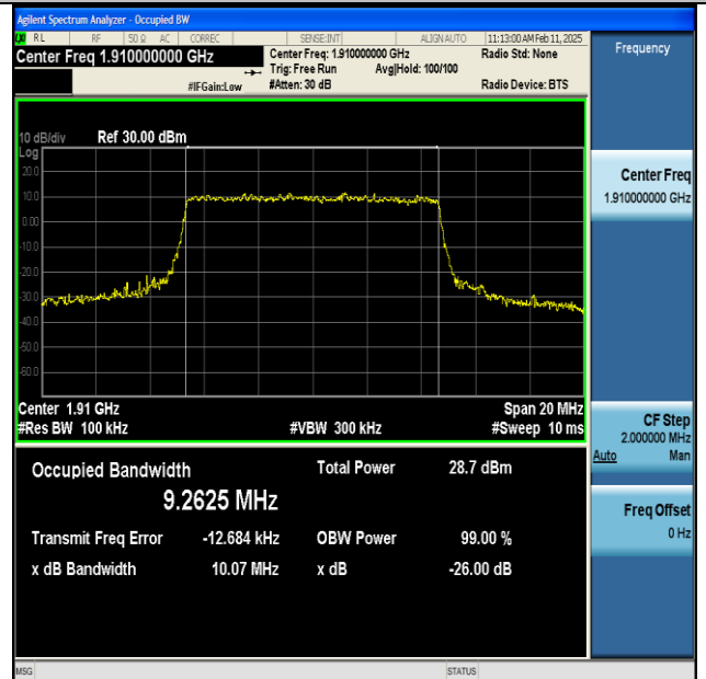
NTNV-n25-PC3-15-10-H-CP-16QAM-Outer_Full-Ant1- PASS
