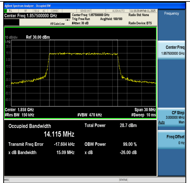
NTNV-n25-PC3-15-15-L-CP-64QAM-Outer_Full-Ant1- PASS
