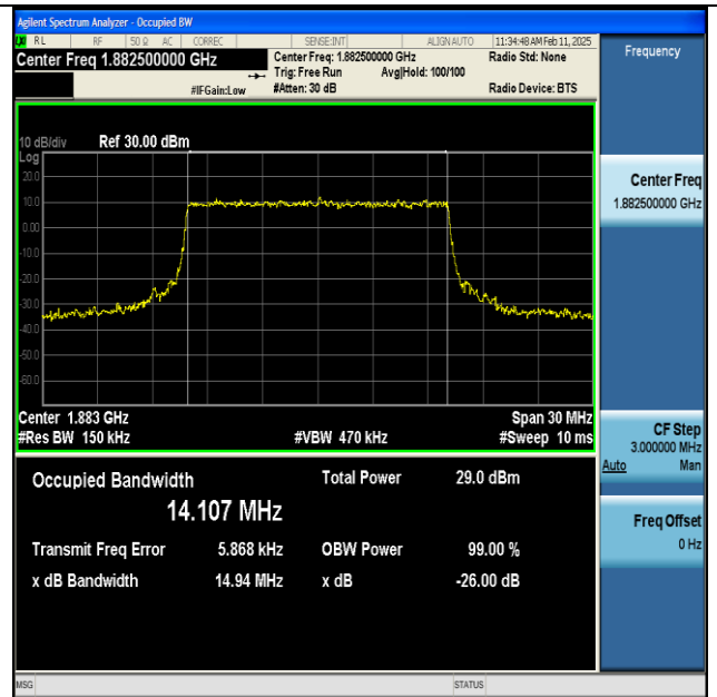
NTNV-n25-PC3-15-15-M-CP-16QAM-Outer_Full-Ant1-PASS
