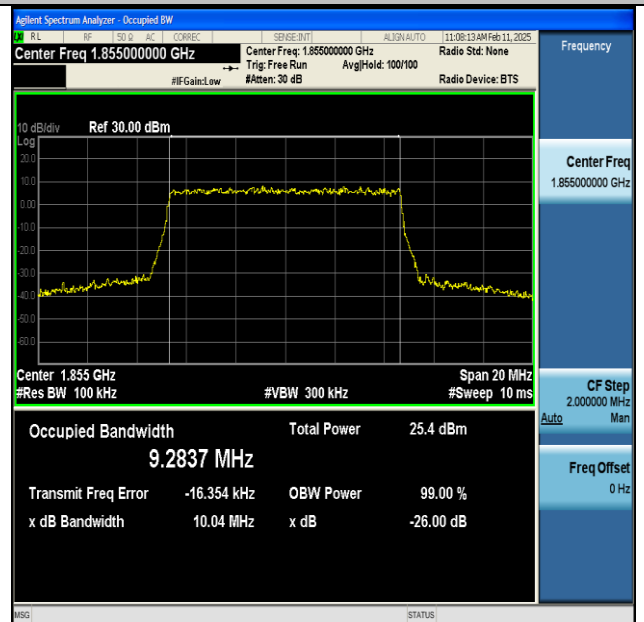
NTNV-n25-PC3-15-10-L-CP-256QAM-Outer_Full-Ant1-PASS
