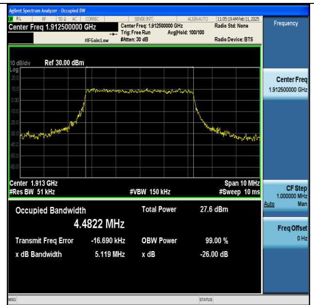
NTNV-n25-PC3-15-5-H-CP-64QAM-Outer_Full-Ant1-PASS
