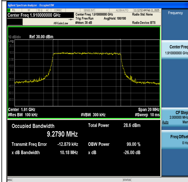
NTNV-n25-PC3-15-10-H-DFT-64QAM-Outer_Full-Ant1- PASS
