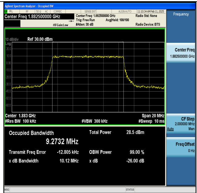
NTNV-n25-PC3-15-10-M-CP-QPSK-Outer_Full-Ant1-PASS
