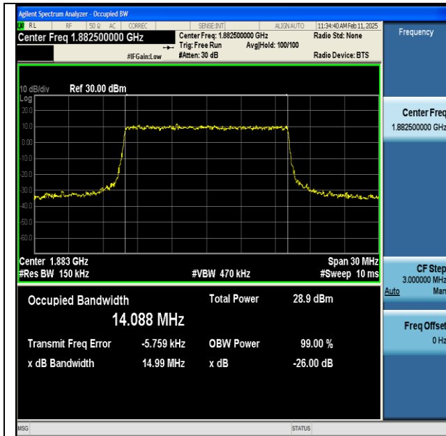
NTNV-n25-PC3-15-15-M-CP-QPSK-Outer_Full-Ant1-PASS
