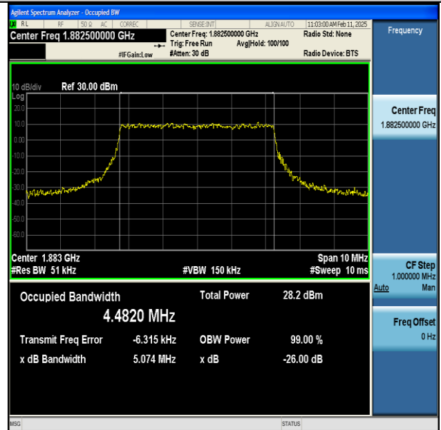
NTNV-n25-PC3-15-5-M-CP-16QAM-Outer_Full-Ant1- PASS
