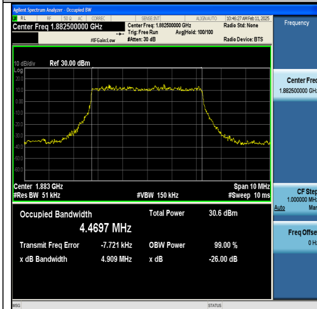
NTNV-n25-PC3-15-5-L-CP-256QAM-Outer_Full-Ant1-PASS
