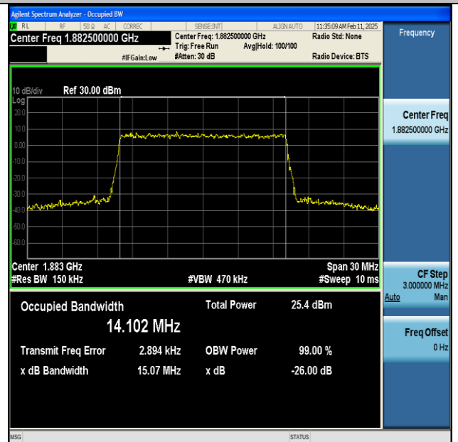
NTNV-n25-PC3-15-15-M-CP-256QAM-Outer_Full-Ant1-PASS
