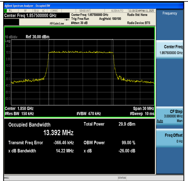
NTNV-n25-PC3-15-15-L-DFT-64QAM-Outer_Full-Ant1- PASS
