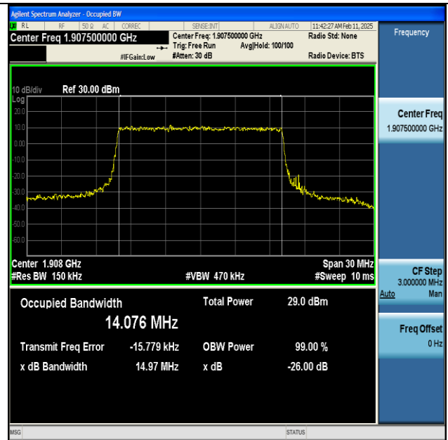
NTNV-n25-PC3-15-15-H-CP-QPSK-Outer_Full-Ant1-PASS
