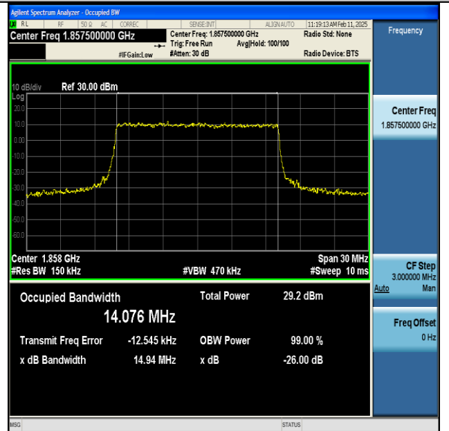
NTNV-n25-PC3-15-15-L-DFT-64QAM-Outer_Full-Ant1- PASS
