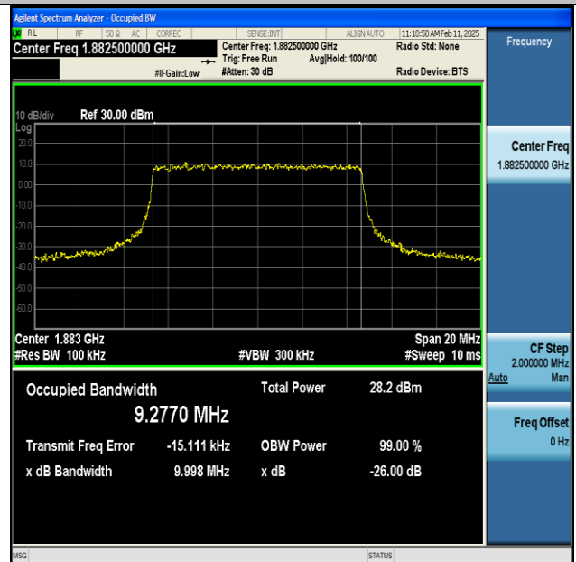
NTNV-n25-PC3-15-10-M-CP-64QAM-Outer_Full-Ant1-PASS
