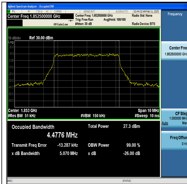
NTNV-n25-PC3-15-5-L-DFT-256QAM-Outer_Full-Ant1-PASS
