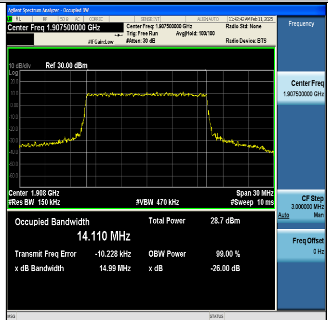
NTNV-n25-PC3-15-15-H-CP-64QAM-Outer_Full-Ant1-PASS
