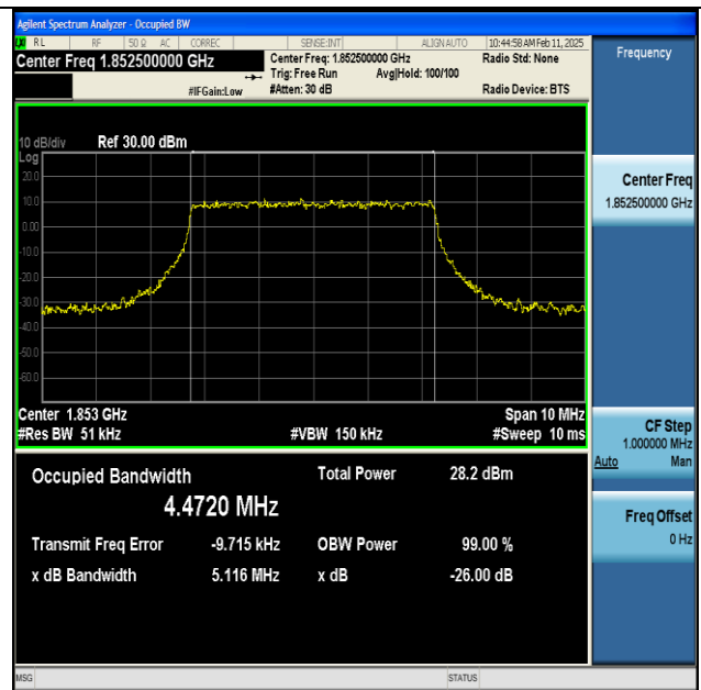
NTNV-n25-PC3-15-5-L-CP-QPSK-Outer_Full-Ant1-PASS
