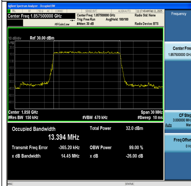
NTNV-n25-PC3-15-15-L-DFT-BPSK-Outer_Full-Ant1- PASS
