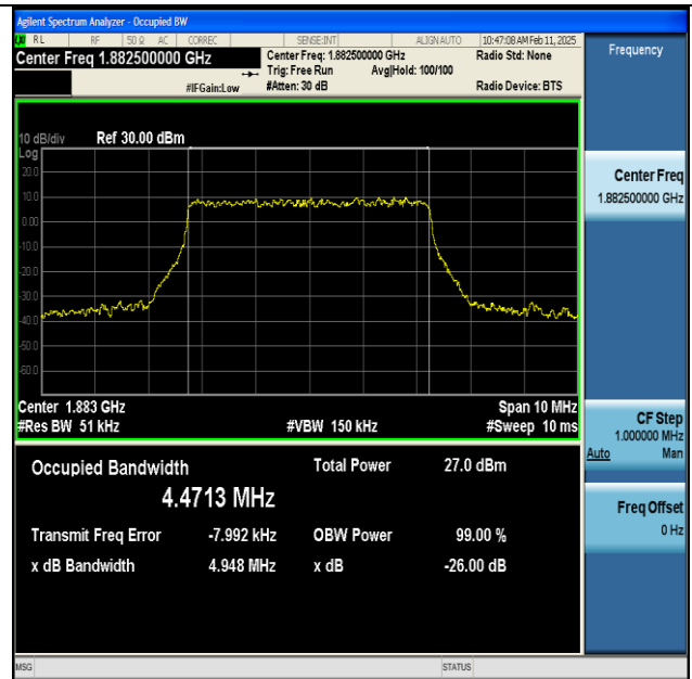
NTNV-n25-PC3-15-5-M-DFT-256QAM-Outer_Full-Ant1- PASS
