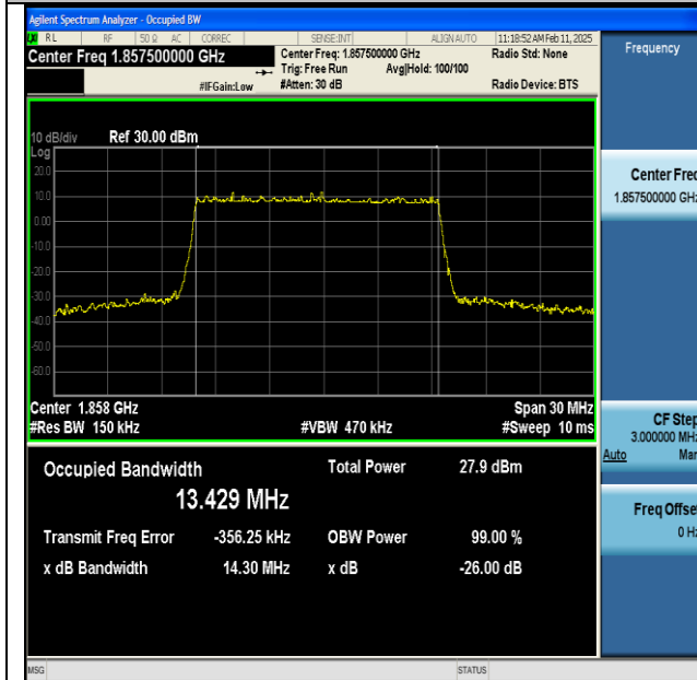
NTNV-n25-PC3-15-15-L-DFT-256QAM-Outer_Full-Ant1- PASS
