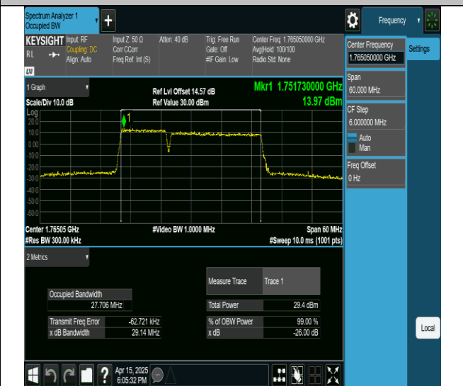
66-66-10MHz-20MHz-16QAM-16QAM-132428-132572-50RB#0-100RB#0-PASS
