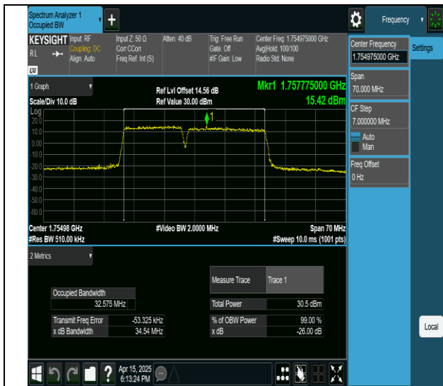
66-66-15MHz-20MHz-QPSK-QPSK-132325-132496-75RB#0-100RB#0-PASS
