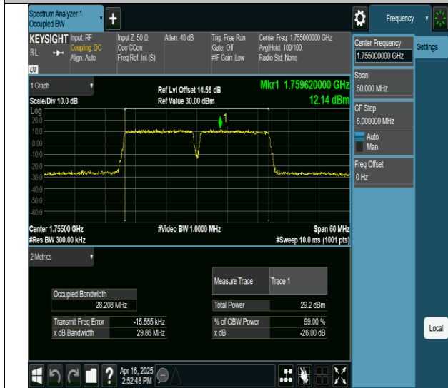
66-66-15MHz-15MHz-64QAM-64QAM-132347-132497-75RB#0-75RB#0-PASS
