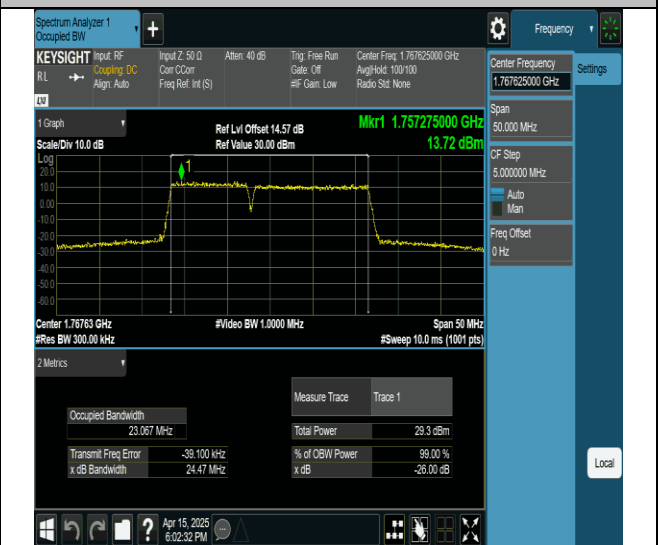
66-66-10MHz-15MHz-16QAM-16QAM-132477-132597-50RB#0-75RB#0-PASS
