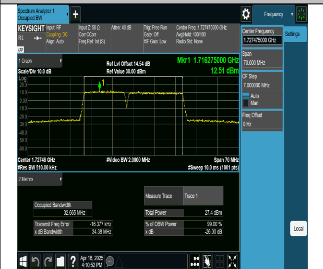
66-66-15MHz-20MHz-256QAM-256QAM-132050-132221- 75RB#0-100RB#0-PASS
