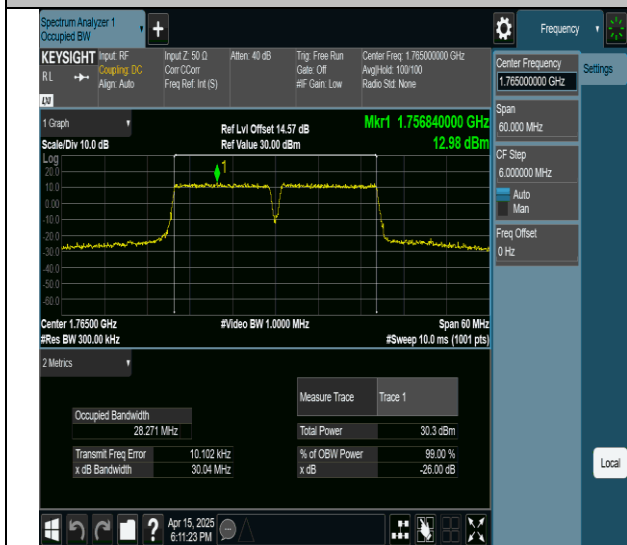
66-66-15MHz-15MHz-QPSK-QPSK-132447-132597-75RB#0-75RB#0-PASS
