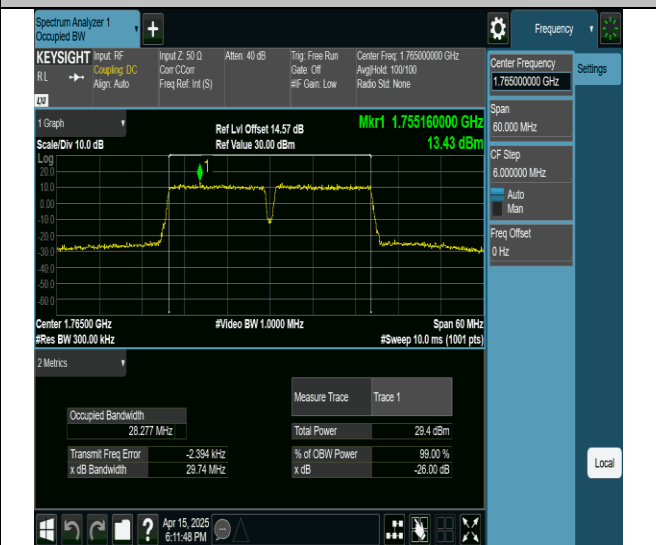
66-66-15MHz-15MHz-16QAM-16QAM-132447-132597-75RB#0-75RB#0-PASS
