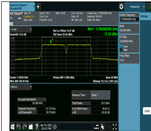
66-66-15MHz-15MHz-64QAM-64QAM-132447-132597-75RB#0- 75RB#0-PASS
