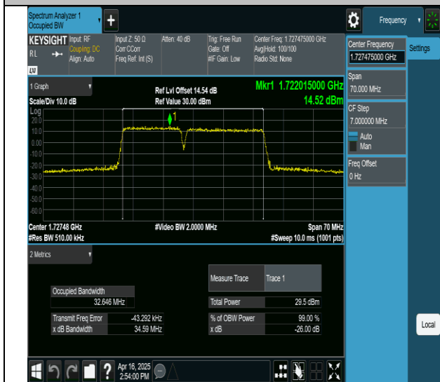
66-66-15MHz-20MHz-64QAM-64QAM-132050-132221-75RB#0- 100RB#0-PASS
