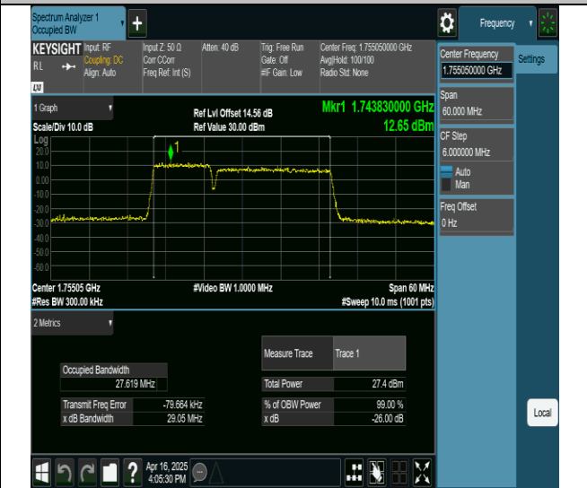
66-66-10MHz-20MHz-256QAM-256QAM-132328-132472-50RB#0-100RB#0-PASS
