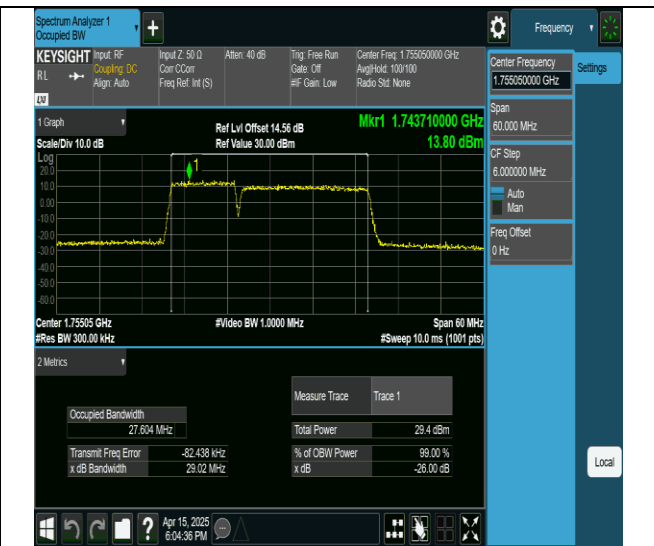
66-66-10MHz-20MHz-16QAM-16QAM-132328-132472-50RB#0-100RB#0-PASS
