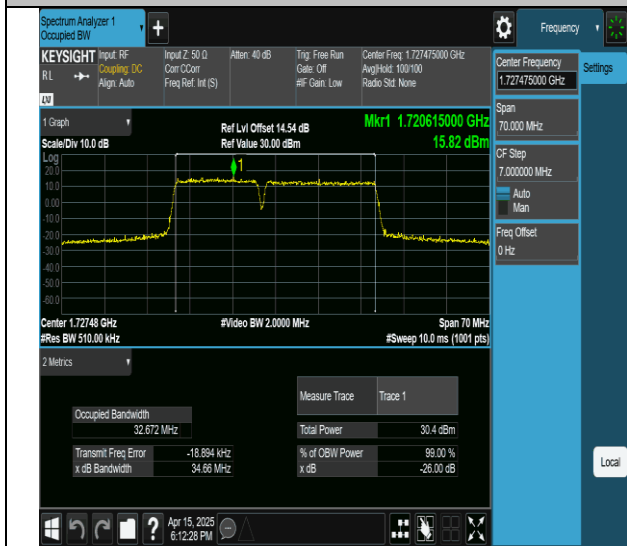
66-66-15MHz-20MHz-QPSK-QPSK-132050-132221-75RB#0- 100RB#0-PASS
