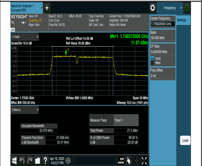
66-66-10MHz-15MHz-256QAM-256QAM-132351-132471-50RB#0-75RB#0-PASS
