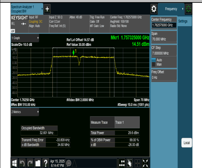
66-66-15MHz-20MHz-16QAM-16QAM-132401-132572-75RB#0-100RB#0-PASS
