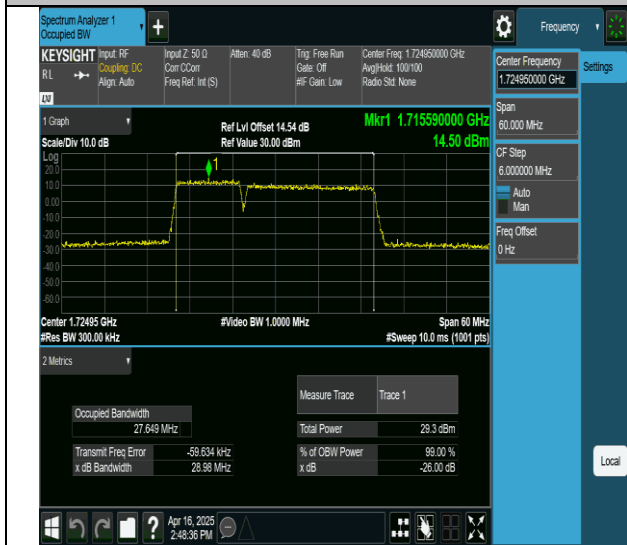
66-66-10MHz-20MHz-64QAM-64QAM-132027-132171-50RB#0-100RB#0-PASS
