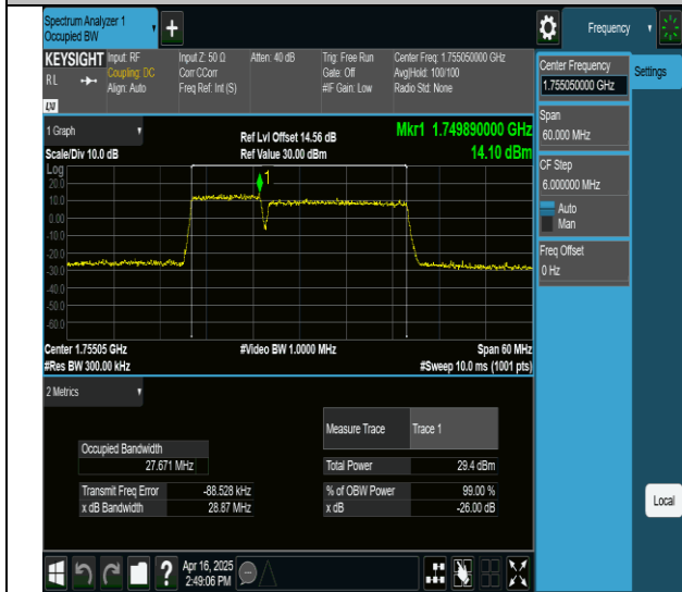
66-66-10MHz-20MHz-64QAM-64QAM-132328-132472-50RB#0-100RB#0-PASS
