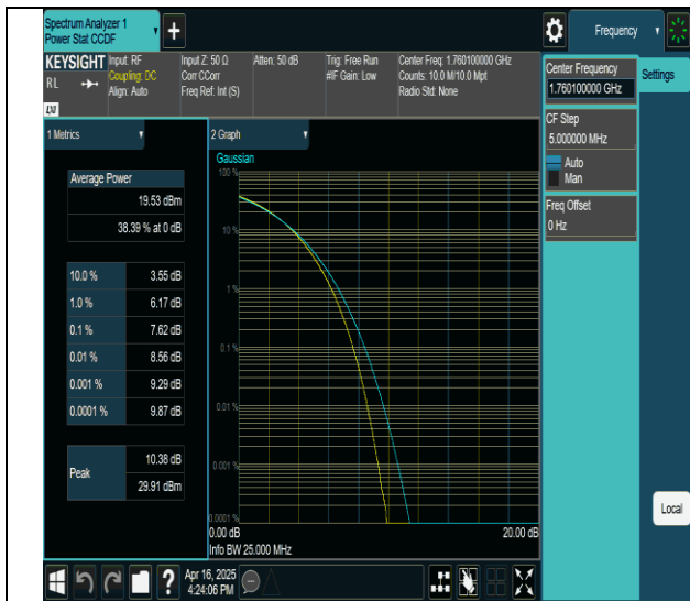
66-66-20MHz-20MHz-64QAM-64QAM-132374-132572-100RB#0- 100RB#0-PASS
