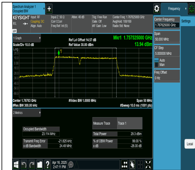
66-66-10MHz-15MHz-64QAM-64QAM-132477-132597-50RB#0-75RB#0-PASS
