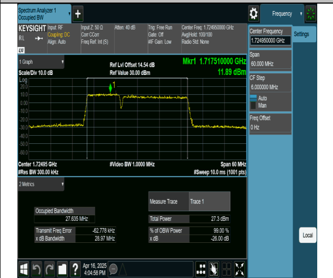
66-66-10MHz-20MHz-256QAM-256QAM-132027-132171-50RB#0-100RB#0-PASS
