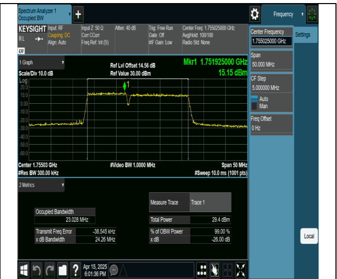
66-66-10MHz-15MHz-16QAM-16QAM-132351-132471-50RB#0-75RB#0-PASS
