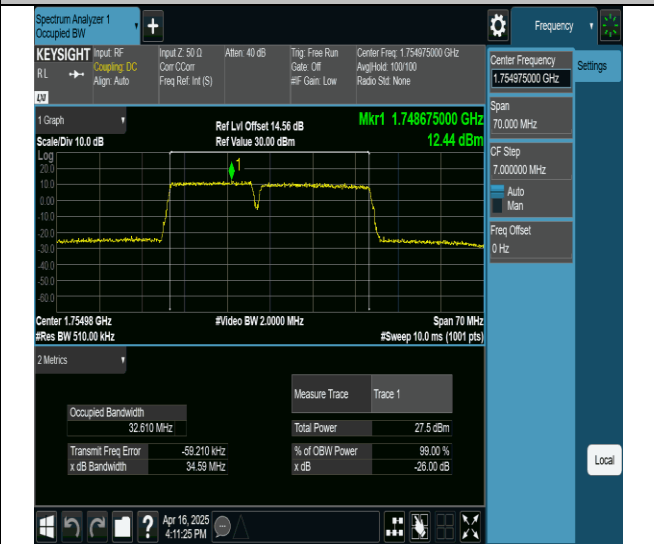
66-66-15MHz-20MHz-256QAM-256QAM-132325-132496-75RB#0-100RB#0-PASS
