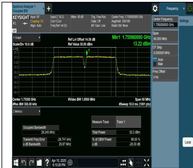
66-66-15MHz-15MHz-QPSK-QPSK-132347-132497-75RB#0-75RB#0-PASS
