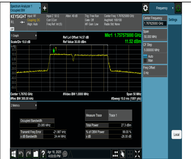
66-66-10MHz-15MHz-256QAM-256QAM-132477-132597-50RB#0-75RB#0-PASS
