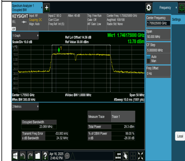
66-66-10MHz-15MHz-64QAM-64QAM-132351-132471-50RB#0-75RB#0-PASS
