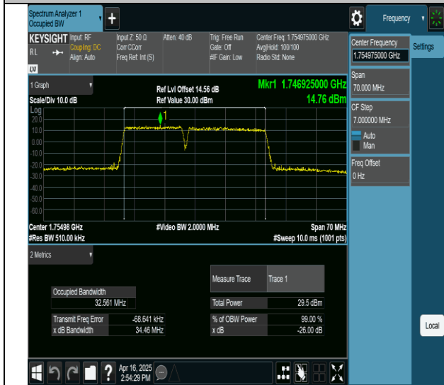
66-66-15MHz-20MHz-64QAM-64QAM-132325-132496-75RB#0-100RB#0-PASS
