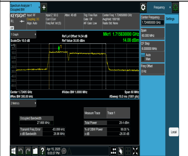
66-66-10MHz-20MHz-16QAM-16QAM-132027-132171-50RB#0-100RB#0-PASS
