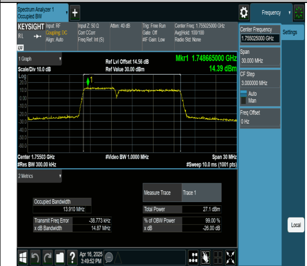
66-66-5MHz-10MHz-256QAM-256QAM-132375-132447-25RB#0-50RB#0-PASS
