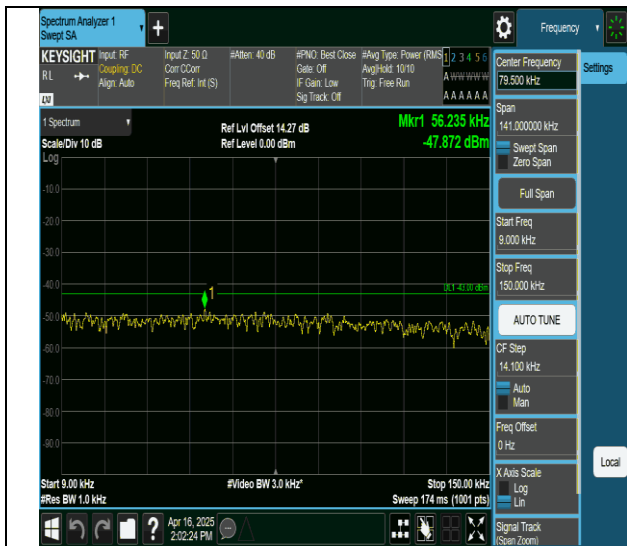
66-66-10MHz-10MHz-QPSK-QPSK-132523-132622-1RB#0- ORB#0-0.009~0.15MHz-PASS
