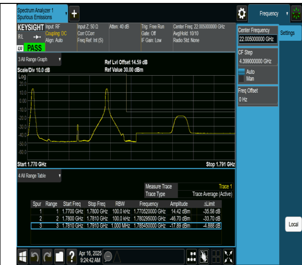
66-66-5MHz-5MHz-QPSK@QPSK-QPSK@QPSK-132599- 132647-1RB#0@0RB#0-1RB#15@0RB#0-PASS
