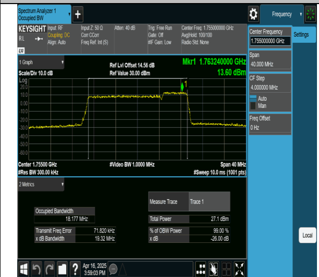
66-66-15MHz-5MHz-256QAM-256QAM-132398-132491-75RB#0-25RB#0-PASS
