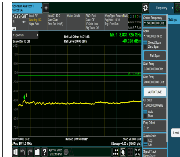
66-66-10MHz-10MHz-QPSK-QPSK-132022-132121-1RB#0- ORB#0-3000~20000MHz-PASS
