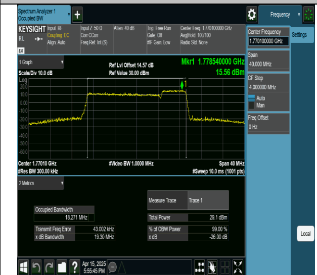
66-66-15MHz-5MHz-16QAM-16QAM-132549-132642-75RB#0-25RB#0-PASS
