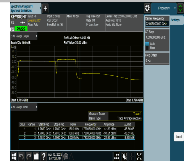
66-66-10MHz-5MHz-QPSK@QPSK-QPSK@QPSK-132572- 132644-50RB#0@0RB#0-25RB#0@0RB#0-PASS
