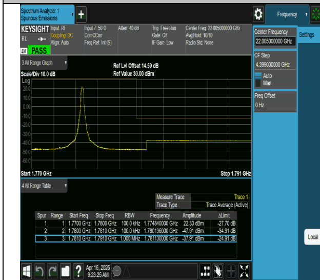
66-66-5MHz-5MHz-QPSK@QPSK-QPSK@QPSK-132599- 132647-1RB#24@0RB#0-0RB#0@0RB#0-PASS
