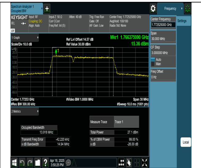
66-66-5MHz-10MHz-256QAM-256QAM-132550-132622-25RB#0-50RB#0-PASS
