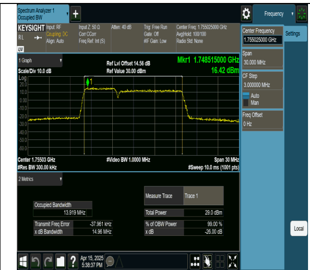
66-66-5MHz-10MHz-16QAM-16QAM-132375-132447-25RB#0-50RB#0-PASS
