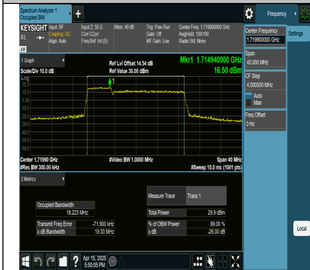
66-66-5MHz-15MHz-QPSK-QPSK-132002-132095-25RB#0-75RB#0-PASS
