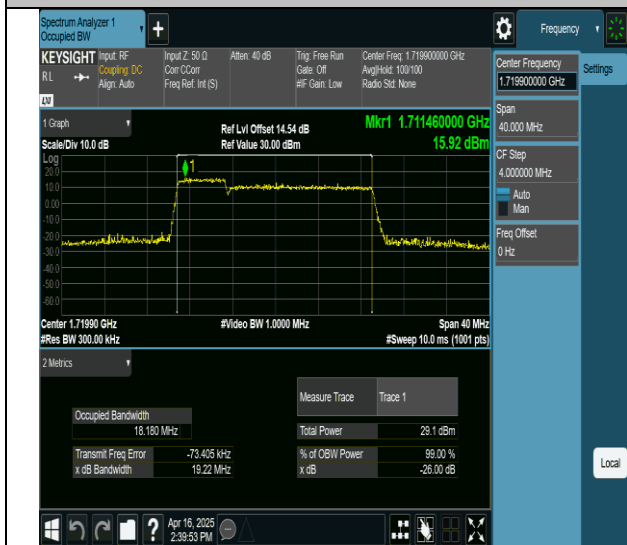
66-66-5MHz-15MHz-64QAM-64QAM-132002-132095-25RB#0-75RB#0-PASS
