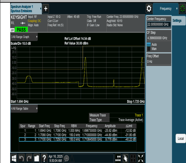
66-66-5MHz-10MHz-QPSK@QPSK-QPSK@QPSK-132000- 132072-1RB#0@0RB#0-1RB#49@0RB#0-PASS
