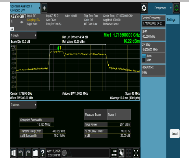
66-66-5MHz-15MHz-16QAM-16QAM-132002-132095-25RB#0-75RB#0-PASS
