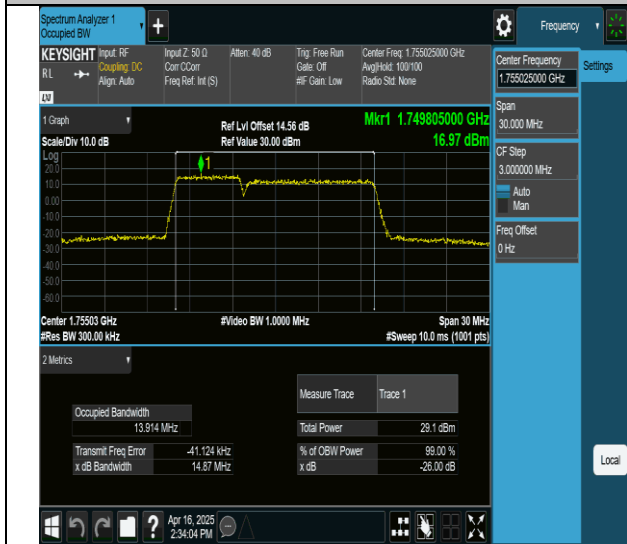
66-66-5MHz-10MHz-64QAM-64QAM-132375-132447-25RB#0-50RB#0-PASS
