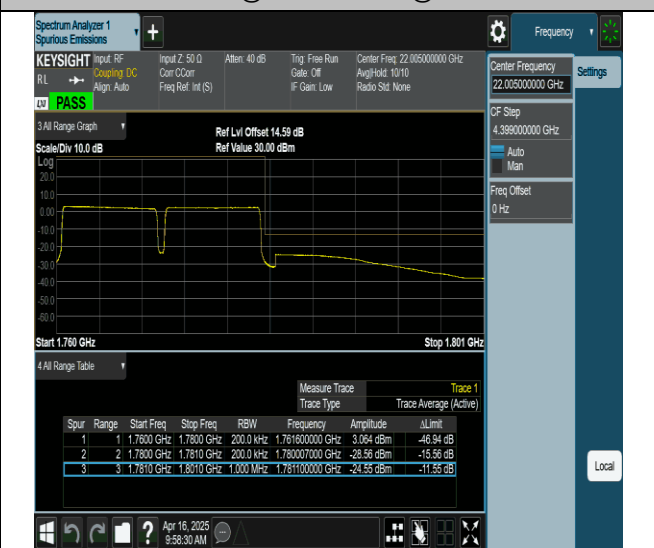
66-66-10MHz-10MHz-QPSK@QPSK-QPSK@QPSK-132523-132622-50RB#0@0RB#0-50RB#0@0RB#0-PASS
