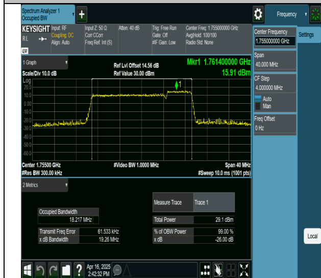
66-66-15MHz-5MHz-64QAM-64QAM-132398-132491-75RB#0-25RB#0-PASS
