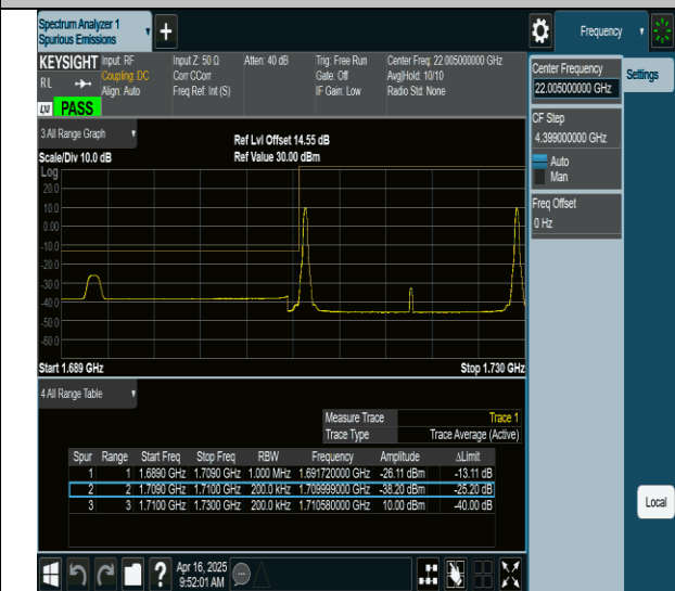
66-66-10MHz-10MHz-QPSK@QPSK-QPSK@QPSK-132022- 132121-1RB#0@0RB#0-1RB#49@0RB#0-PASS
