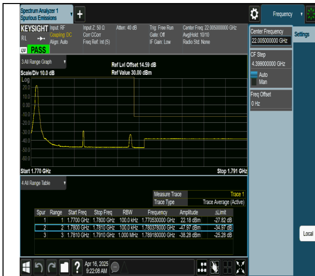
66-66-5MHz-5MHz-QPSK@QPSK-QPSK@QPSK-132599- 132647-1RB#0@0RB#0-0RB#0@0RB#0-PASS
