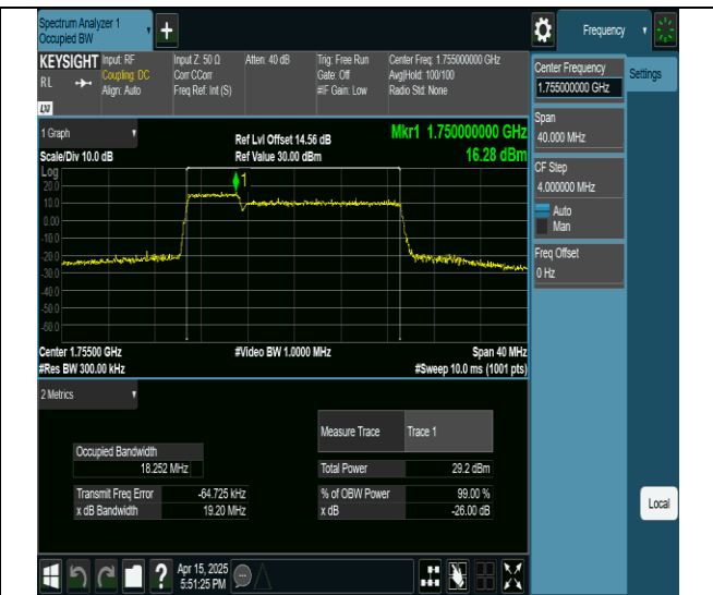
66-66-5MHz-15MHz-16QAM-16QAM-132353-132446-25RB#0- 75RB#0-PASS
