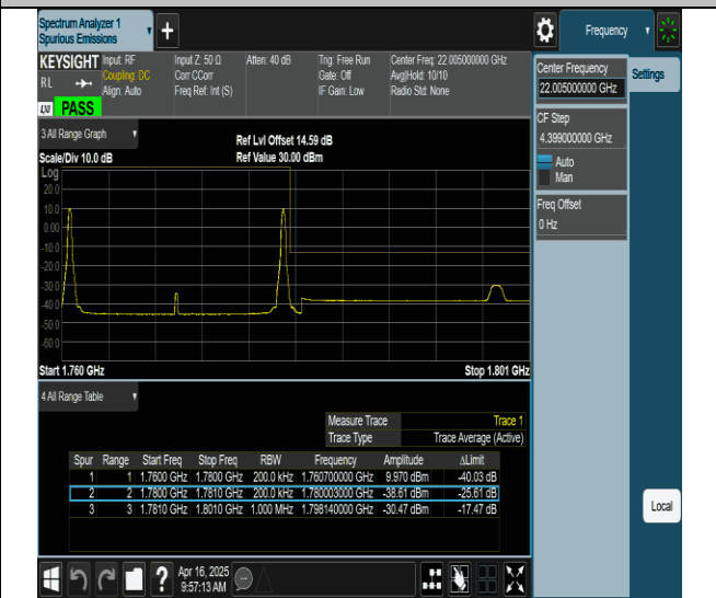
66-66-10MHz-10MHz-QPSK@QPSK-QPSK@QPSK-132523-132622-1RB#0@0RB#0-1RB#49@0RB#0-PASS
