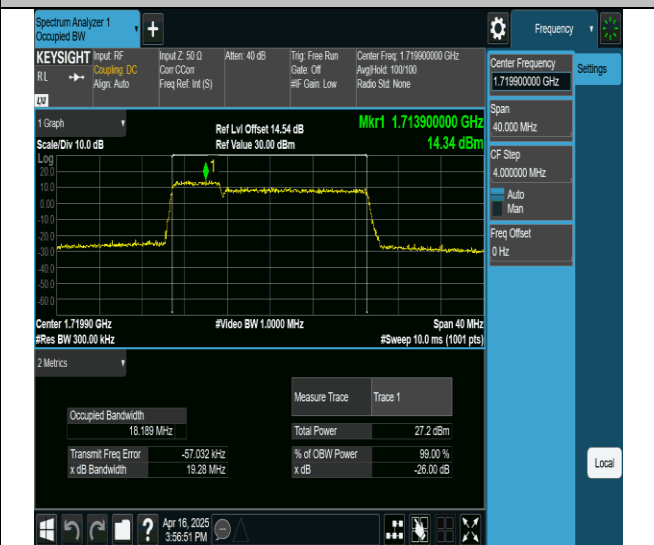
66-66-5MHz-15MHz-256QAM-256QAM-132002-132095-25RB#0-75RB#0-PASS
