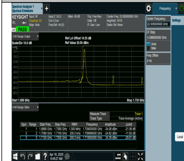
66-66-10MHz-10MHz-QPSK@QPSK-QPSK@QPSK-132022- 132121-1RB#0@0RB#0-0RB#0@0RB#0-PASS
