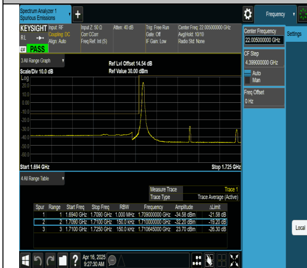
66-66-5MHz-10MHz-QPSK@QPSK-QPSK@QPSK-132000- 132072-1RB#0@0RB#0-0RB#0@0RB#0-PASS
