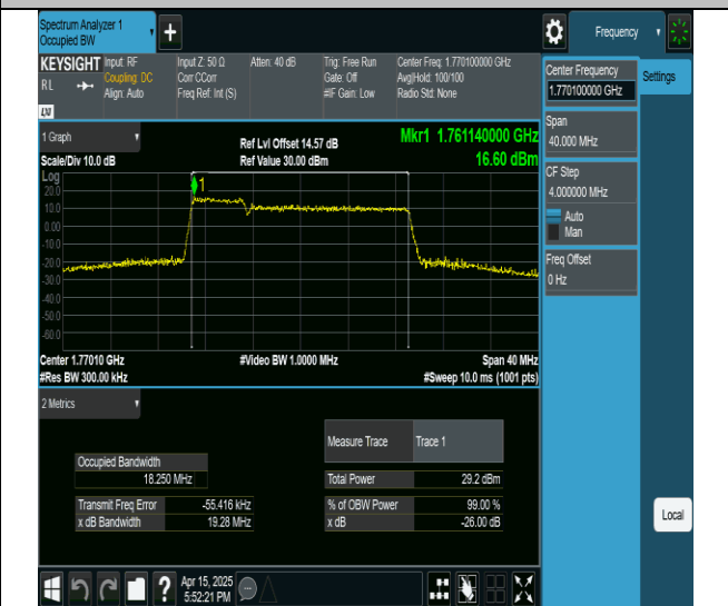
66-66-5MHz-15MHz-16QAM-16QAM-132504-132597-25RB#0- 75RB#0-PASS
