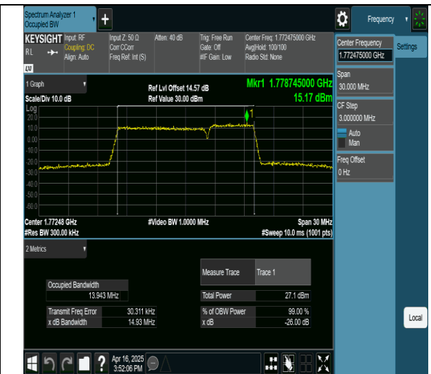
66-66-10MHz-5MHz-256QAM-256QAM-132572-132644-50RB#0-25RB#0-PASS
