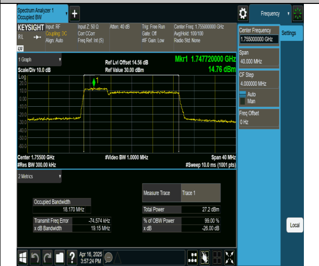
66-66-5MHz-15MHz-256QAM-256QAM-132353-132446-25RB#0- 75RB#0-PASS
