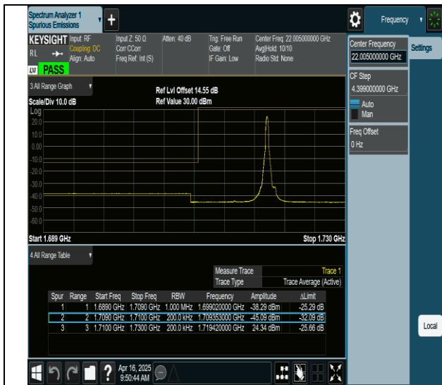
66-66-10MHz-10MHz-QPSK@QPSK-QPSK@QPSK-132022-132121-1RB#49@0RB#0-0RB#0@0RB#0-PASS
