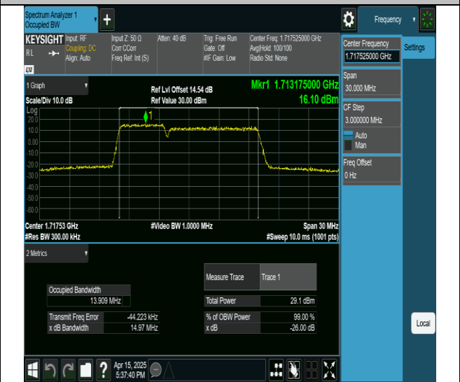
66-66-5MHz-10MHz-16QAM-16QAM-132000-132072-25RB#0-50RB#0-PASS
