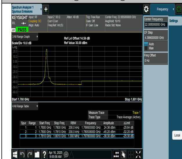
66-66-10MHz-10MHz-QPSK@QPSK-QPSK@QPSK-132523-132622-1RB#49@0RB#0-0RB#0@0RB#0-PASS
