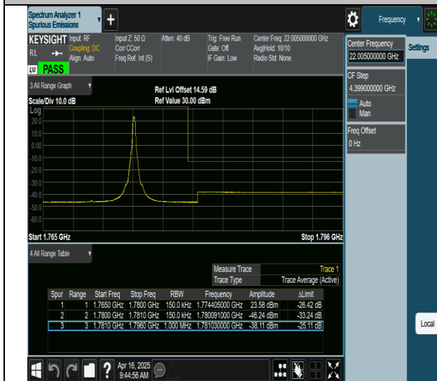
66-66-10MHz-5MHz-QPSK@QPSK-QPSK@QPSK-132572- 132644-1RB#49@0RB#0-0RB#0@0RB#0-PASS
