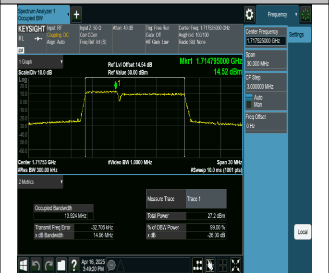
66-66-5MHz-10MHz-256QAM-256QAM-132000-132072-25RB#0-50RB#0-PASS
