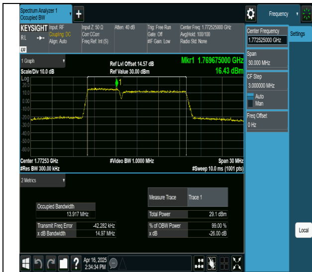
66-66-5MHz-10MHz-64QAM-64QAM-132550-132622-25RB#0-50RB#0-PASS
