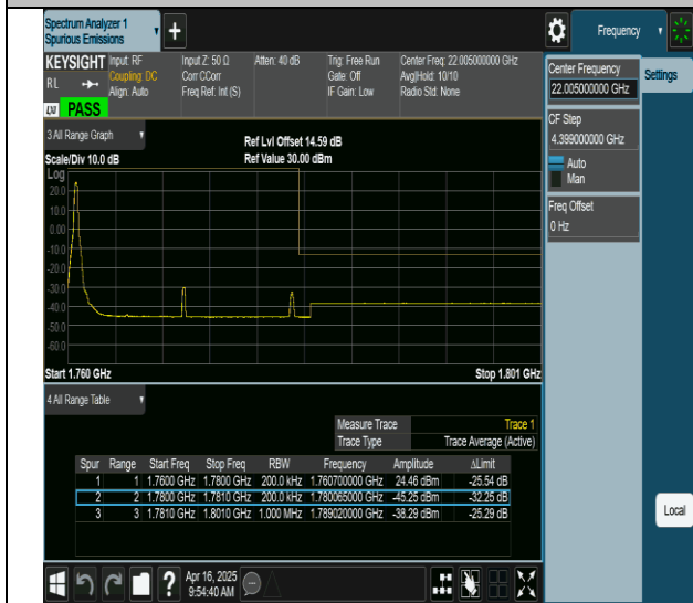
66-66-10MHz-10MHz-QPSK@QPSK-QPSK@QPSK-132523-132622-1RB#0@0RB#0-0RB#0@0RB#0-PASS
