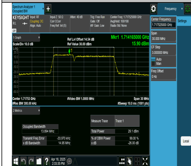
66-66-5MHz-10MHz-64QAM-64QAM-132000-132072-25RB#0-50RB#0-PASS
