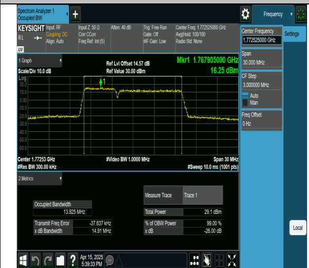
66-66-5MHz-10MHz-16QAM-16QAM-132550-132622-25RB#0-50RB#0-PASS
