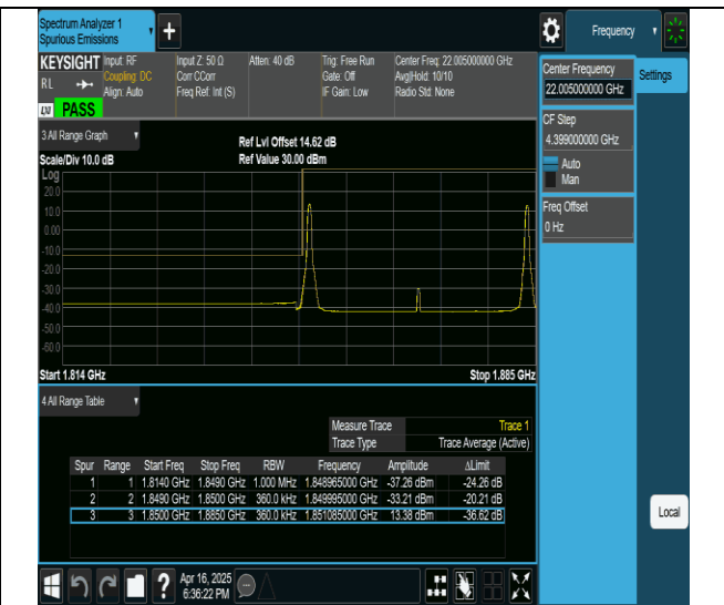
2-2-20MHz-15MHz-QPSK@QPSK-QPSK@QPSK-18700-18871- 1RB#0@0RB#0-1RB#74@0RB#0-PASS
