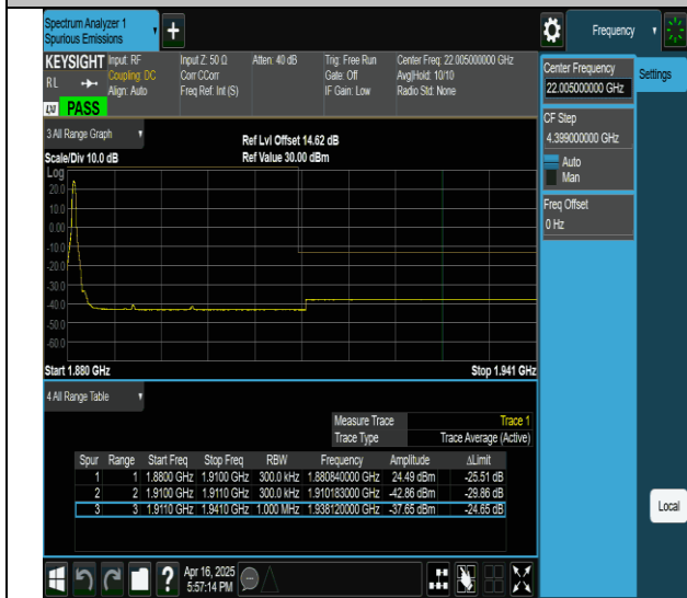
2-2-15MHz-15MHz-QPSK@QPSK-QPSK@QPSK-18975-19125- 1RB#0@0RB#0-0RB#0@0RB#0-PASS
