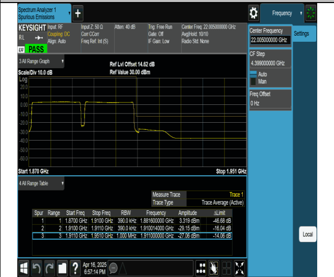
2-2-20MHz-20MHz-QPSK@QPSK-QPSK@QPSK-18902-19100-100RB#0@0RB#0-100RB#0@0RB#0-PASS
