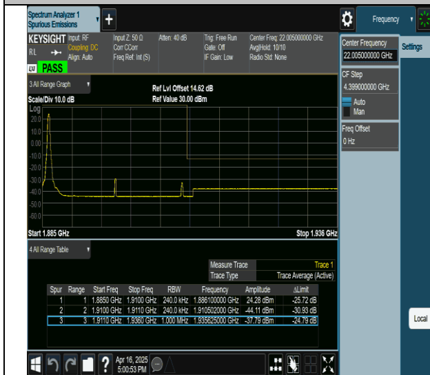
2-2-10MHz-15MHz-QPSK@QPSK-QPSK@QPSK-19005-19125- 1RB#0@0RB#0-0RB#0@0RB#0-PASS
