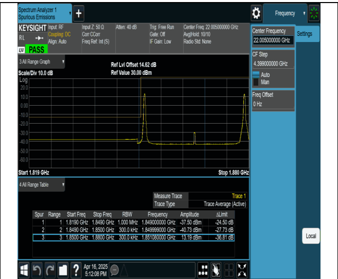
2-2-10MHz-20MHz-QPSK@QPSK-QPSK@QPSK-18655-18799- 1RB#0@0RB#0-1RB#99@0RB#0-PASS
