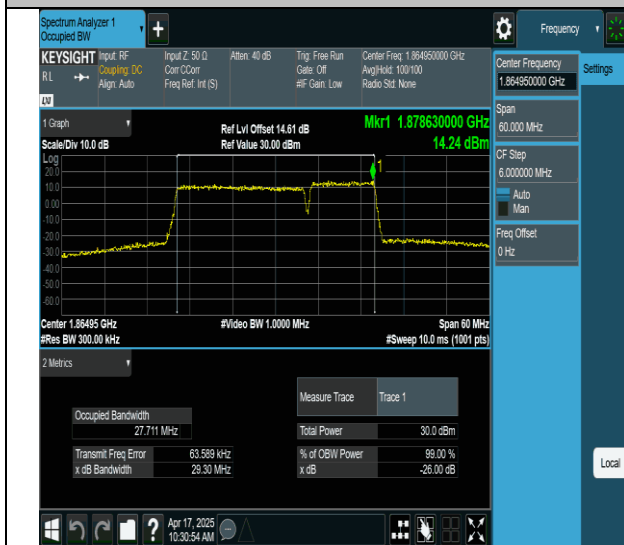
2-2-20MHz-10MHz-64QAM-64QAM-18700-18844-100RB#0- 50RB#0-PASS
