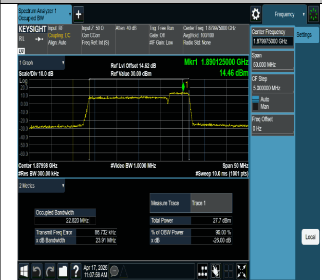
2-2-20MHz-5MHz-256QAM-256QAM-18875-18992-100RB#0- 25RB#0-PASS
