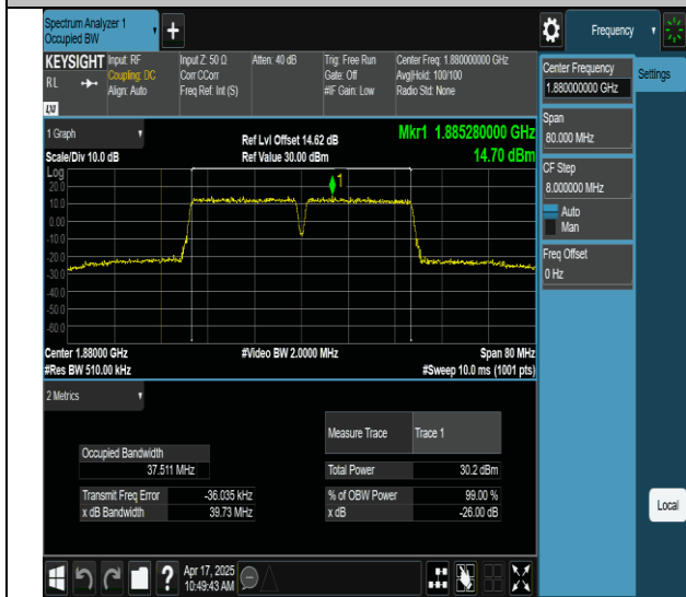
2-2-20MHz-20MHz-64QAM-64QAM-18801-18999-100RB#0-100RB#0-PASS
