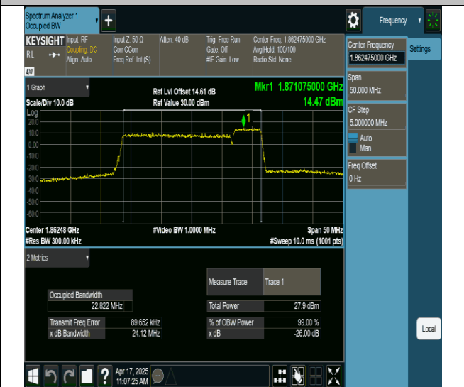
2-2-20MHz-5MHz-256QAM-256QAM-18700-18817-100RB#0-25RB#0-PASS
