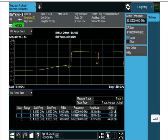
2-2-15MHz-15MHz-QPSK@QPSK-QPSK@QPSK-18675-18825- 75RB#0@0RB#0-0RB#0@0RB#0-PASS
