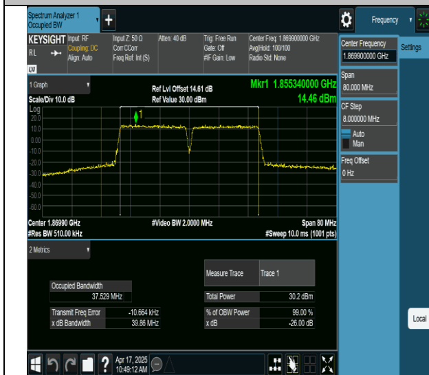
2-2-20MHz-20MHz-64QAM-64QAM-18700-18898-100RB#0-100RB#0-PASS
