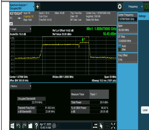
2-2-20MHz-5MHz-64QAM-64QAM-18875-18992-100RB#0- 25RB#0-PASS
