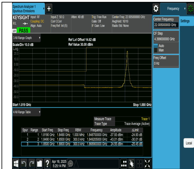
2-2-20MHz-10MHz-QPSK@QPSK-QPSK@QPSK-18700-18844- 1RB#99@0RB#0-0RB#0@0RB#0-PASS
