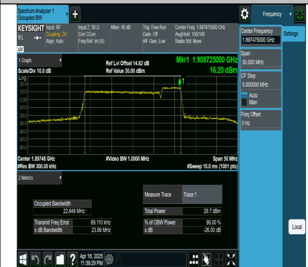
2-2-20MHz-5MHz-16QAM-16QAM-19050-19167-100RB#0- 25RB#0-PASS
