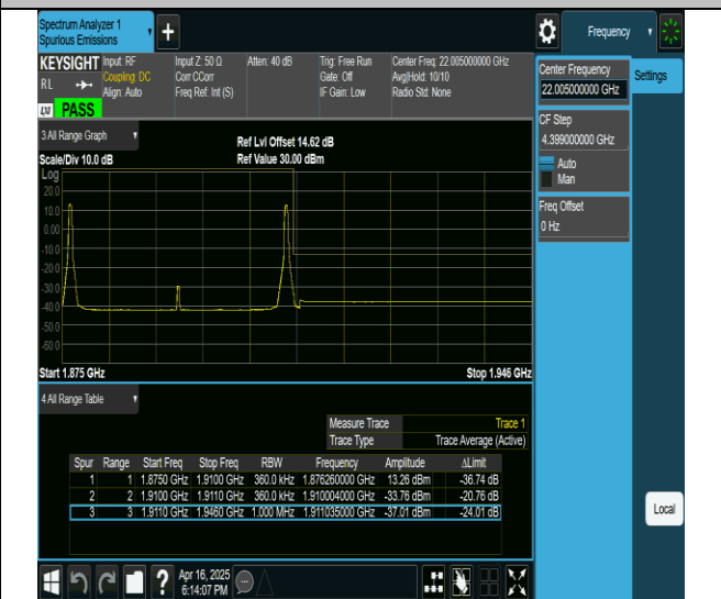
2-2-15MHz-20MHz-QPSK@QPSK-QPSK@QPSK-18929-19100-1RB#0@0RB#0-1RB#99@0RB#0-PASS
