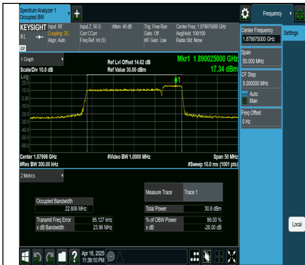
2-2-20MHz-5MHz-QPSK-QPSK-18875-18992-100RB#0-25RB#0- PASS
