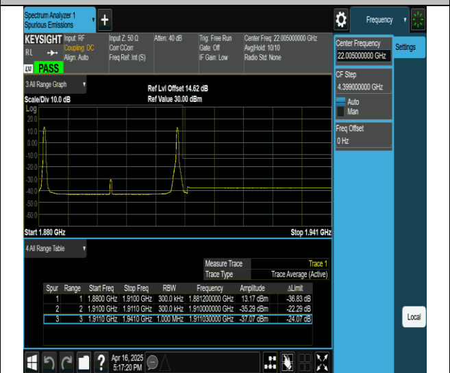
2-2-10MHz-20MHz-QPSK@QPSK-QPSK@QPSK-18956-19100- 1RB#0@0RB#0-1RB#99@0RB#0-PASS
