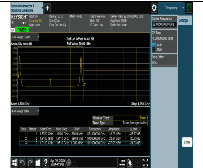
2-2-20MHz-20MHz-QPSK@QPSK-QPSK@QPSK-18902-19100-1RB#0@0RB#0-1RB#99@0RB#0-PASS
