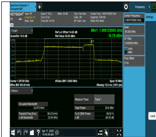
2-2-20MHz-5MHz-64QAM-64QAM-19050-19167-100RB#0- 25RB#0-PASS
