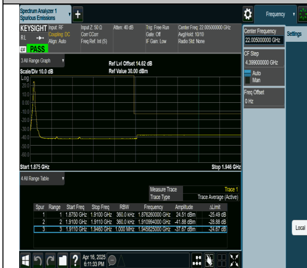
2-2-15MHz-20MHz-QPSK@QPSK-QPSK@QPSK-18929-19100-1RB#0@0RB#0-0RB#0@0RB#0-PASS
