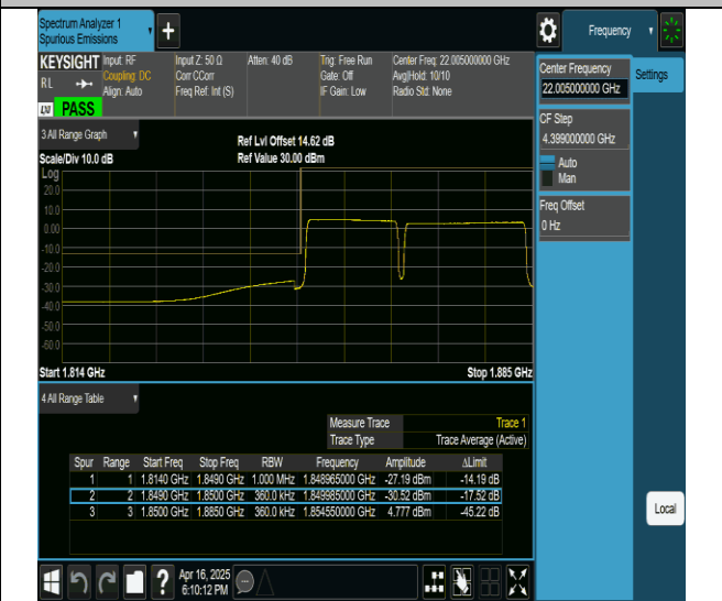
2-2-15MHz-20MHz-QPSK@QPSK-QPSK@QPSK-18678-18849-75RB#0@0RB#0-100RB#0@0RB#0-PASS
