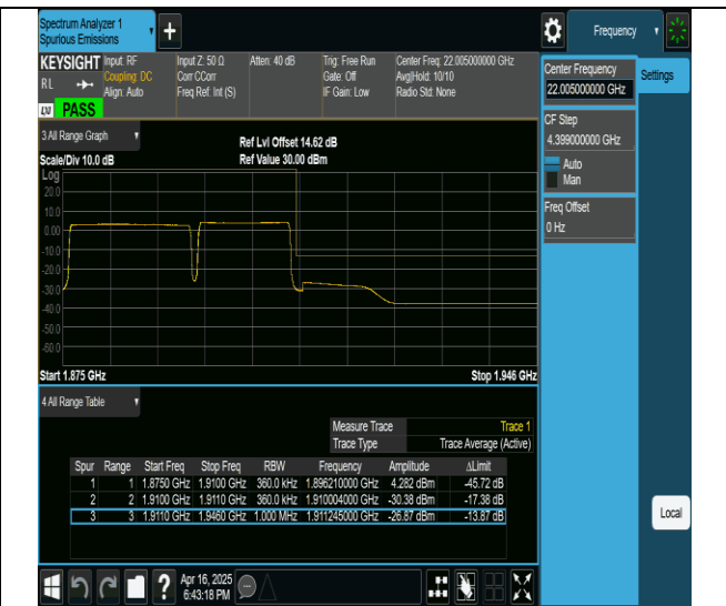
2-2-20MHz-15MHz-QPSK@QPSK-QPSK@QPSK-18951-19122-100RB#0@0RB#0-75RB#0@0RB#0-PASS
