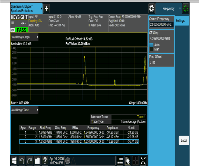
2-2-20MHz-20MHz-QPSK@QPSK-QPSK@QPSK-18700-18898-1RB#0@0RB#0-1RB#99@0RB#0-PASS
