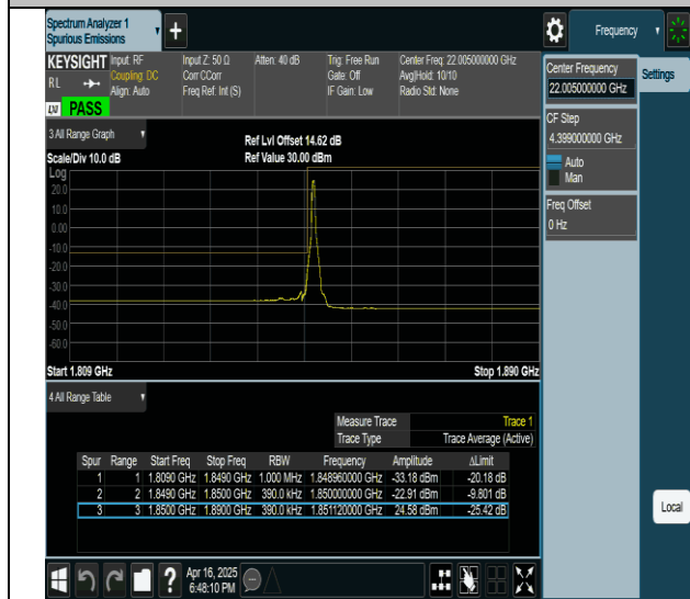
2-2-20MHz-20MHz-QPSK@QPSK-QPSK@QPSK-18700-18898-1RB#0@0RB#0-0RB#0@0RB#0-PASS
