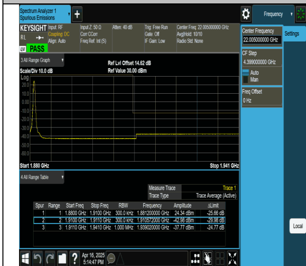
2-2-10MHz-20MHz-QPSK@QPSK-QPSK@QPSK-18956-19100- 1RB#0@0RB#0-0RB#0@0RB#0-PASS
