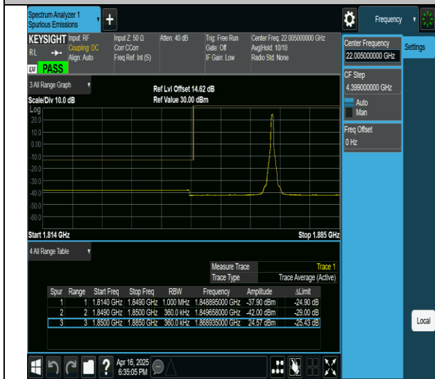
2-2-20MHz-15MHz-QPSK@QPSK-QPSK@QPSK-18700-18871- 1RB#99@0RB#0-0RB#0@0RB#0-PASS
