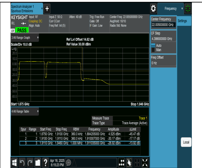
2-2-15MHz-20MHz-QPSK@QPSK-QPSK-18929-19100-75RB#0@0RB#0-100RB#0@0RB#0-PASS
