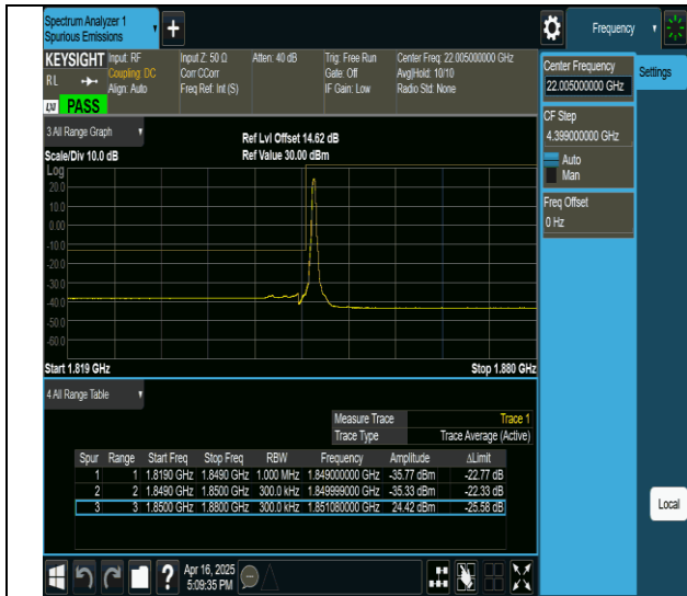
2-2-10MHz-20MHz-QPSK@QPSK-QPSK@QPSK-18655-18799- 1RB#0@0RB#0-0RB#0@0RB#0-PASS
