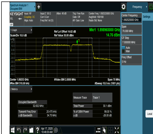
2-2-20MHz-15MHz-64QAM-64QAM-18951-19122-100RB#0-75RB#0-PASS
