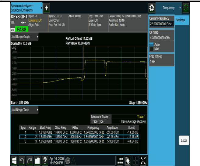
2-2-10MHz-20MHz-QPSK@QPSK-QPSK@QPSK-18655-18799- 50RB#0@0RB#0-100RB#0@0RB#0-PASS
