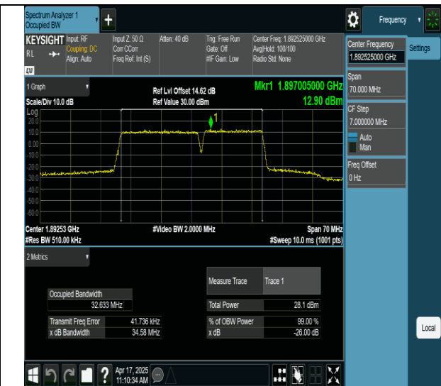
2-2-20MHz-15MHz-256QAM-256QAM-18951-19122-100RB#0-75RB#0-PASS
