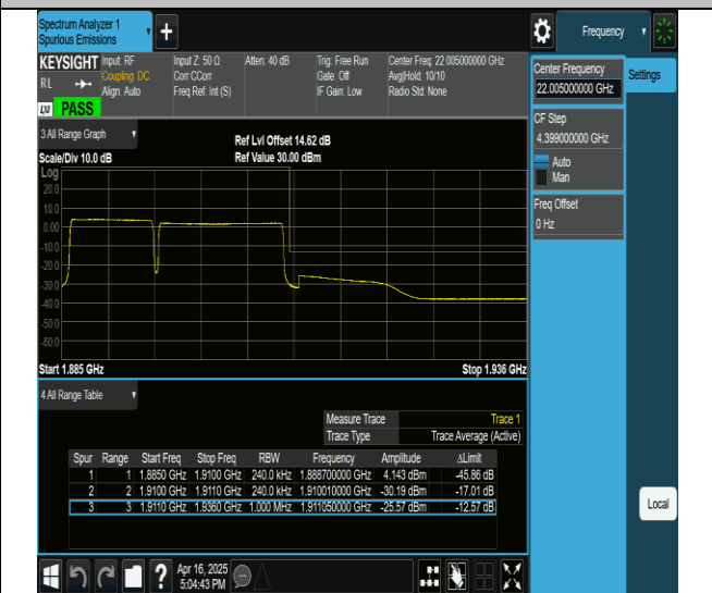
2-2-10MHz-15MHz-QPSK@QPSK-QPSK@QPSK-19005-19125- 50RB#0@0RB#0-75RB#0@0RB#0-PASS
