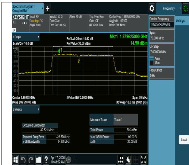
2-2-15MHz-20MHz-64QAM-64QAM-18929-19100-75RB#0-100RB#0-PASS
