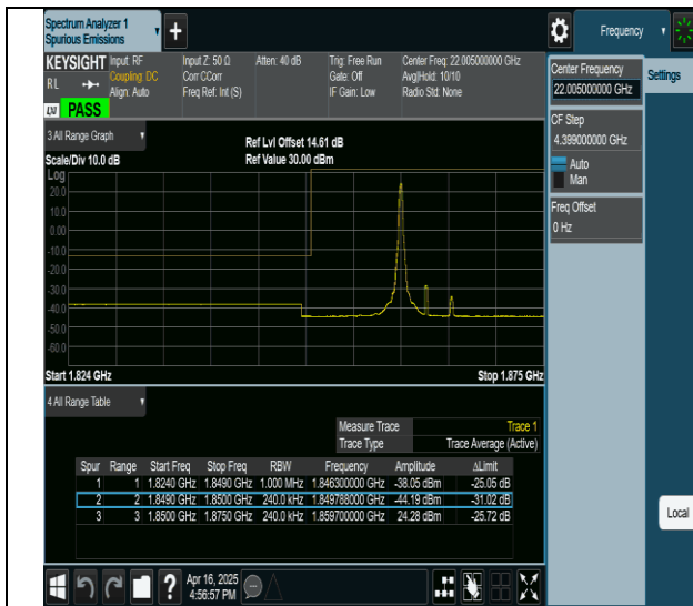
2-2-10MHz-15MHz-QPSK@QPSK-QPSK@QPSK-18653-18773- 1RB#49@0RB#0-0RB#0@0RB#0-PASS
