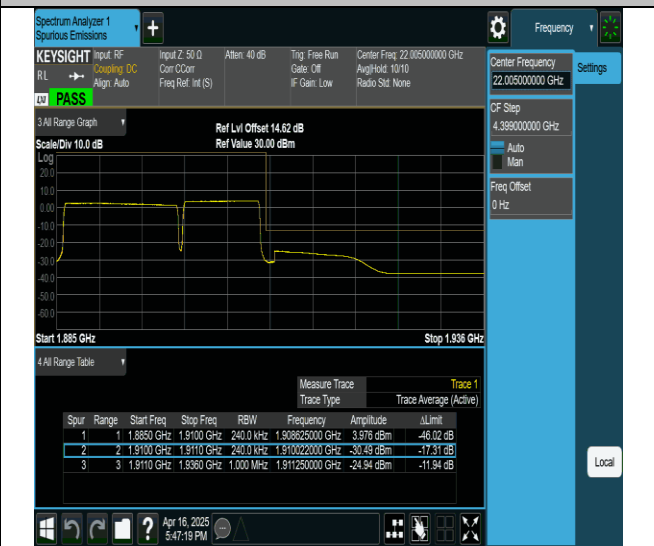
2-2-15MHz-10MHz-QPSK@QPSK-QPSK-19027-19147-75RB#0@0RB#0-50RB#0@0RB#0-PASS
