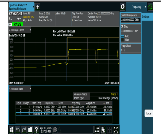
2-2-20MHz-15MHz-QPSK@QPSK-QPSK@QPSK-18700-18871- 100RB#0@0RB#0-75RB#0@0RB#0-PASS
