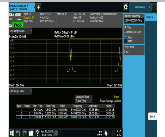
2-2-10MHz-15MHz-QPSK@QPSK-QPSK@QPSK-18653-18773- 1RB#0@0RB#0-1RB#74@0RB#0-PASS
