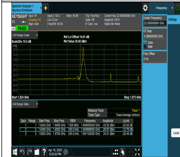
2-2-20MHz-5MHz-QPSK@QPSK-QPSK-18700-18817-1RB#0@0RB#0-0RB#0@0RB#0-PASS
