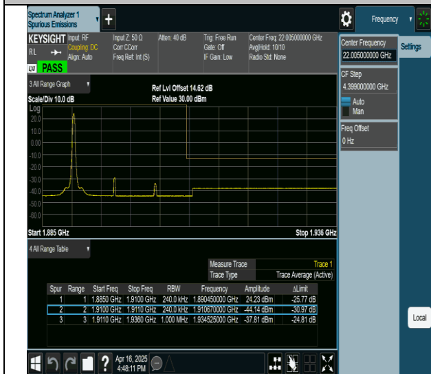
2-2-5MHz-20MHz-QPSK@QPSK-QPSK@QPSK-18983-19100- 1RB#24@0RB#0-0RB#0@0RB#0-PASS
