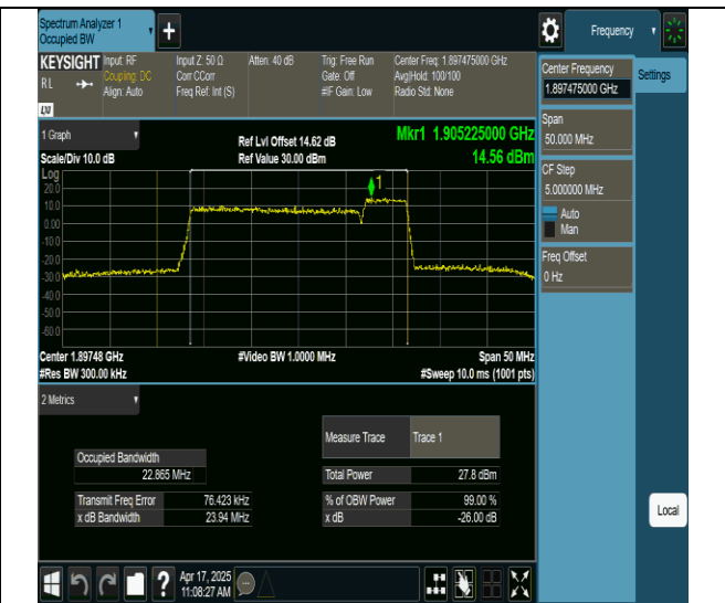
2-2-20MHz-5MHz-256QAM-256QAM-19050-19167-100RB#0- 25RB#0-PASS
