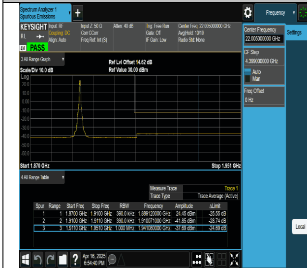
2-2-20MHz-20MHz-QPSK@QPSK-QPSK@QPSK-18902-19100-1RB#99@0RB#0-0RB#0@0RB#0-PASS
