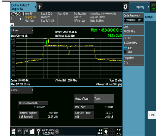
2-2-15MHz-15MHz-QPSK-QPSK-18675-18825-75RB#0-75RB#0-PASS
