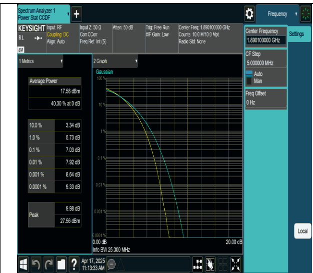
2-2-20MHz-20MHz-256QAM-256QAM-18902-19100-100RB#0- 100RB#0-PASS
