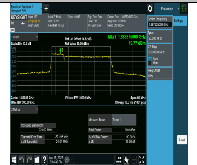
2-2-5MHz-20MHz-16QAM-16QAM-18983-19100-25RB#0- 100RB#0-PASS
