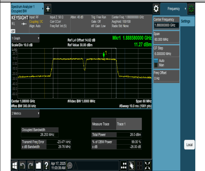
2-2-15MHz-15MHz-256QAM-256QAM-18825-18975-75RB#0- 75RB#0-PASS
