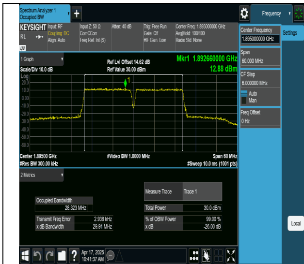
2-2-15MHz-15MHz-64QAM-64QAM-18975-19125-75RB#0-75RB#0-PASS
