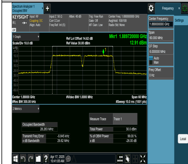
2-2-15MHz-15MHz-64QAM-64QAM-18825-18975-75RB#0- 75RB#0-PASS
