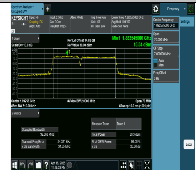
2-2-15MHz-20MHz-16QAM-16QAM-18929-19100-75RB#0- 100RB#0-PASS
