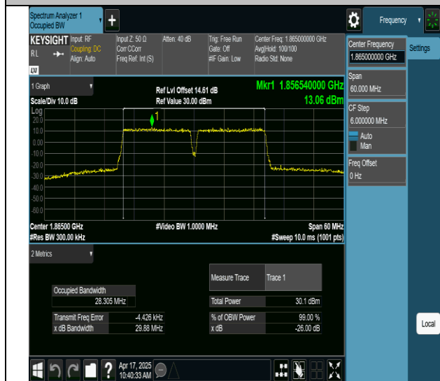
2-2-15MHz-15MHz-64QAM-64QAM-18675-18825-75RB#0-75RB#0-PASS
