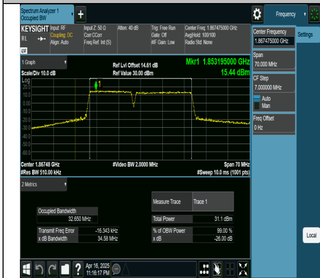
2-2-15MHz-20MHz-QPSK-QPSK-18678-18849-75RB#0-100RB#0-PASS
