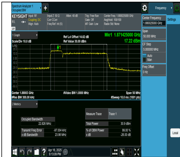
2-2-5MHz-20MHz-QPSK-QPSK-18808-18925-25RB#0-100RB#0- PASS
