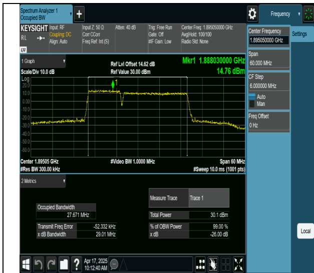
2-2-10MHz-20MHz-64QAM-64QAM-18956-19100-50RB#0-100RB#0-PASS
