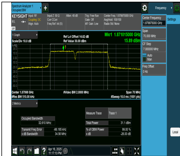
2-2-15MHz-20MHz-QPSK-QPSK-18803-18974-75RB#0- 100RB#0-PASS
