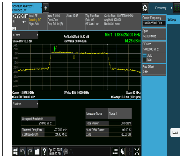
2-2-10MHz-15MHz-64QAM-64QAM-19005-19125-50RB#0-75RB#0-PASS
