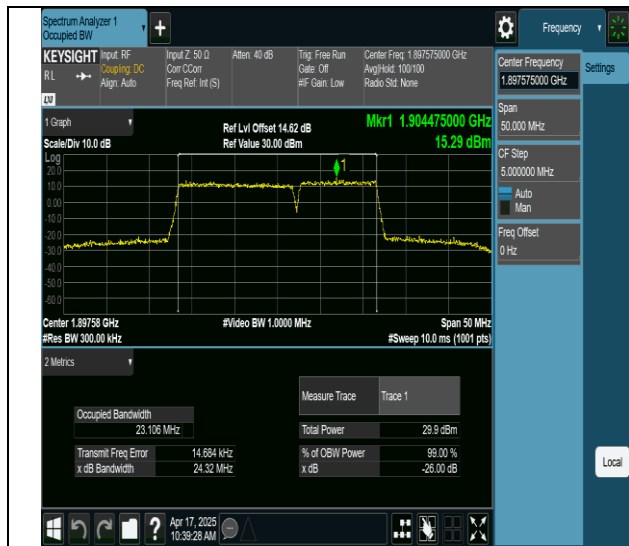
2-2-15MHz-10MHz-64QAM-64QAM-19027-19147-75RB#0-50RB#0-PASS
