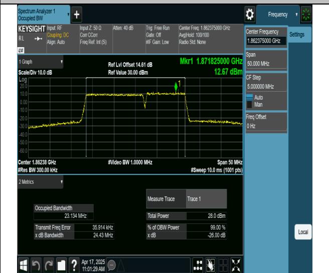
2-2-15MHz-10MHz-256QAM-256QAM-18675-18795-75RB#0-50RB#0-PASS
