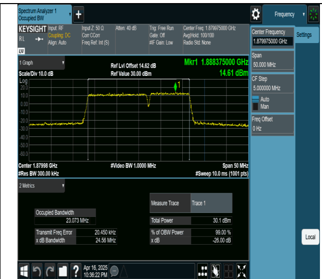
2-2-15MHz-10MHz-16QAM-16QAM-18851-18971-75RB#0-50RB#0-PASS
