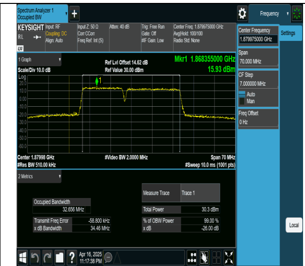
2-2-15MHz-20MHz-16QAM-16QAM-18803-18974-75RB#0- 100RB#0-PASS
