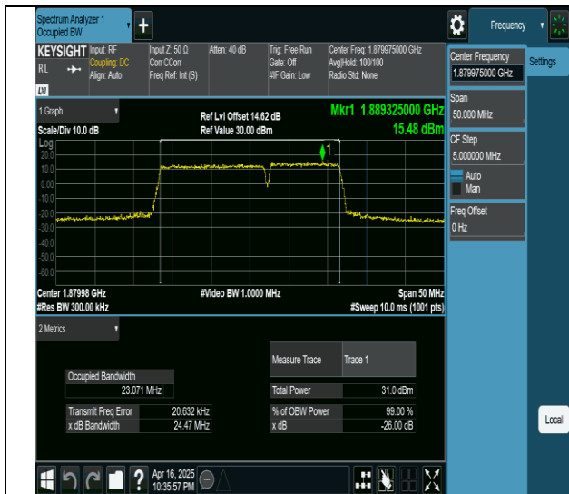
2-2-15MHz-10MHz-QPSK-QPSK-18851-18971-75RB#0-50RB#0-PASS
