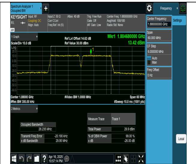
2-2-15MHz-15MHz-16QAM-16QAM-18825-18975-75RB#0- 75RB#0-PASS
