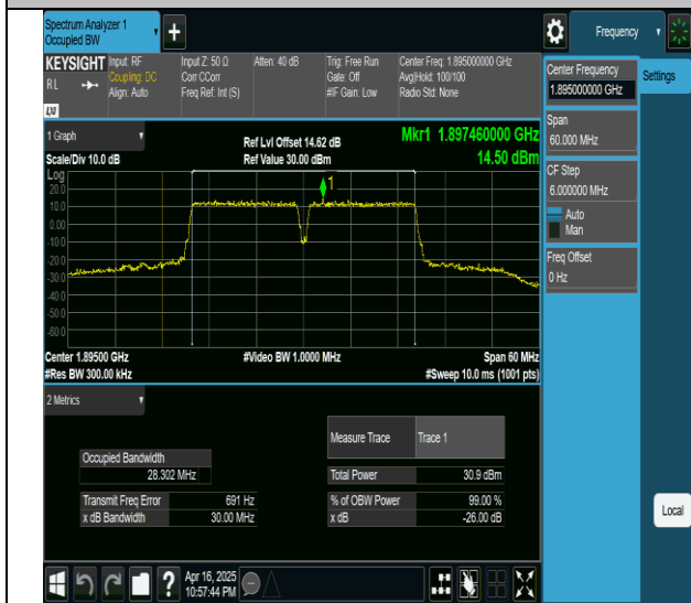
2-2-15MHz-15MHz-QPSK-QPSK-18975-19125-75RB#0-75RB#0- PASS
