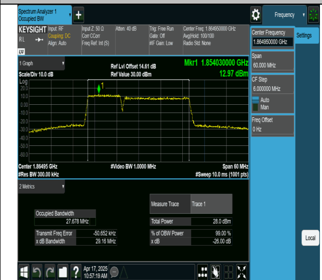
2-2-10MHz-20MHz-256QAM-256QAM-18655-18799-50RB#0-100RB#0-PASS
