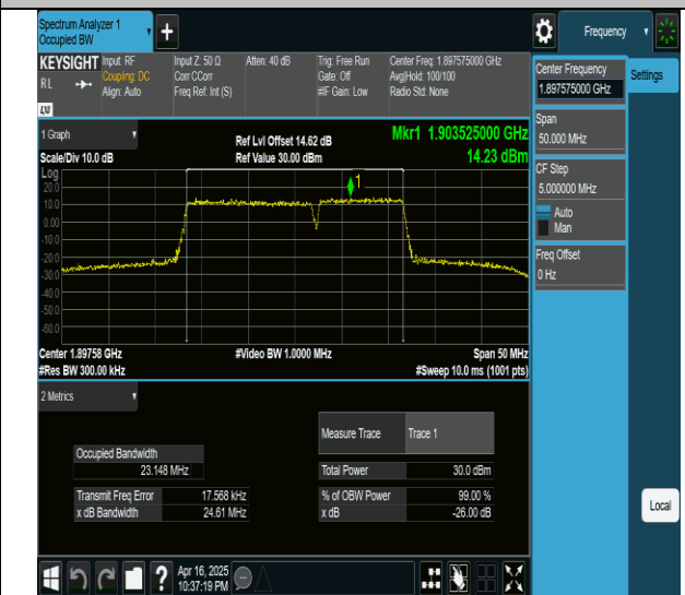
2-2-15MHz-10MHz-16QAM-16QAM-19027-19147-75RB#0-50RB#0-PASS
