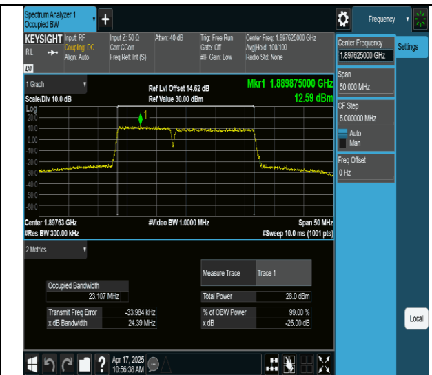
2-2-10MHz-15MHz-256QAM-256QAM-19005-19125-50RB#0-75RB#0-PASS
