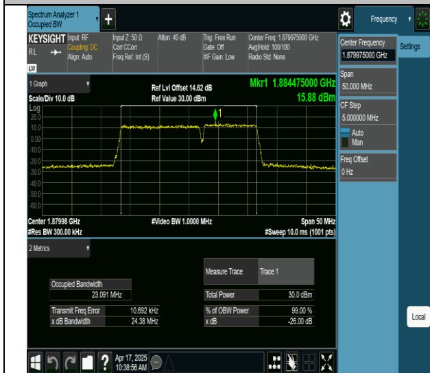
2-2-15MHz-10MHz-64QAM-64QAM-18851-18971-75RB#0-50RB#0-PASS
