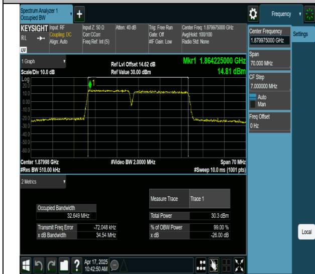
2-2-15MHz-20MHz-64QAM-64QAM-18803-18974-75RB#0- 100RB#0-PASS
