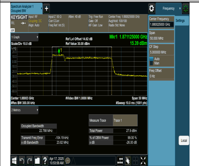
2-2-5MHz-20MHz-256QAM-256QAM-18808-18925-25RB#0- 100RB#0-PASS
