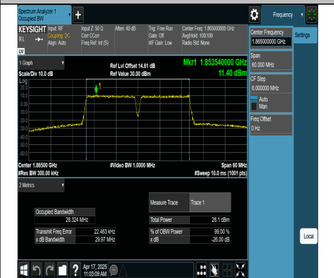
2-2-15MHz-15MHz-256QAM-256QAM-18675-18825-75RB#0-75RB#0-PASS
