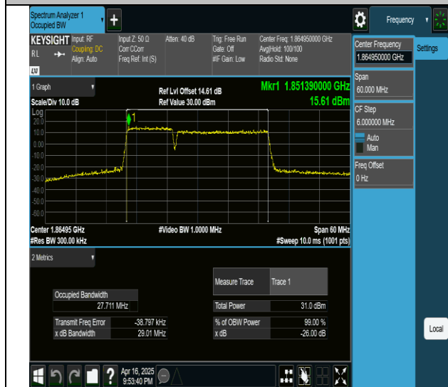
2-2-10MHz-20MHz-QPSK-QPSK-18655-18799-50RB#0-100RB#0-PASS
