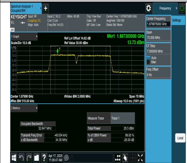
2-2-15MHz-20MHz-256QAM-256QAM-18803-18974-75RB#0- 100RB#0-PASS
