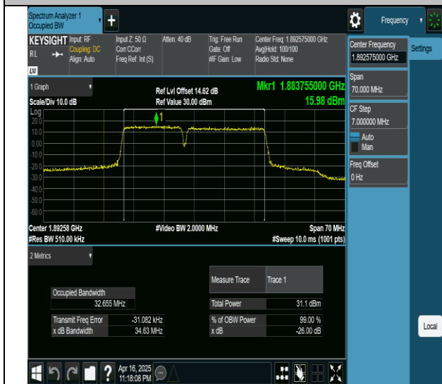
2-2-15MHz-20MHz-QPSK-QPSK-18929-19100-75RB#0- 100RB#0-PASS
