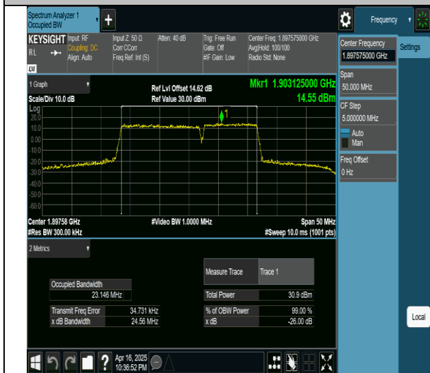
2-2-15MHz-10MHz-QPSK-QPSK-19027-19147-75RB#0-50RB#0-PASS
