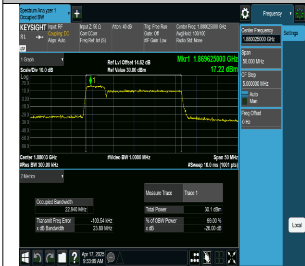
2-2-5MHz-20MHz-64QAM-64QAM-18808-18925-25RB#0- 100RB#0-PASS
