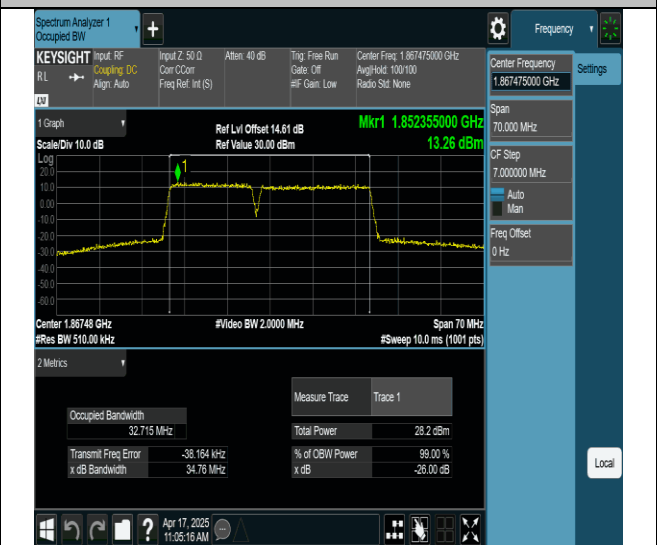
2-2-15MHz-20MHz-256QAM-256QAM-18678-18849-75RB#0-100RB#0-PASS
