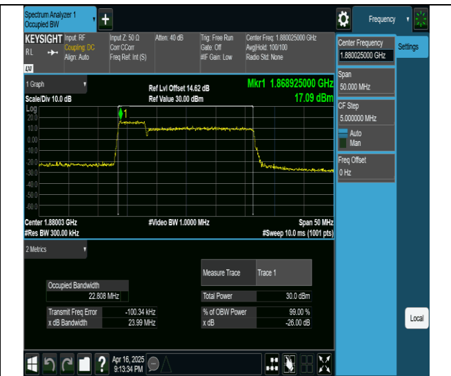
2-2-5MHz-20MHz-16QAM-16QAM-18808-18925-25RB#0- 100RB#0-PASS
