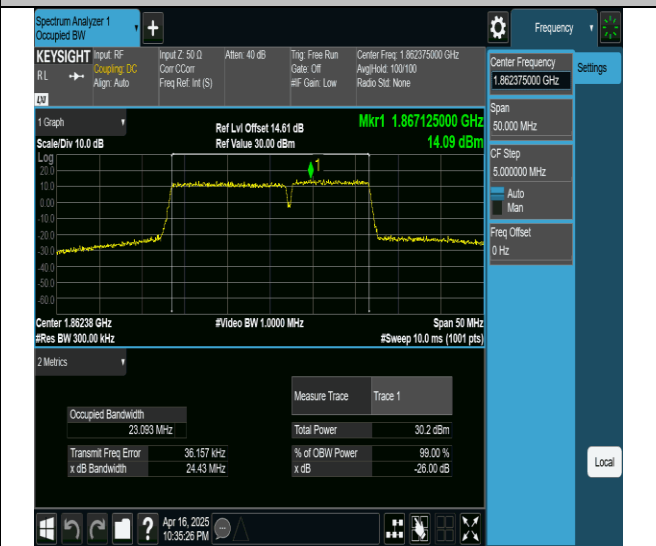
2-2-15MHz-10MHz-16QAM-16QAM-18675-18795-75RB#0-50RB#0-PASS
