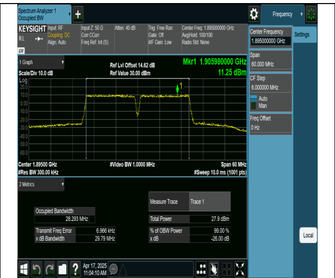
2-2-15MHz-15MHz-256QAM-256QAM-18975-19125-75RB#0-75RB#0-PASS
