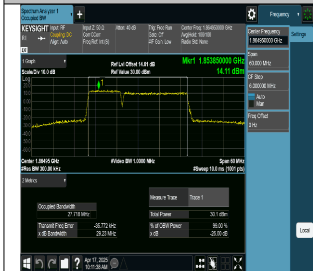
2-2-10MHz-20MHz-64QAM-64QAM-18655-18799-50RB#0-100RB#0-PASS
