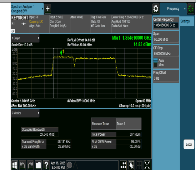
2-2-10MHz-20MHz-16QAM-16QAM-18655-18799-50RB#0-100RB#0-PASS
