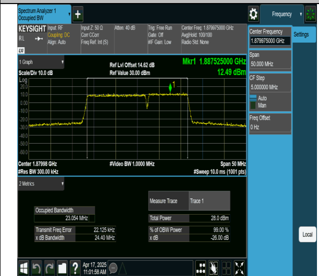
2-2-15MHz-10MHz-256QAM-256QAM-18851-18971-75RB#0-50RB#0-PASS
