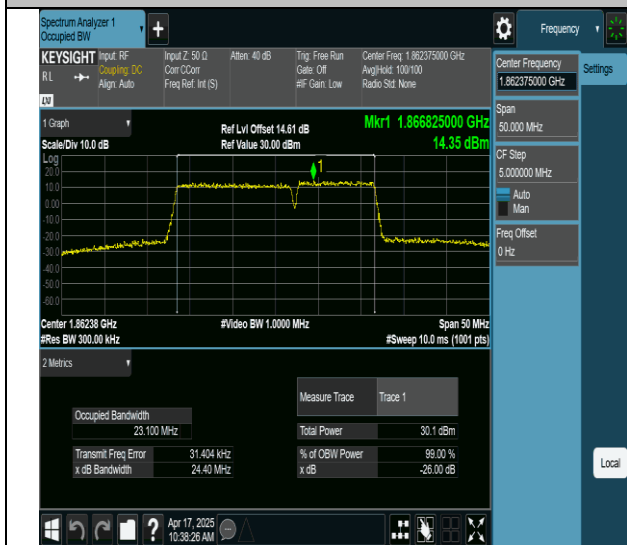
2-2-15MHz-10MHz-64QAM-64QAM-18675-18795-75RB#0-50RB#0-PASS
