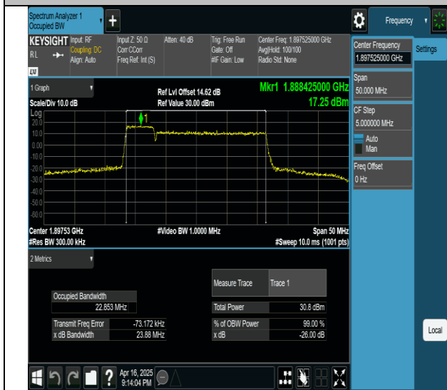
2-2-5MHz-20MHz-QPSK-QPSK-18983-19100-25RB#0-100RB#0- PASS
