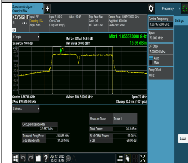
2-2-15MHz-20MHz-64QAM-64QAM-18678-18849-75RB#0-100RB#0-PASS
