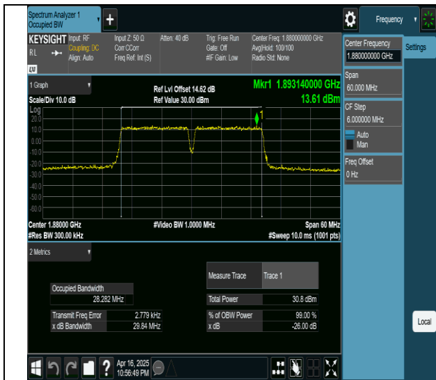
2-2-15MHz-15MHz-QPSK-QPSK-18825-18975-75RB#0-75RB#0- PASS
