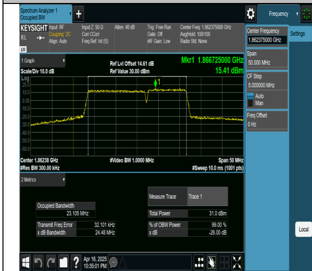
2-2-15MHz-10MHz-QPSK-QPSK-18675-18795-75RB#0-50RB#0-PASS
