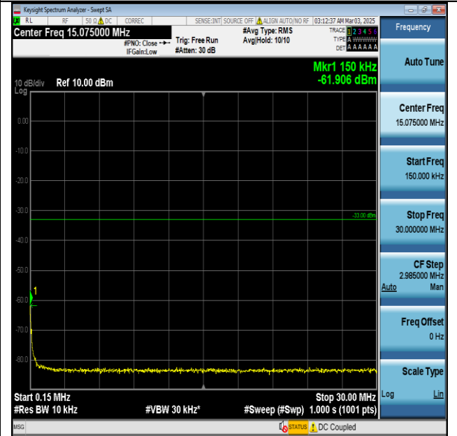
Band66-20MHz-QPSK-132572-1RB#0-0.15~30-PASS
