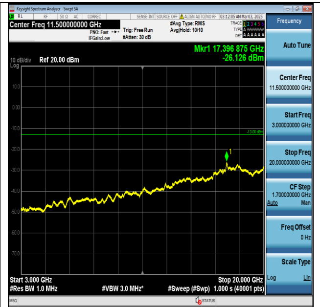
Band66-20MHz-QPSK-132322-1RB#0-3000~20000-PASS
