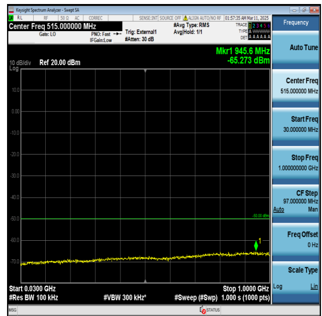
Band48-20MHz-QPSK-55990-1RB#0-30~1000-PASS
