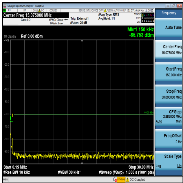
Band48-20MHz-QPSK-55990-1RB#0-0.15~30-PASS
