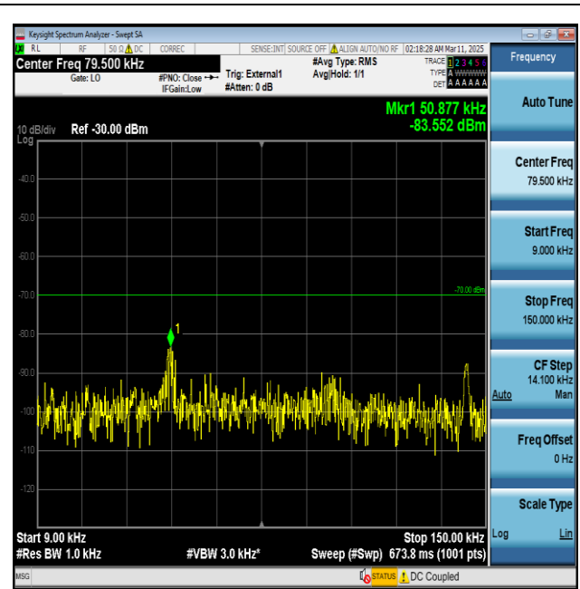
Band48-20MHz-QPSK-55990-1RB#0-0.009~0.15-PASS
