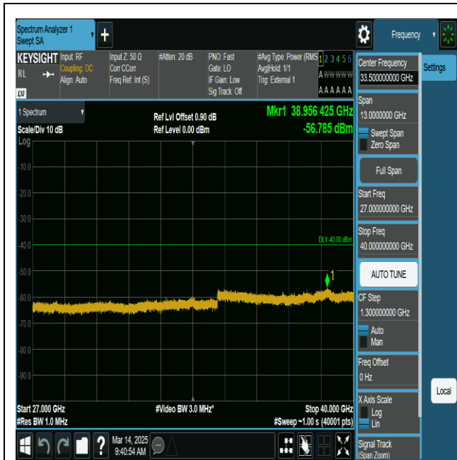
Band48-20MHz-QPSK-55340-1RB#0-27000~40000-PASS
