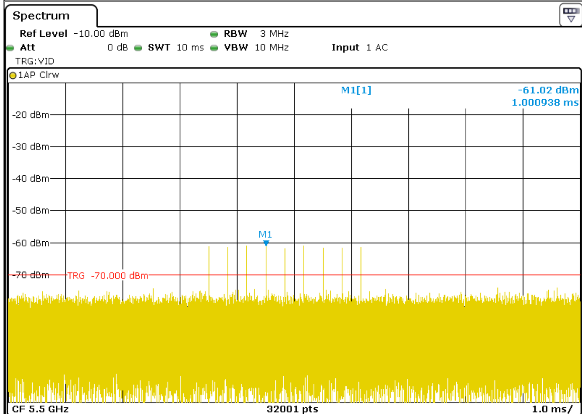
Radar Signal 6
