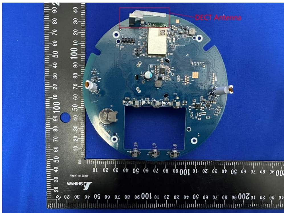
(18) EUT Photo – SSSX5R0-29
