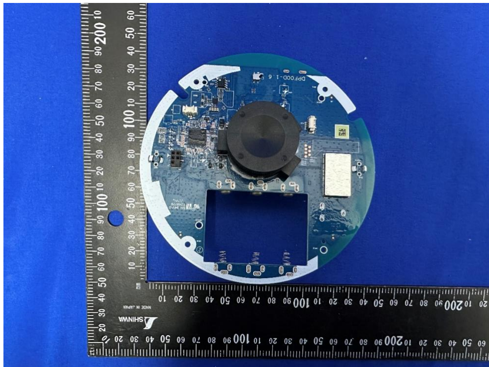
(17) EUT Photo – SSSX5R0-29
