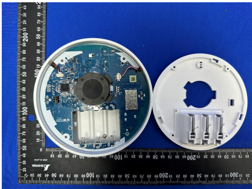
(14) EUT Photo – SSSX5R0-29
