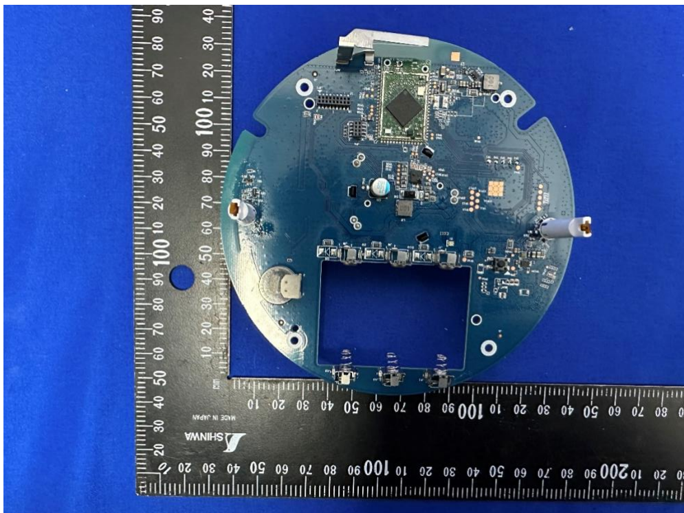
(20) EUT Photo – SSSX5R0-29
