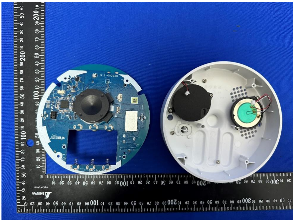
(16) EUT Photo – SSSX5R0-29
