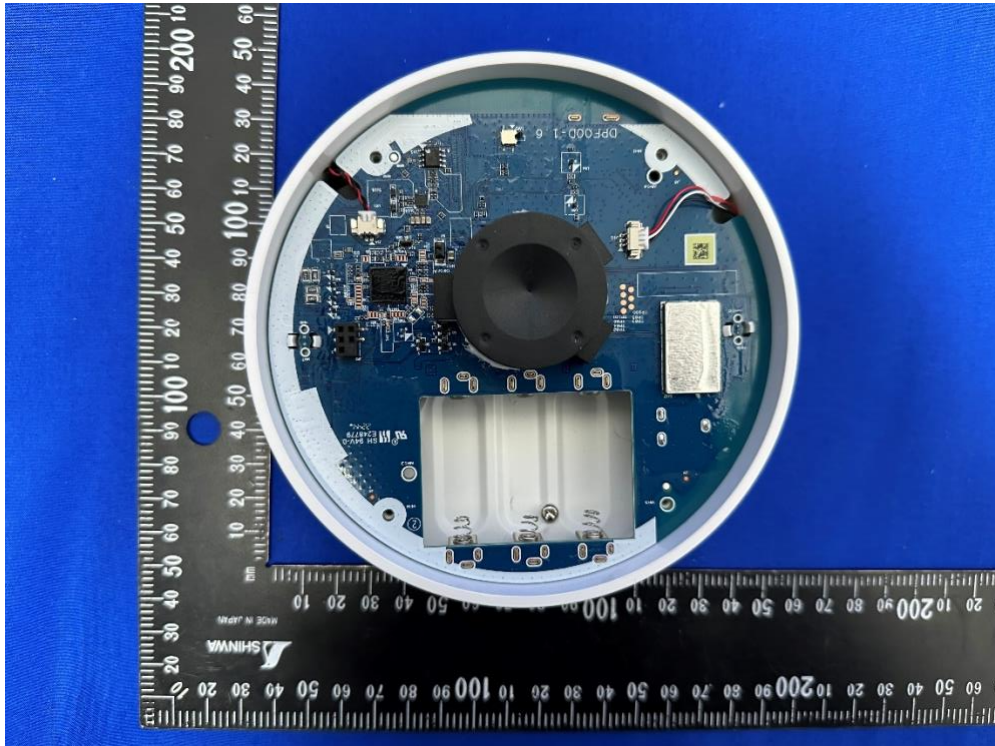
(15) EUT Photo – SSSX5R0-29
