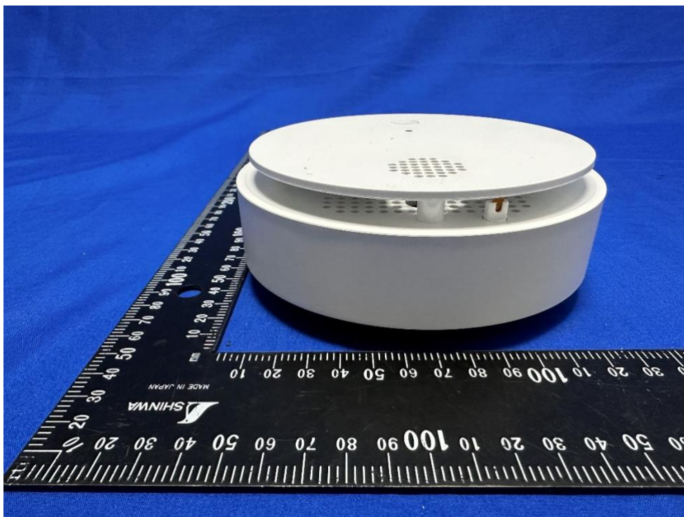
(7) EUT Photo – SSSX5R0-29
