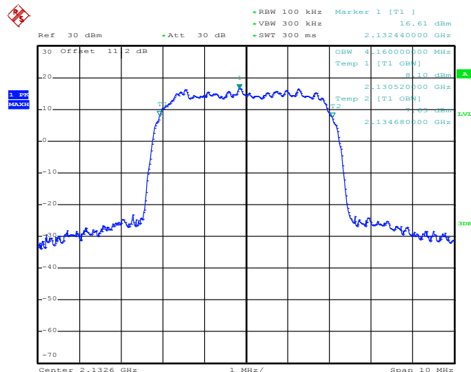
99% Occupied Bandwidth Plot on Channel 1638
