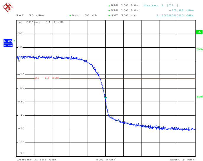
Higher Band Edge Plot on Channel 1738
