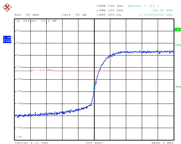
Lower Band Edge Plot on Channel 1537
