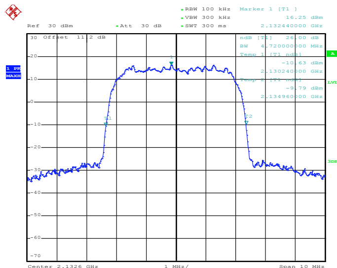
26dB Bandwidth Plot on Channel 1638
