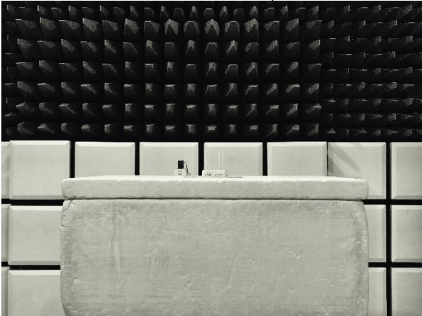
FR1_Radiated_Setup
