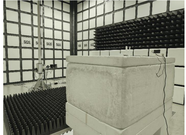
FR1_Radiated_Setup
