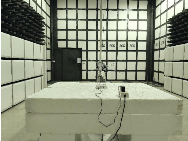
FCC_96.47_NR_CBSD_Setup
