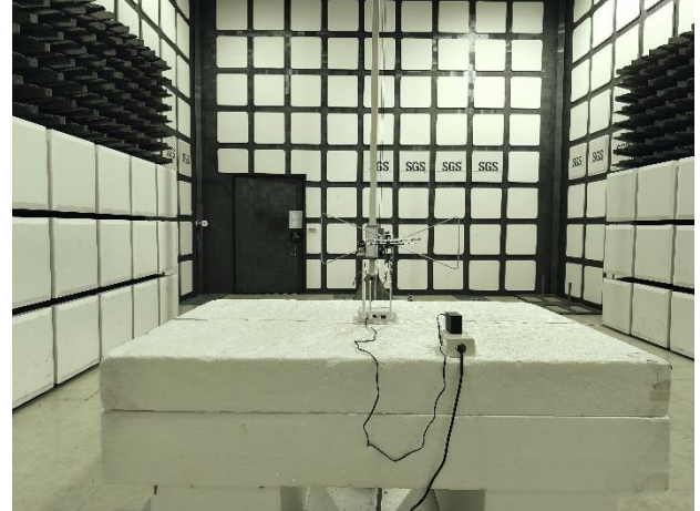
LTE_Radiated_Setup
