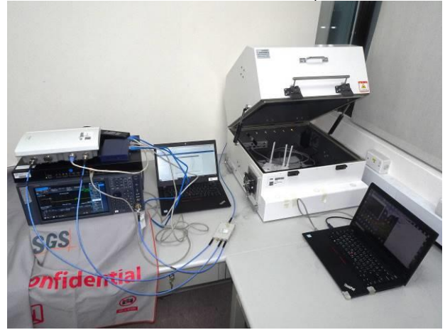
FCC_96.47_LTE_CBSD_Setup
