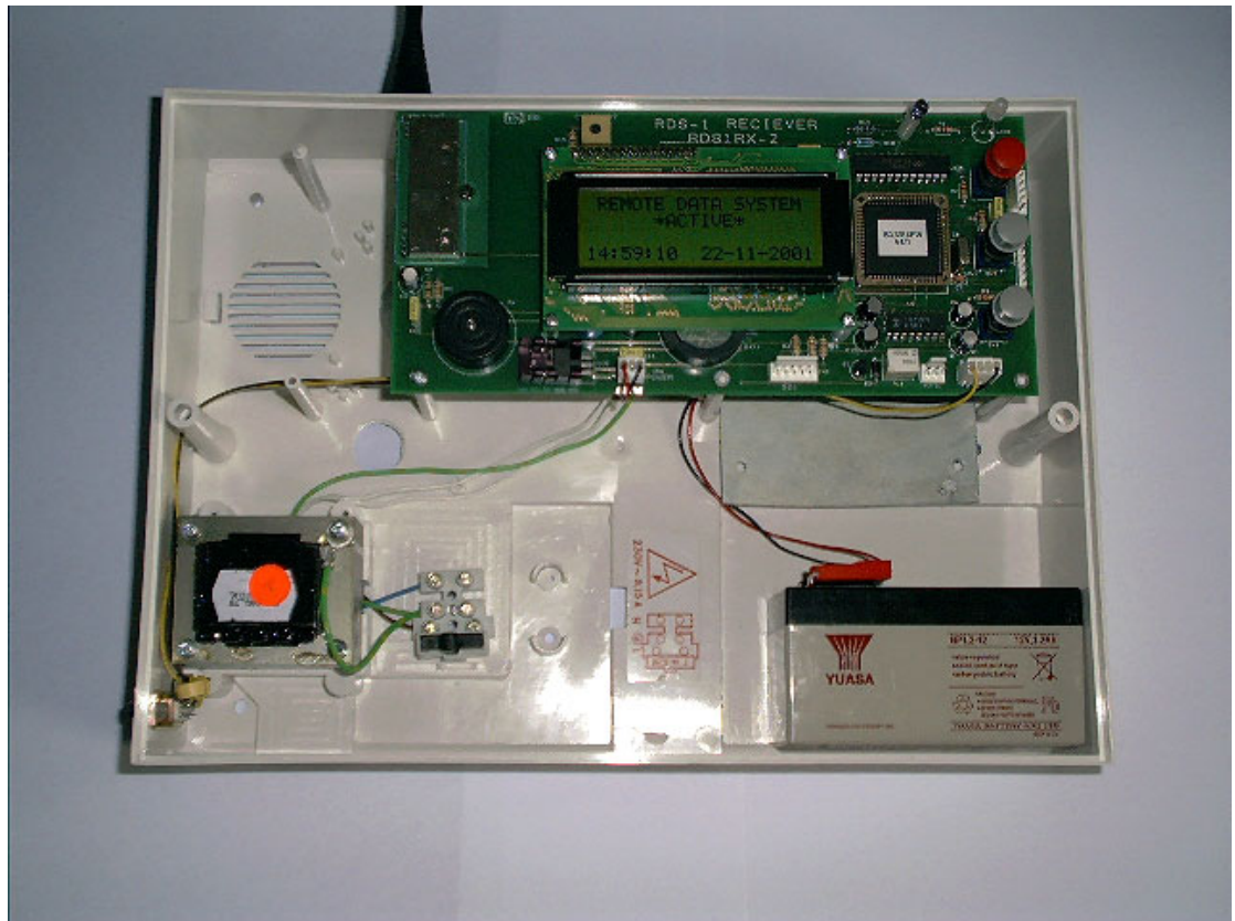
RDS RECEIVER INSIDE VIEW
