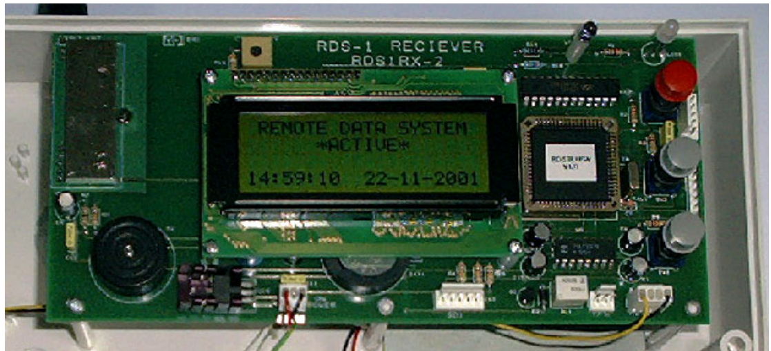
RDS RECEIVER INSIDE VIEW OF MAIN PCB
