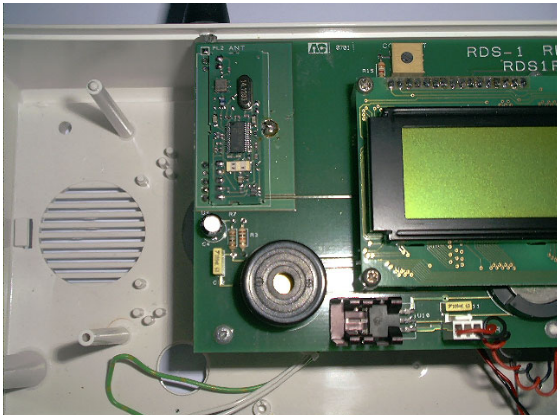
RDS RECEIVER INSIDE VIEW OF PCB WITH RF MODULE SCREEN REMOVED
