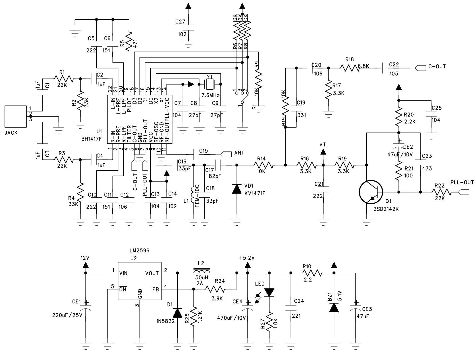
Auto FM Transmitter &amp; Charger SCH
