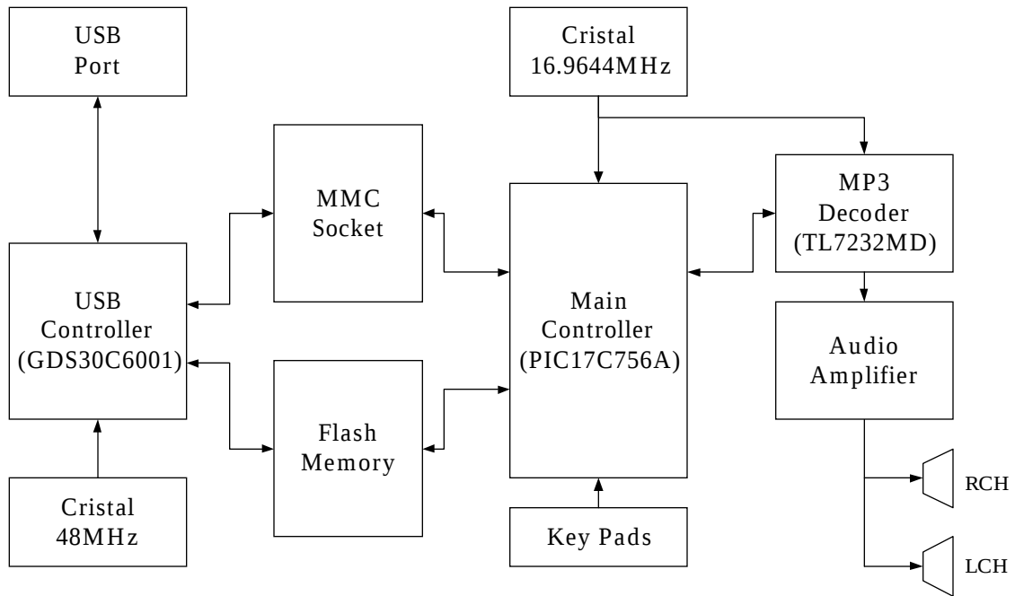
(DMP-2000L Block diagram)
