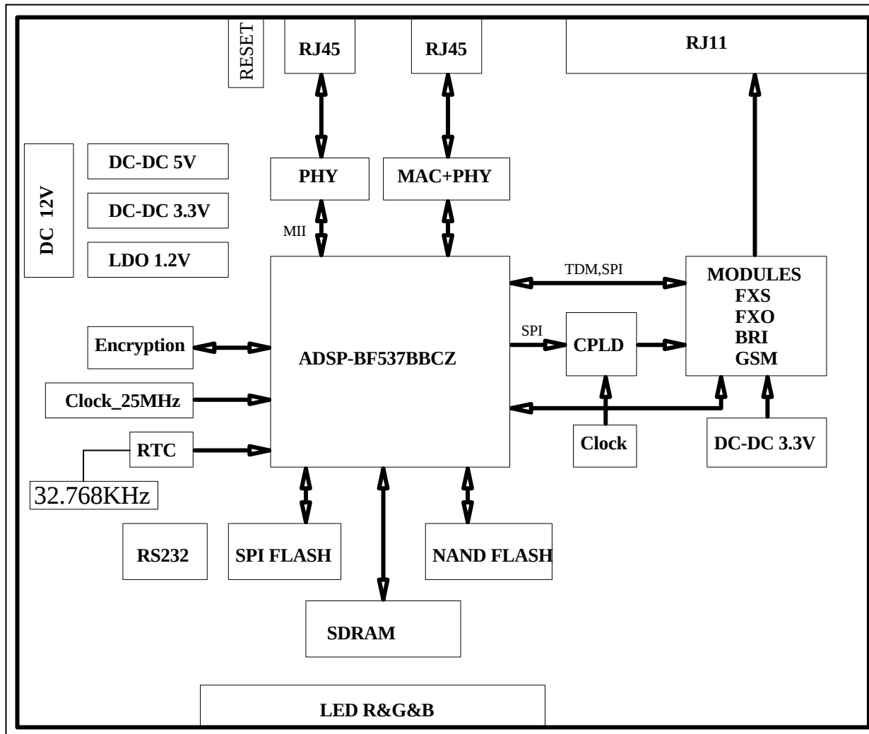
IPV20 System block diagram
