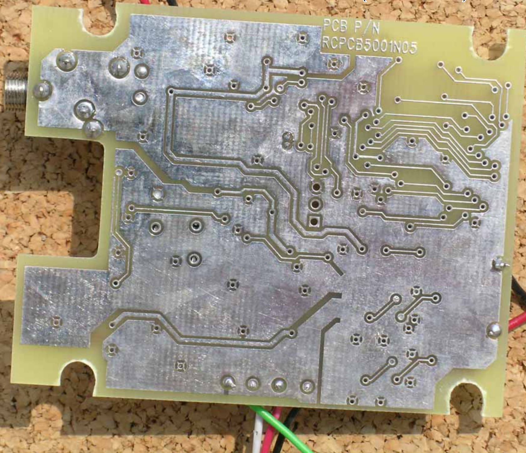
PCB (bottom)
