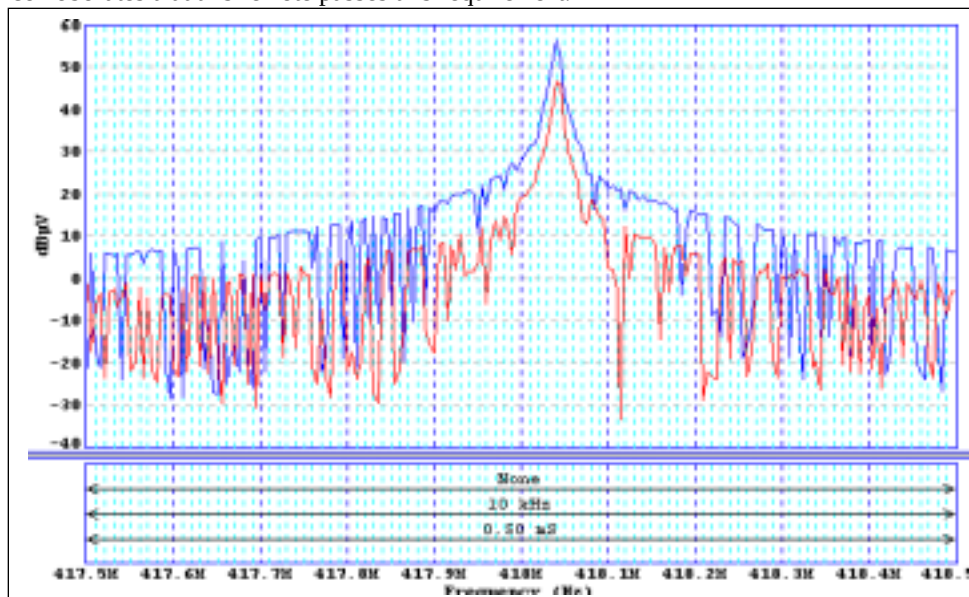
Fig. 1 Fundamental spectrum of the remote. Blue trace was obtained with the device oriented for maximum power with the vertically polarized antenna at 1-m altitude.
