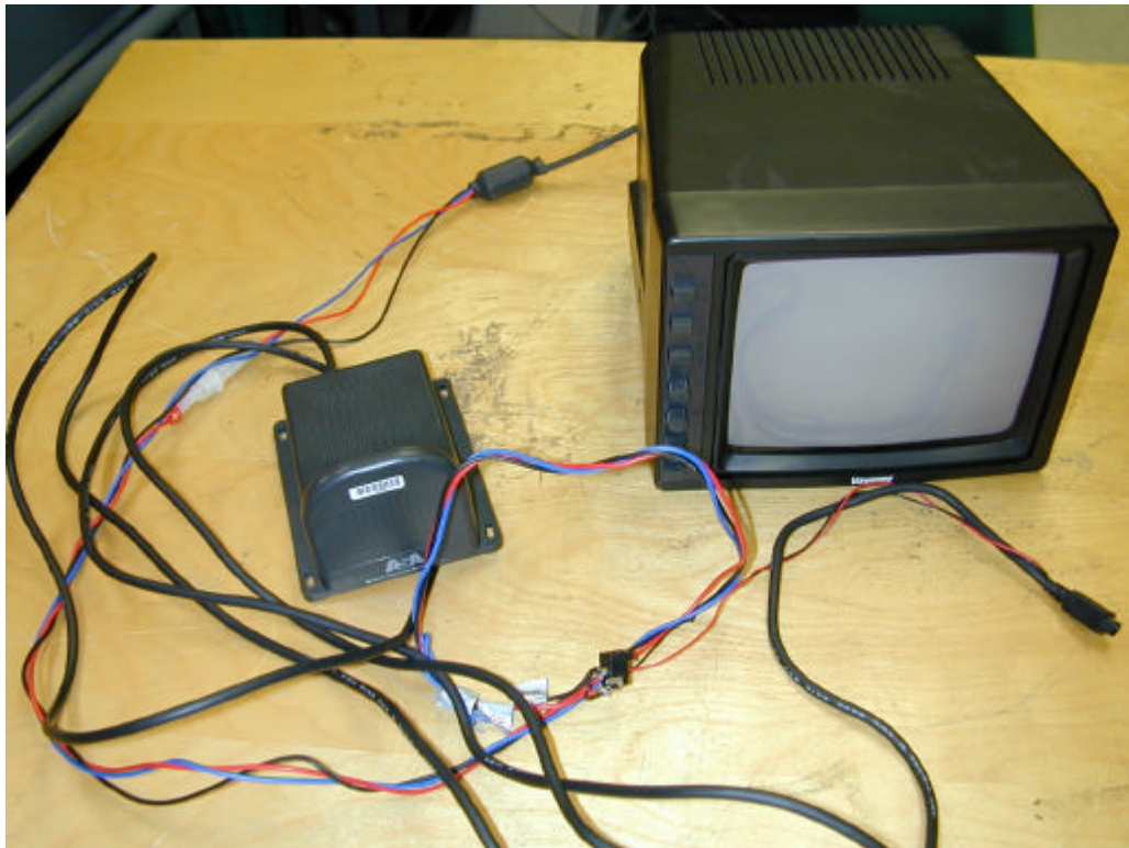
Receiver And NTSC Monitor
