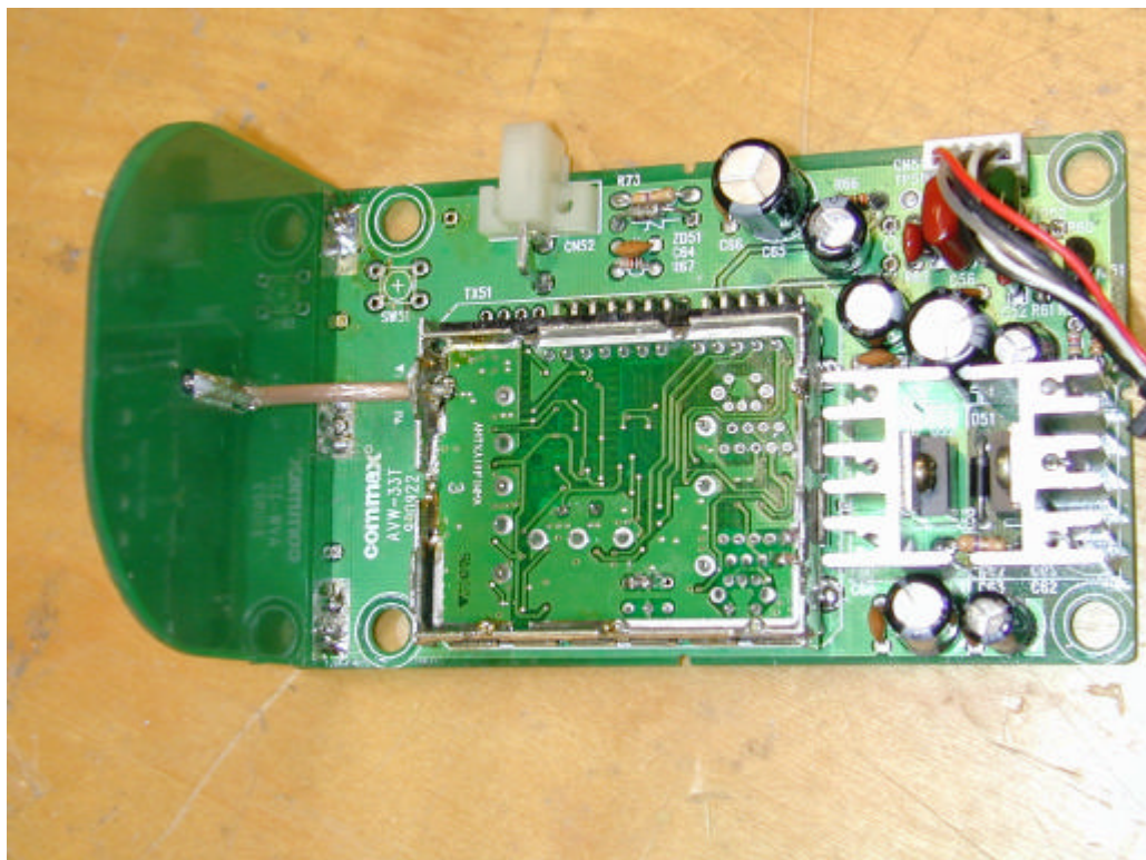
EUT PCB Component View 2
