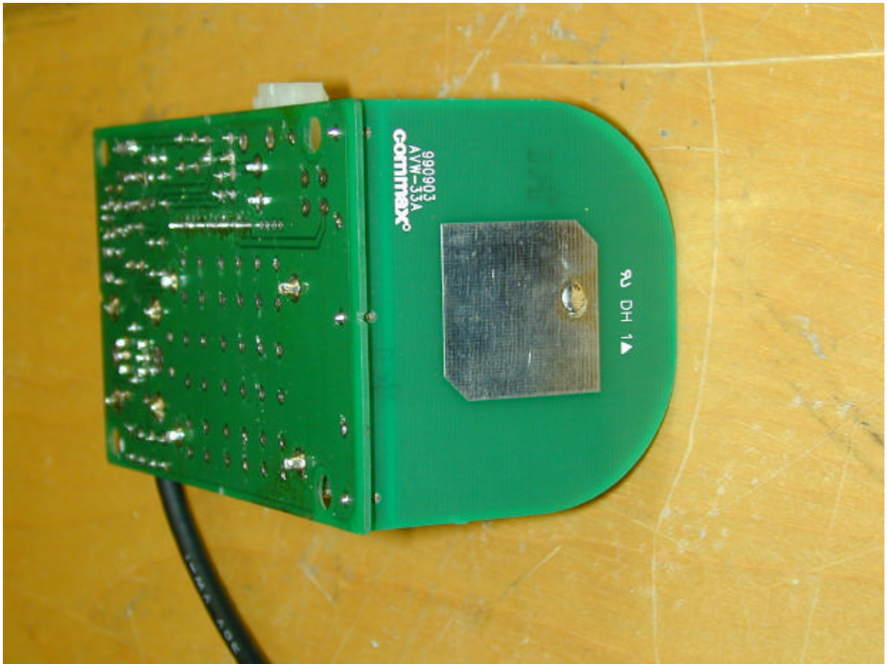
EUT Antenna View
