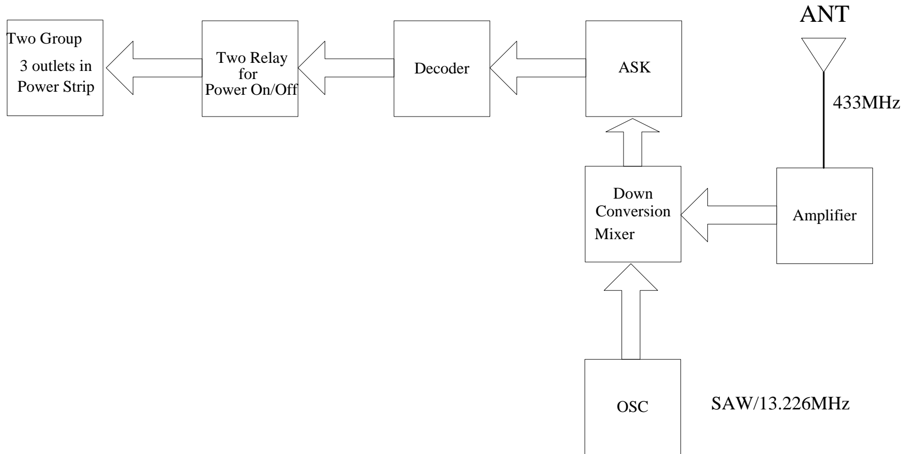
Block diagram of Receiver SPP5107C
