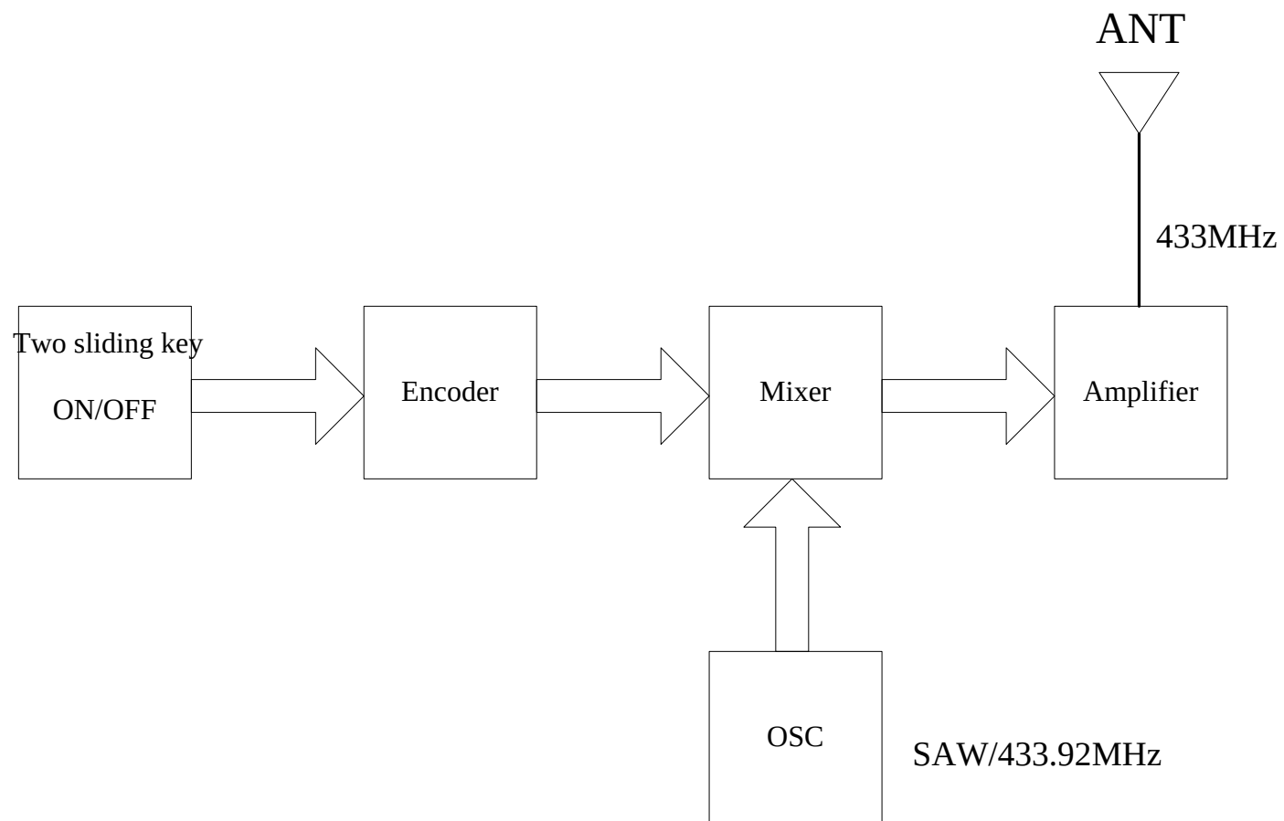
Block diagram of Transmitter RC-07
