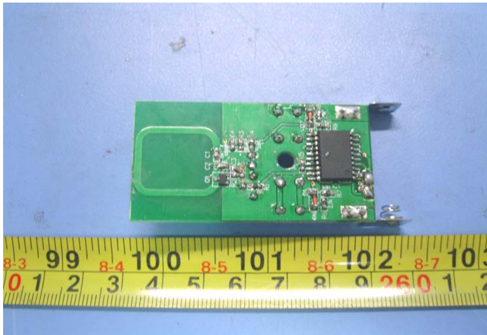
PCB-Front View
