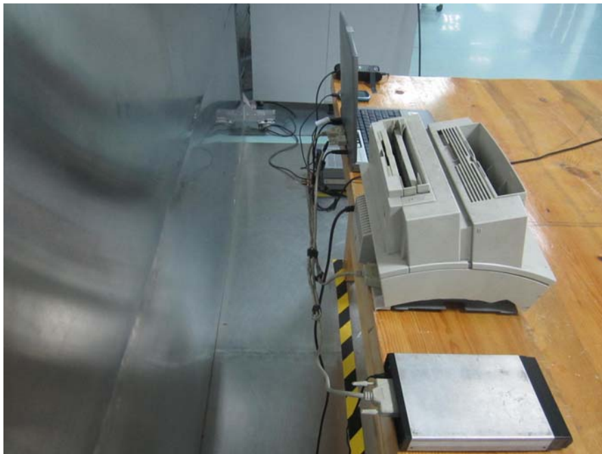
Conducted Emission (Downloading) - Side View
