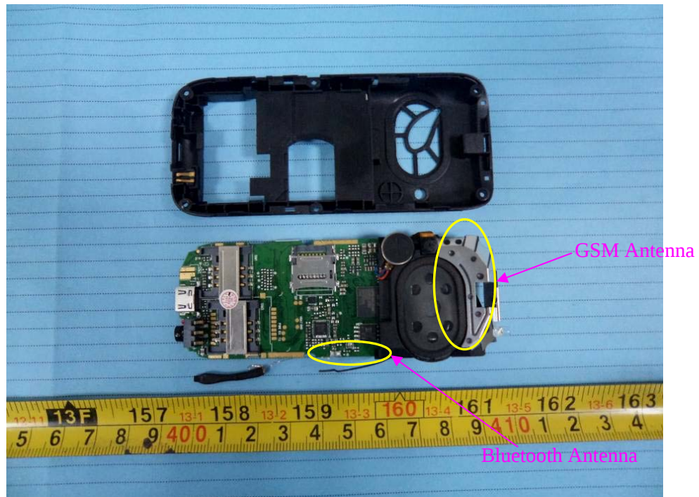
EUT – Main Board Top View
