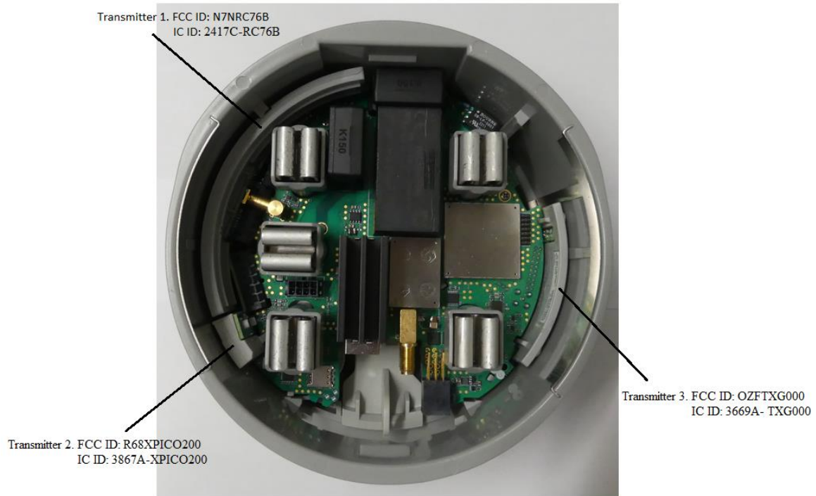
Front View
