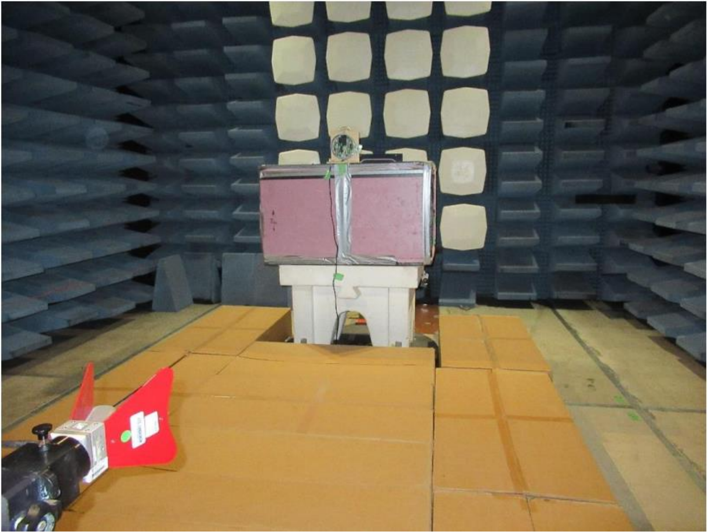
Emissions Test Setup – Intentional Radiated Emissions 1 – 18GHz
