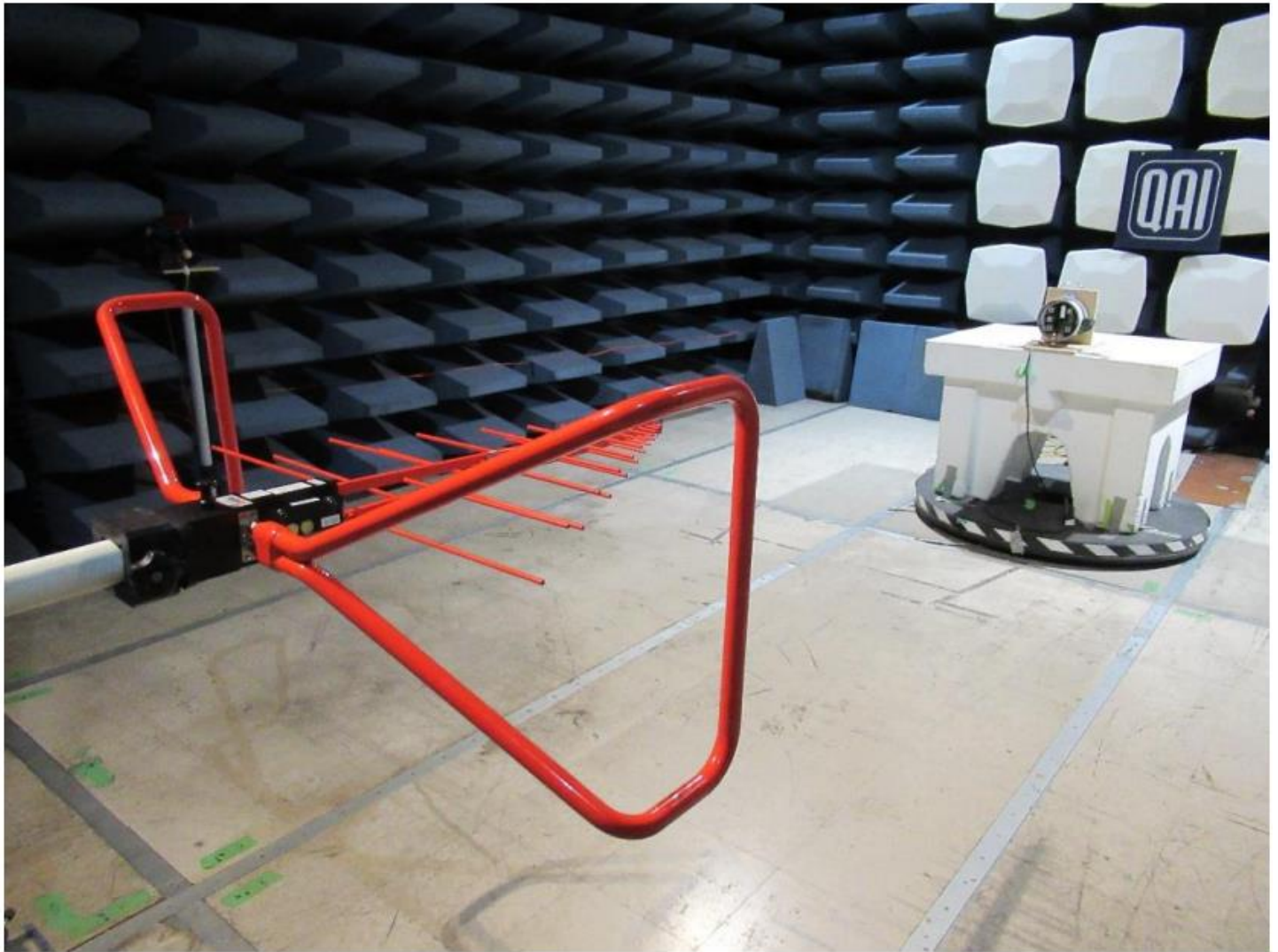
Emissions Test Setup – Unintentional Radiated Emissions 30 – 1000MHz
