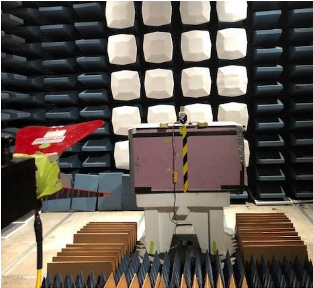
Emissions Test Setup – Intentional Radiated Emissions 1000 - 10000 MHz
