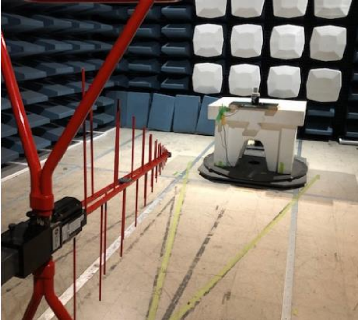
Emissions Test Setup – Unintentional Radiated Emissions 30 – 1000MHz
