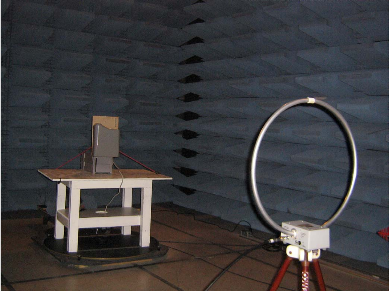
Emissions Test Setup – Intentional/Unintentional Radiated Emissions 0.009 – 30 MHz
