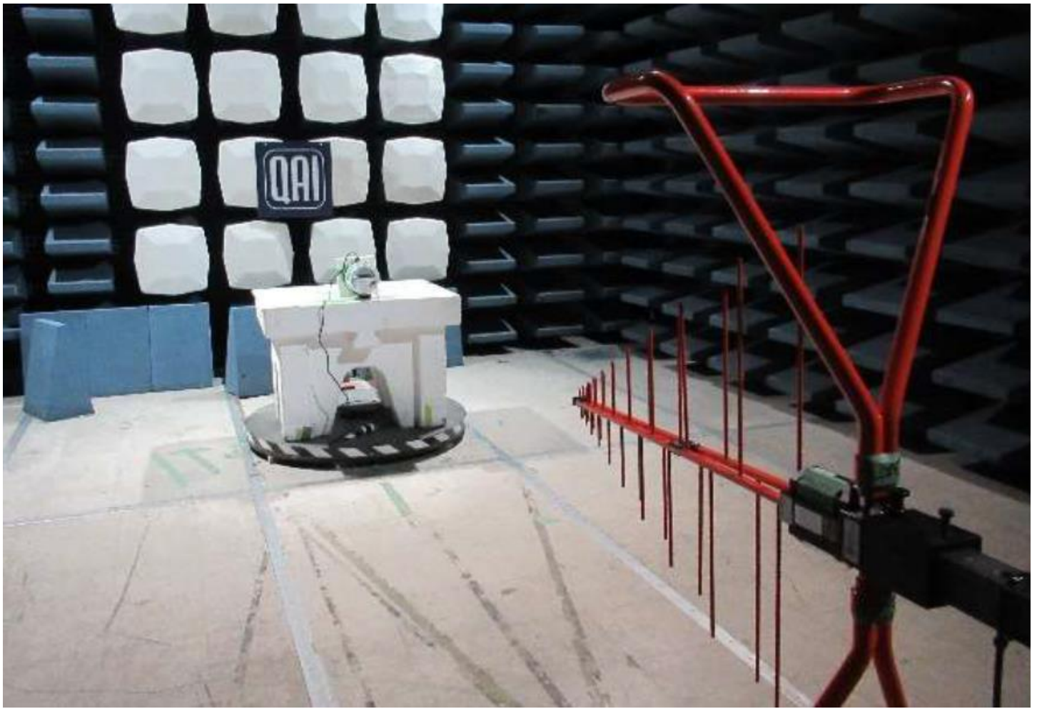
Emissions Test Setup – Unintentional Radiated Emissions 30 – 1000MHz
