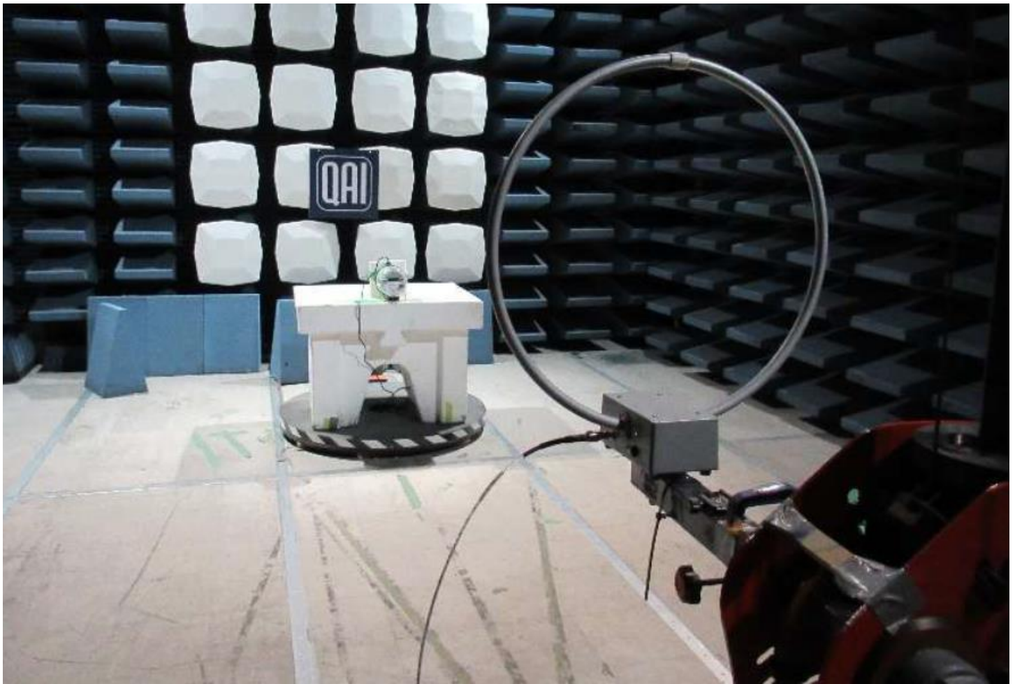
Emissions Test Setup – Unintentional Radiated Emissions 10kHz – 30MHz
