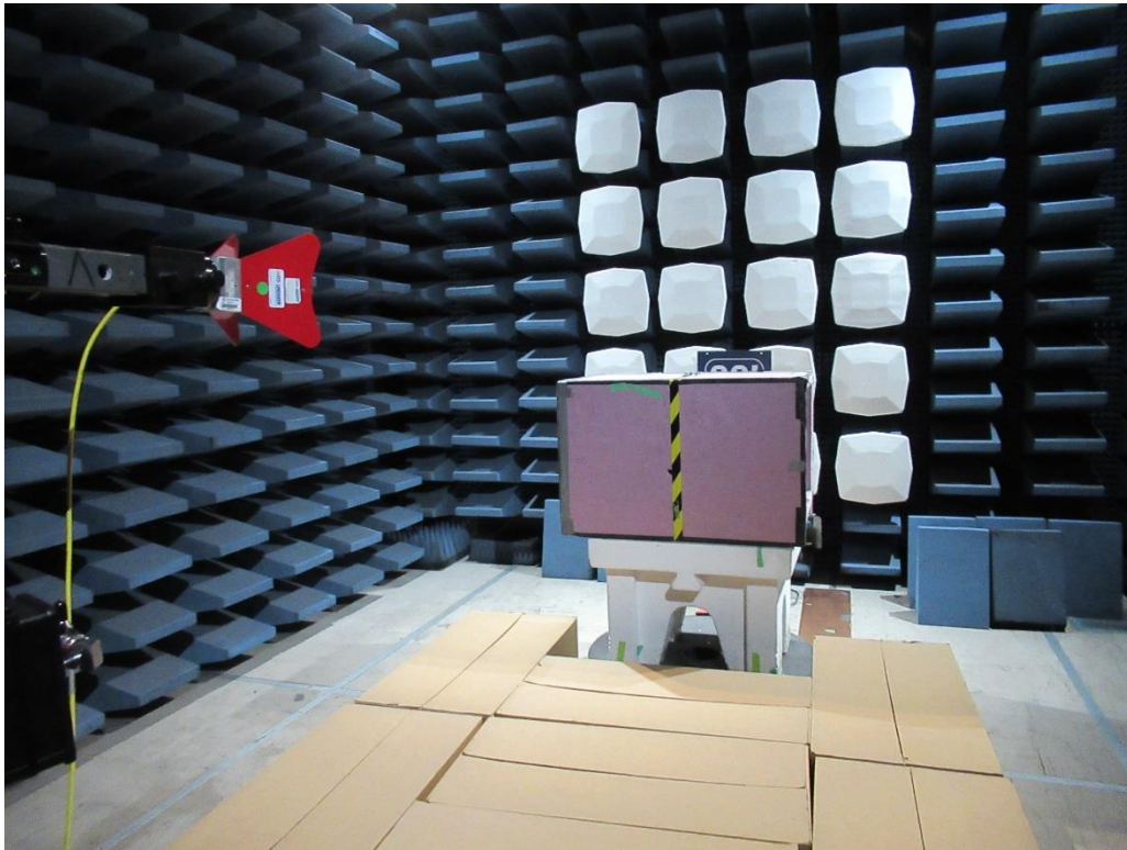
Emissions Test Setup – Intentional Radiated Emissions 1 – 10GHz
