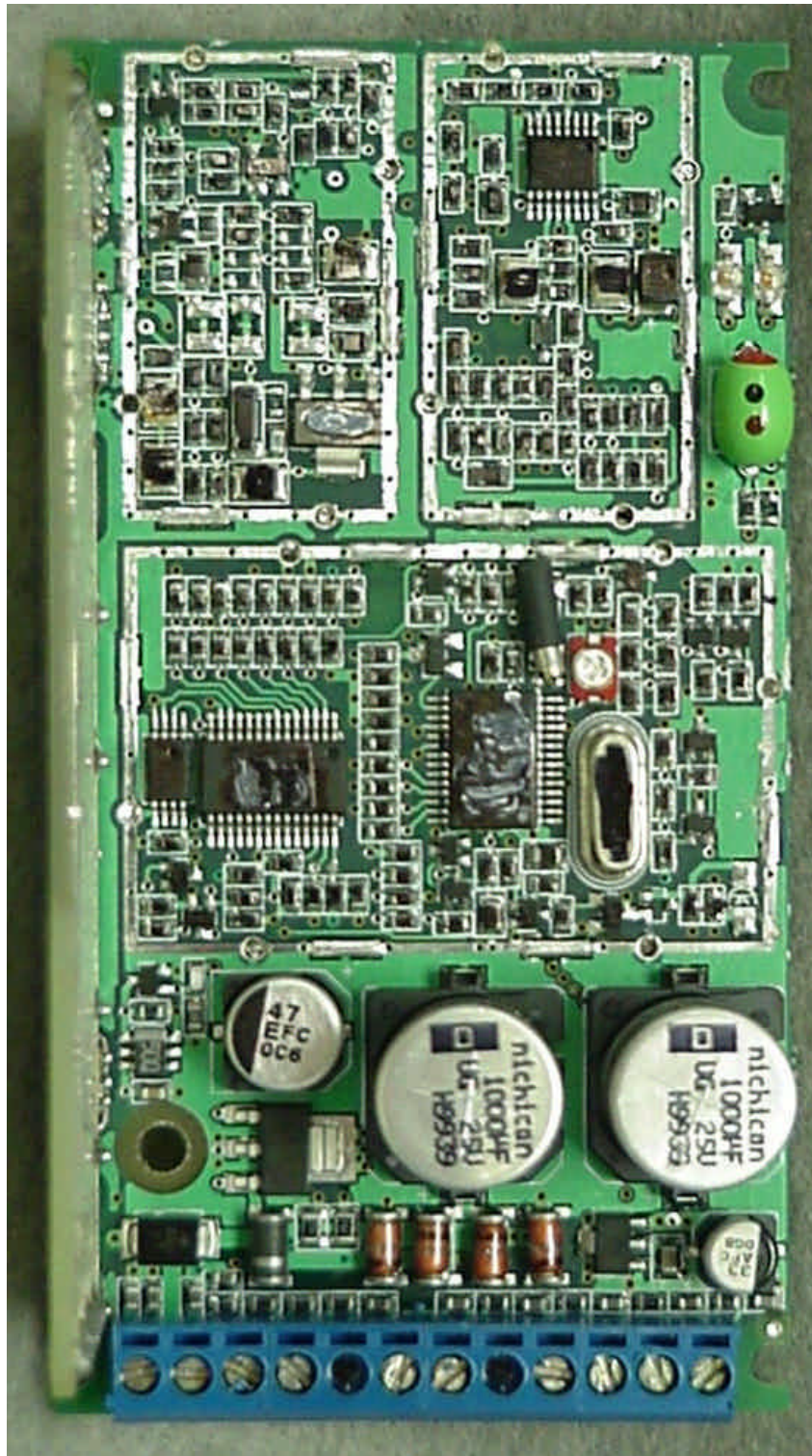
Photo 5. EUT, Top View of Board, Shields Removed
