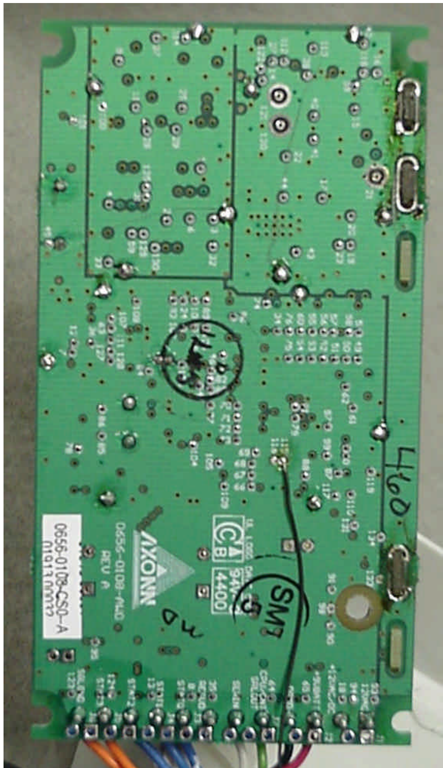
Photo 6. EUT, Bottom View of Board
