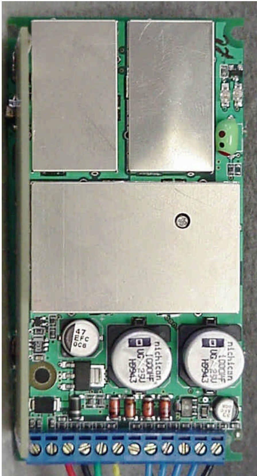
Photo 4. EUT, Top View of Board
