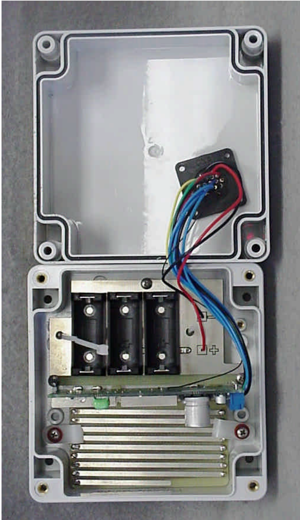
Photo 3. EUT, Internal View Cover Removed
