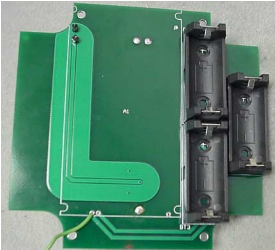
Photo 5. EUT, Bottom View of Antenna Board
