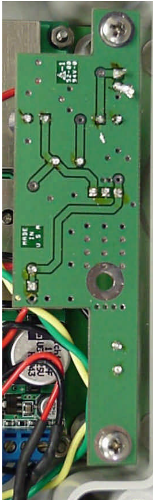
Photo 8. EUT, Bottom View of +9V Regulator Board
