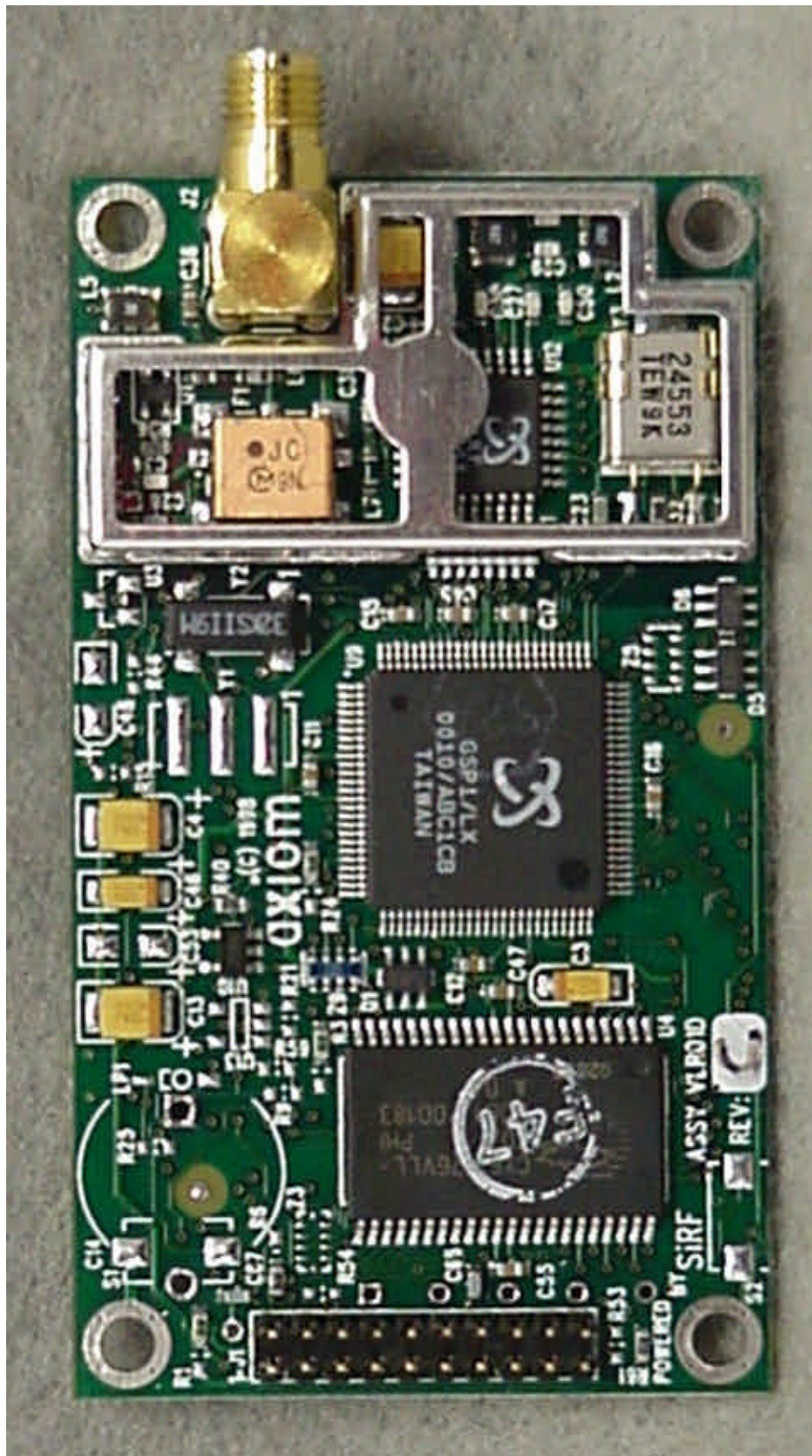
Photo 10. EUT, Top View of GPS Receiver (Shield Removed)
