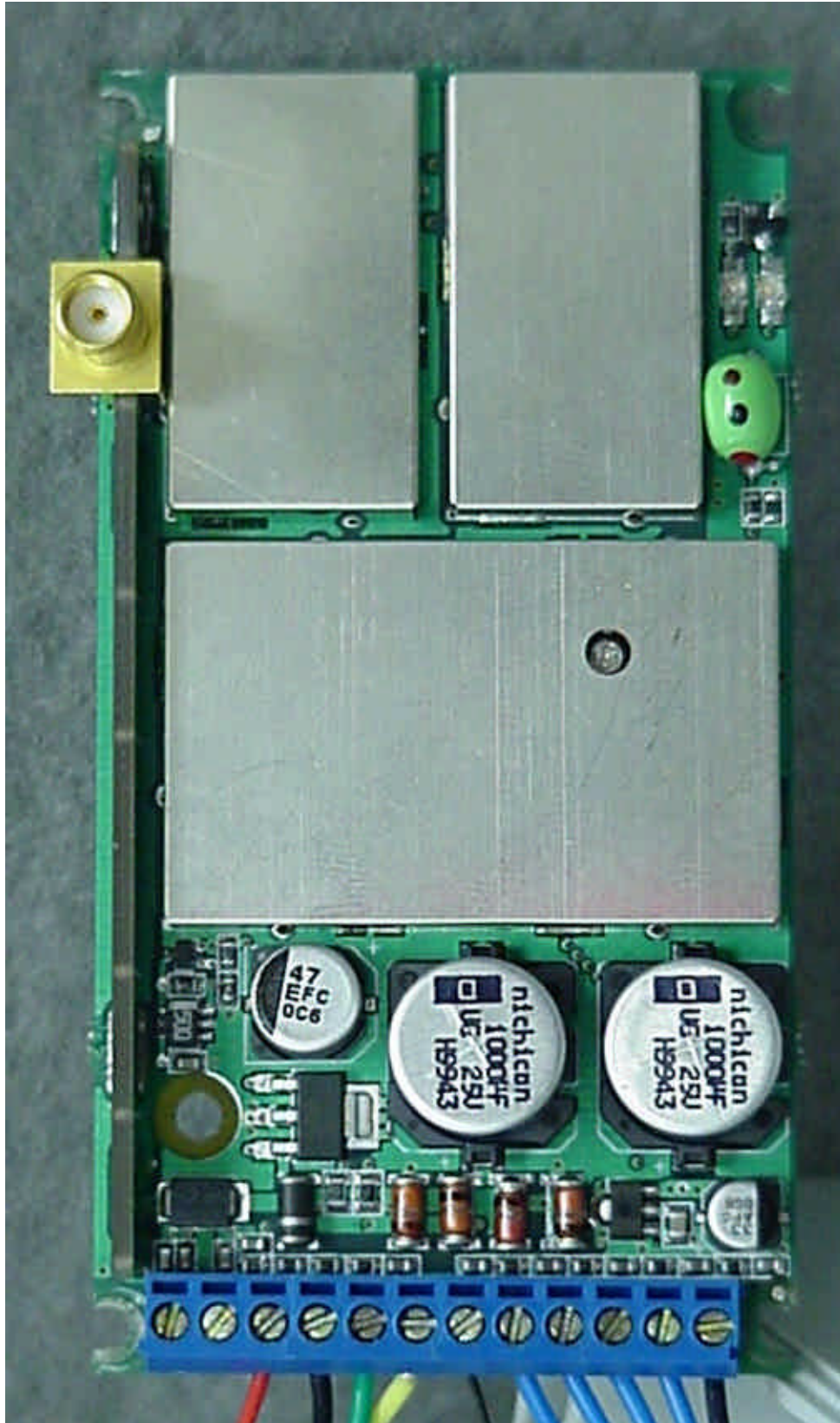
Photo 17. EUT, Top View of Transmitter Board
