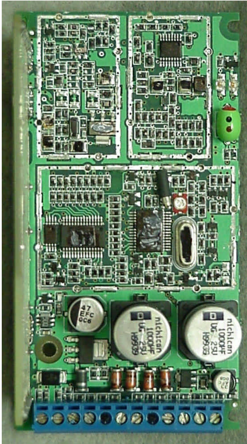
Photo 18. EUT, Top View of Transmitter Board, Shields Removed
