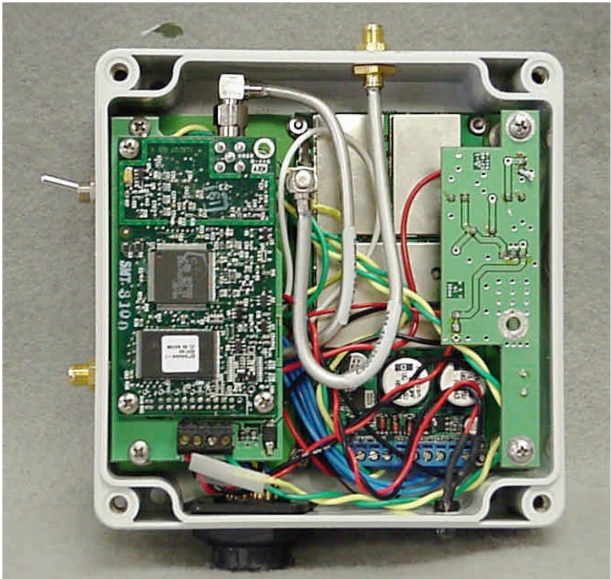
Photo 6. EUT, Internal View Cover Removed
