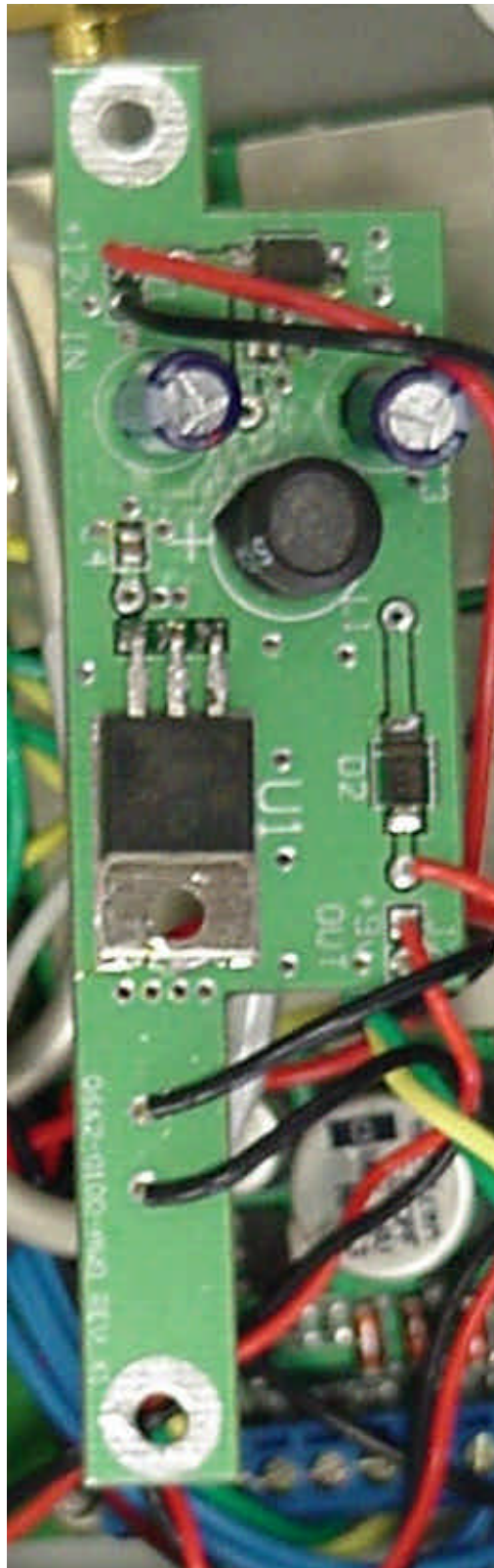
Photo 7. EUT, Top View of +9V Regulator Board
