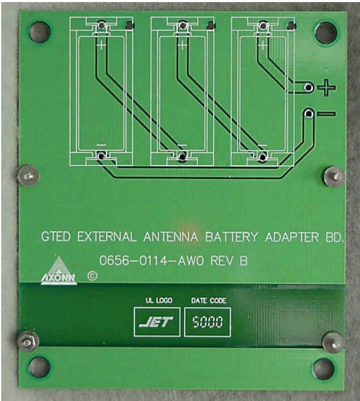
Photo 15. EUT, Top View of Battery Assembly Board, Transmitter Removed
