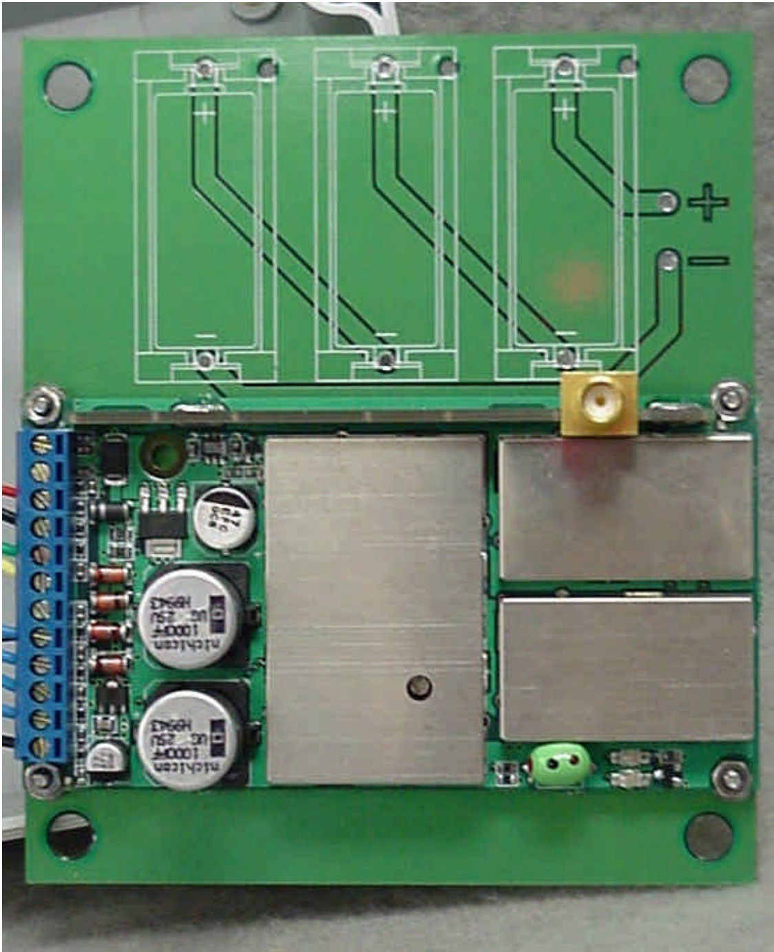
Photo 14. EUT, Transmitter and Battery Board Assembly
