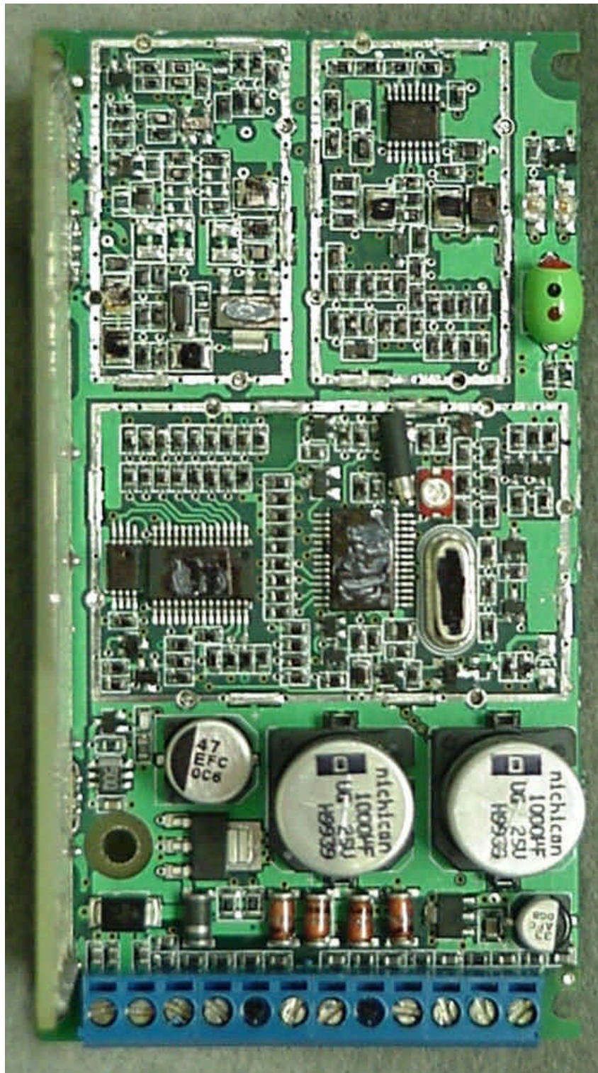
Photo 6. EUT, Top View of Board, Shields Removed
