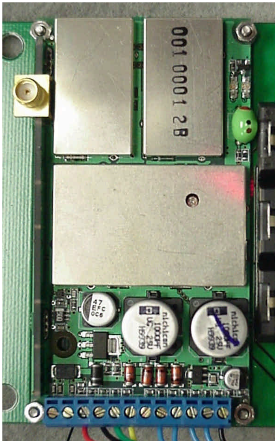
Photo 5. EUT, Top View of Board
