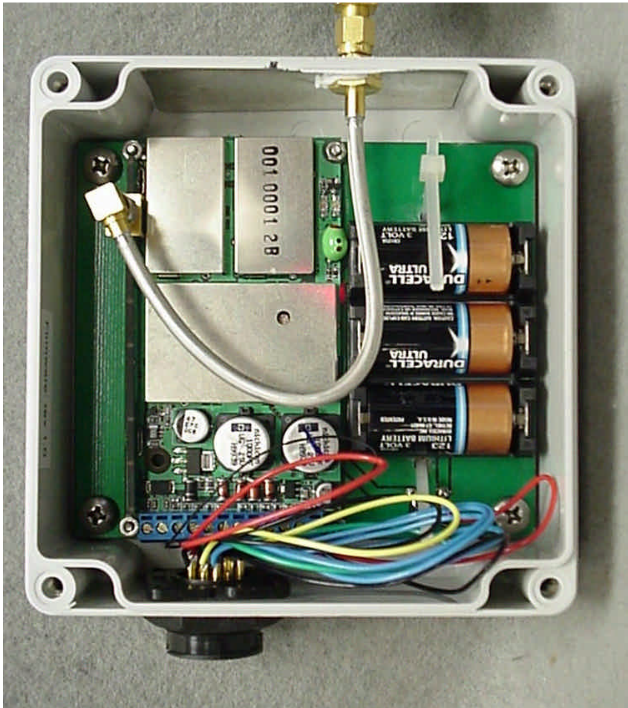
Photo 4. EUT, Internal View Cover Removed
