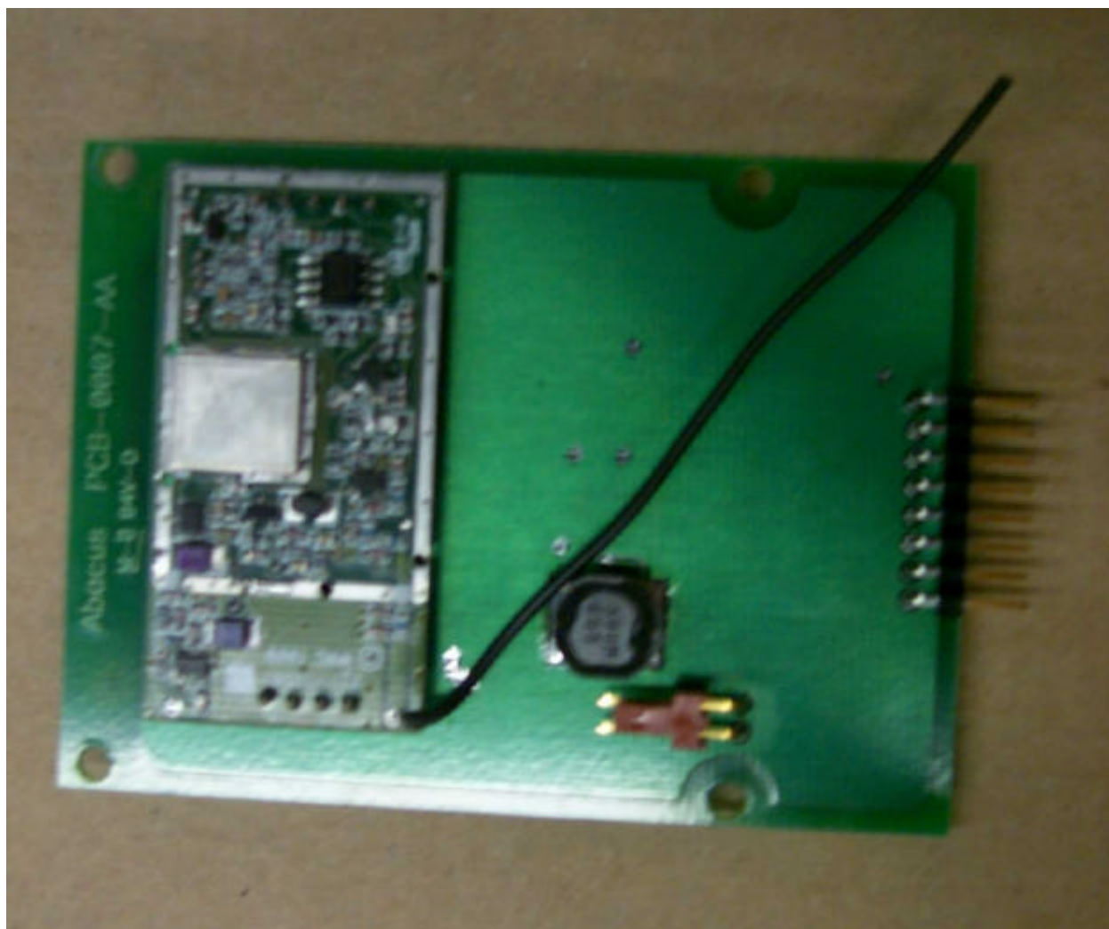
Abacus Controls Inc. Remote I A Series Board photo side 1
