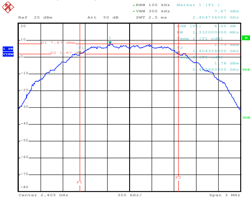
Figure 3. Plot of the 6dB Bandwidth (Conducted)
