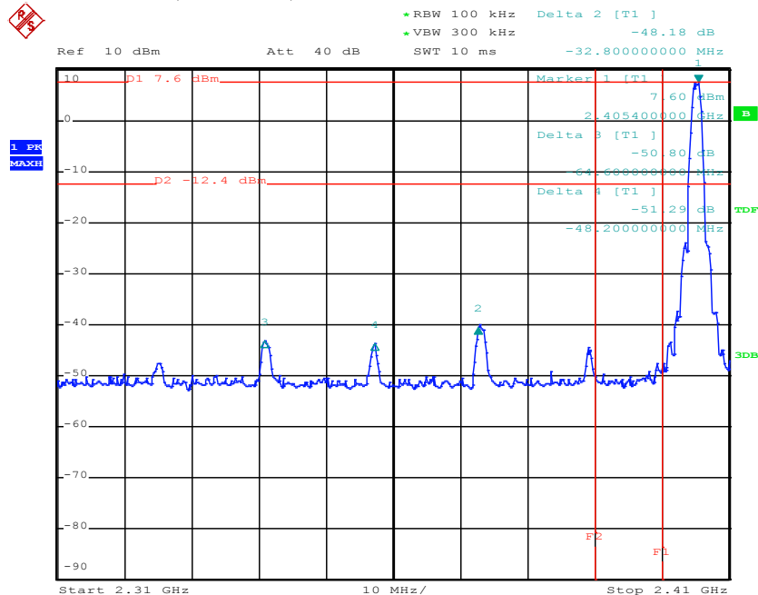
Figure 4. Plot of the Band Edge (Conducted)
