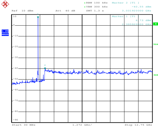
Figure 6. Plot of the Spurious RF conducted emissions
