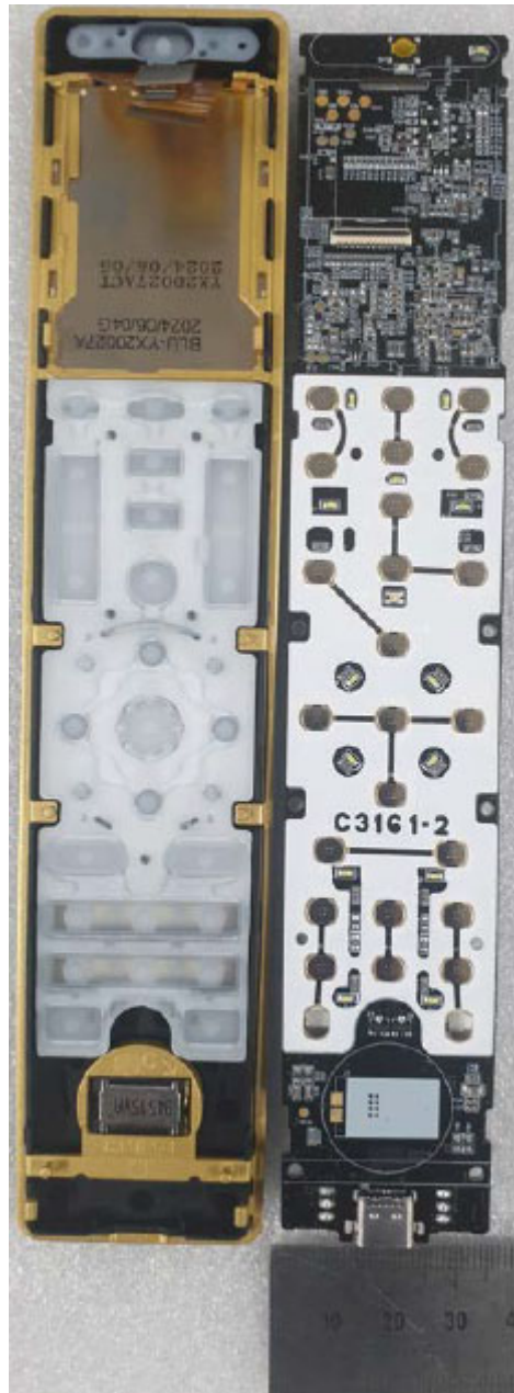
< Main Top View #2 >
