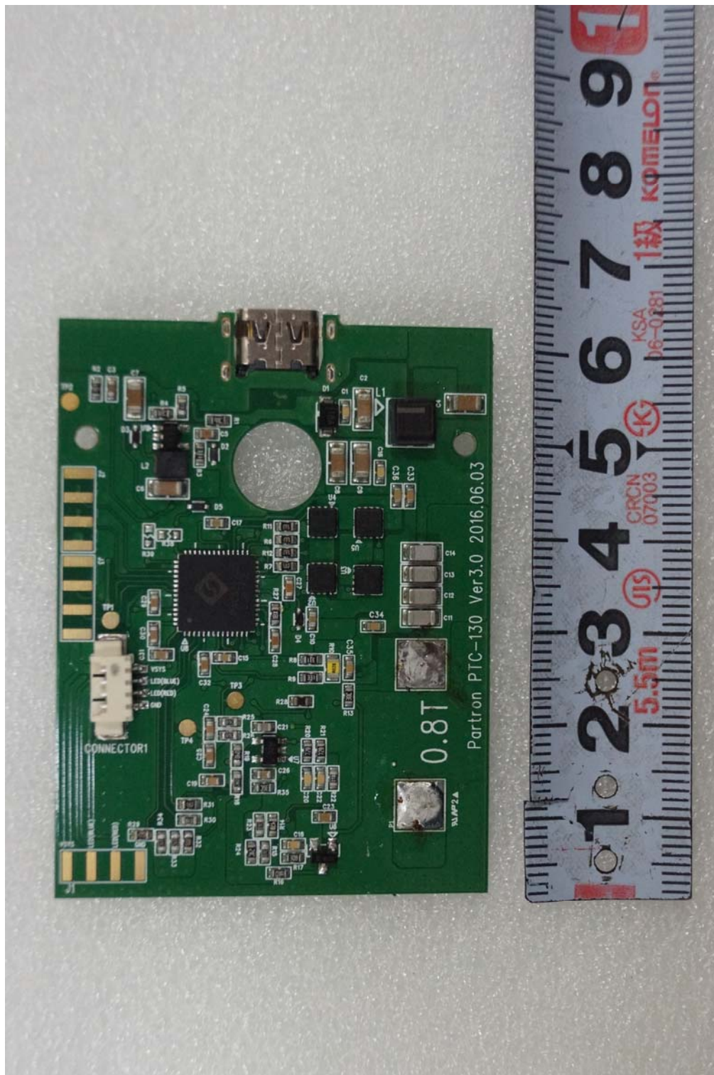
< Power input board top view >
