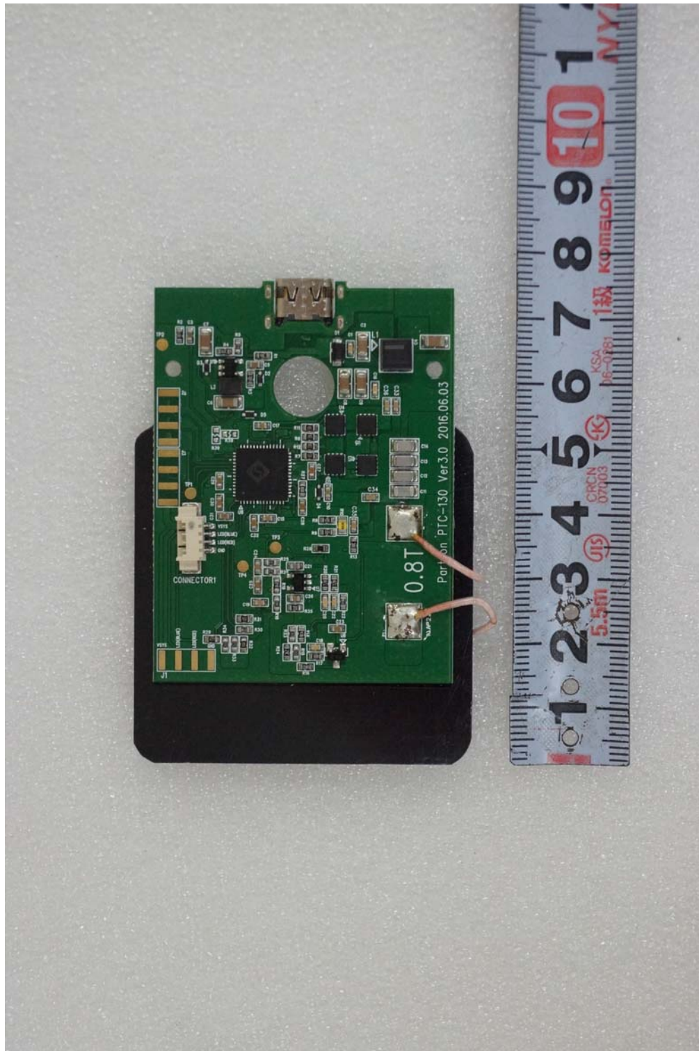
< Charger Part top view >
