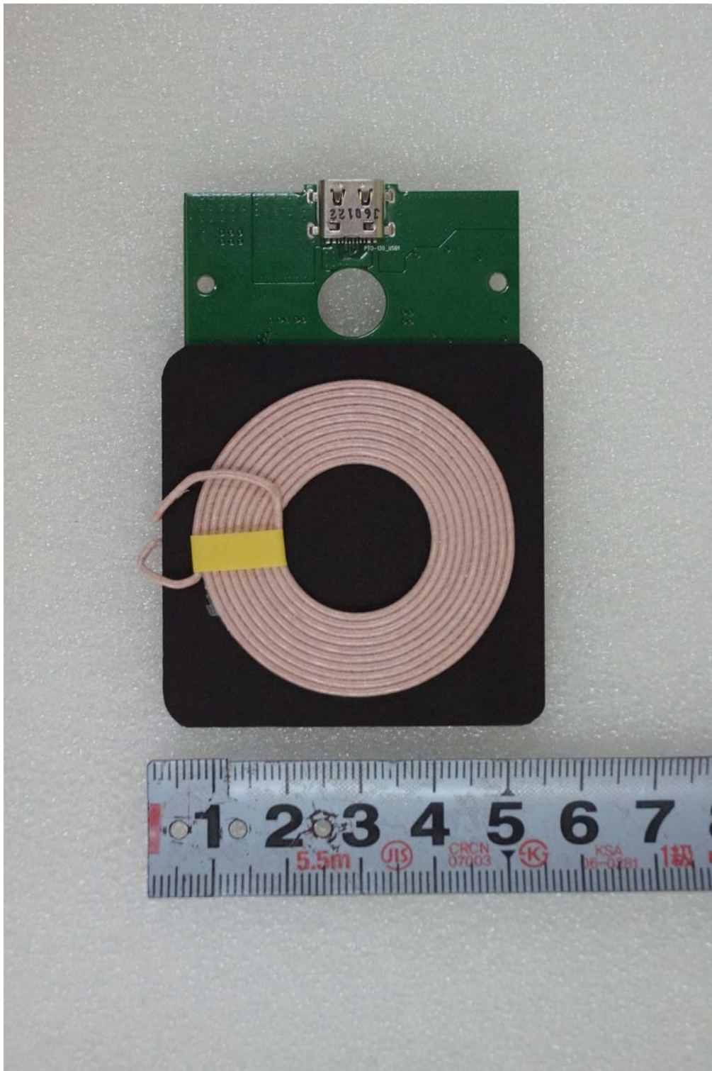
< Charger Part bottom view >
