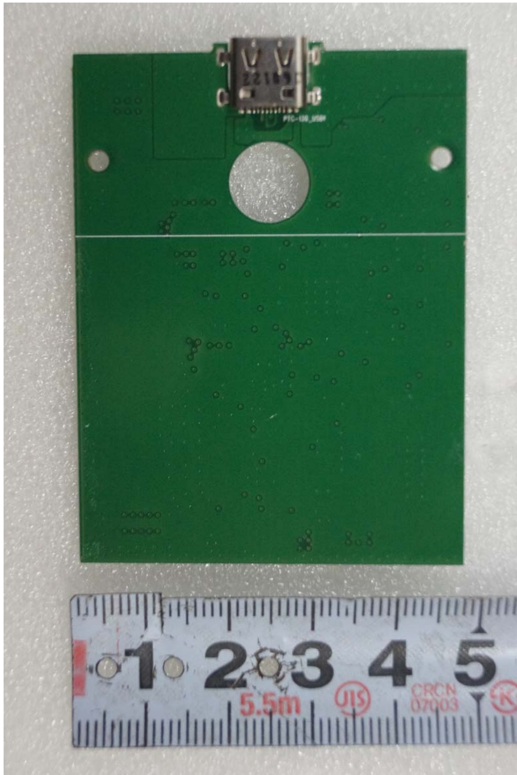
< Power input board bottom view >
