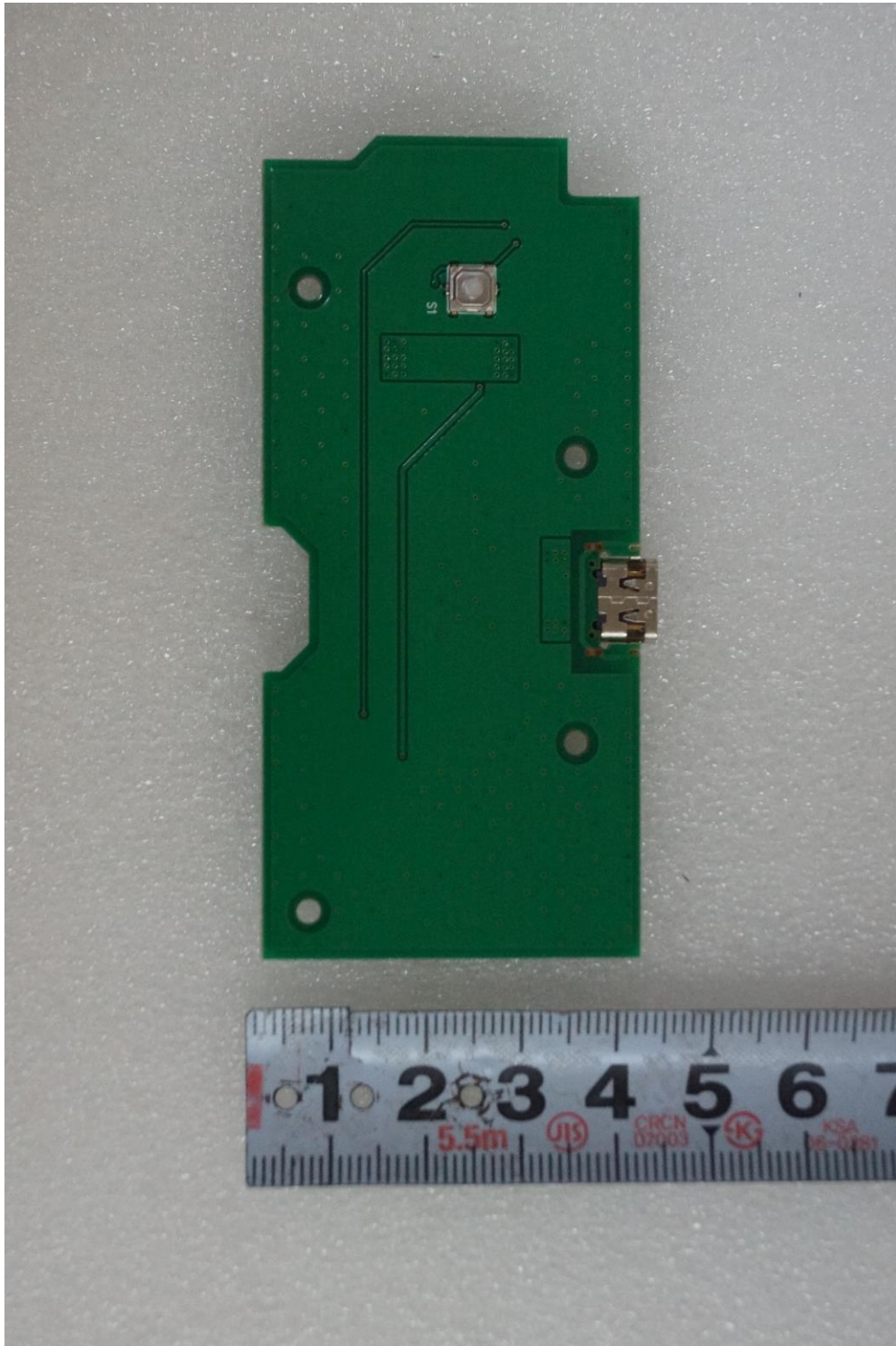
< USB charging board bottom view >
