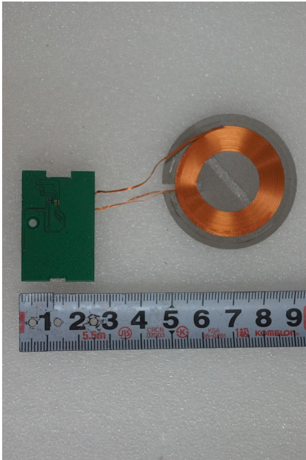
< wireless charger Rx module board bottom view >
