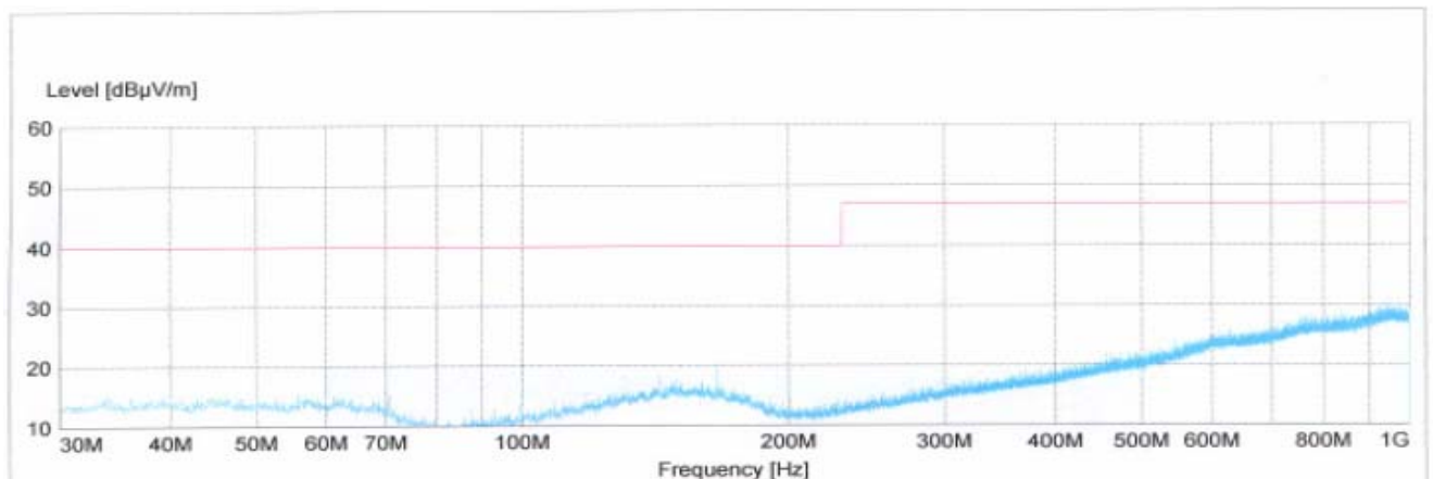
< Fig 6. Radiated emission result >
