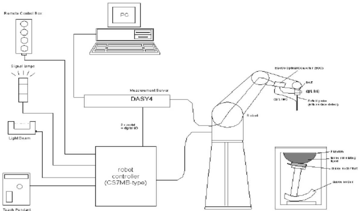
Fig 2. SAR Measurement System Setup
