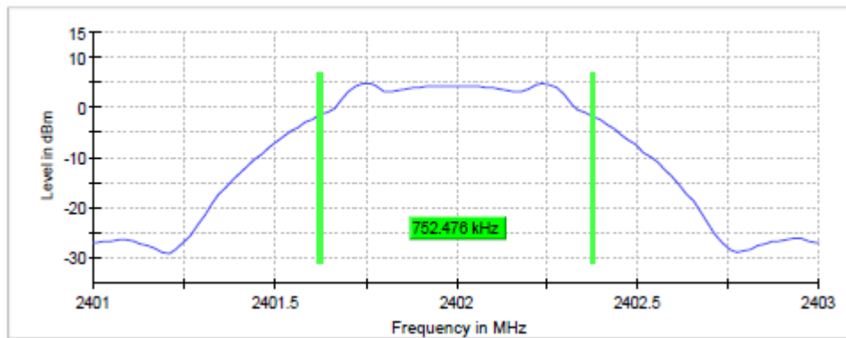
6 dB Bandwidth Plot on Configuration : Lowest channel (2 402 MHz)
