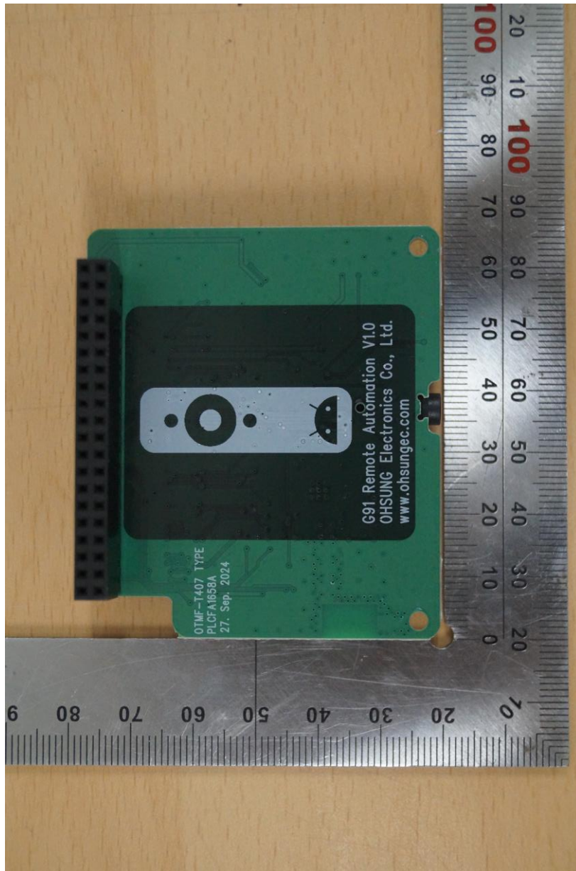
< Rear view >
