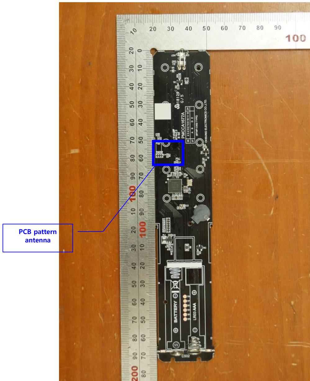
< Main board bottom view >
