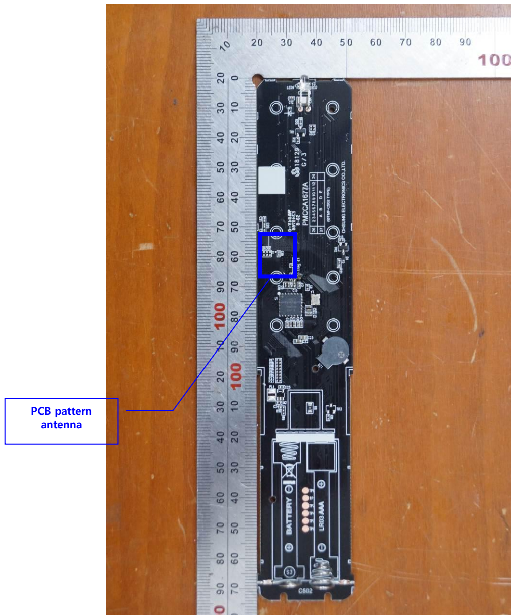
< Main board bottom view >
