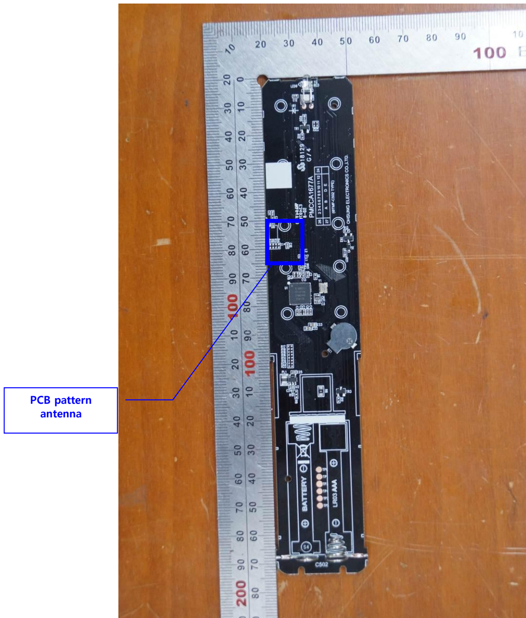
< Main board bottom view >
