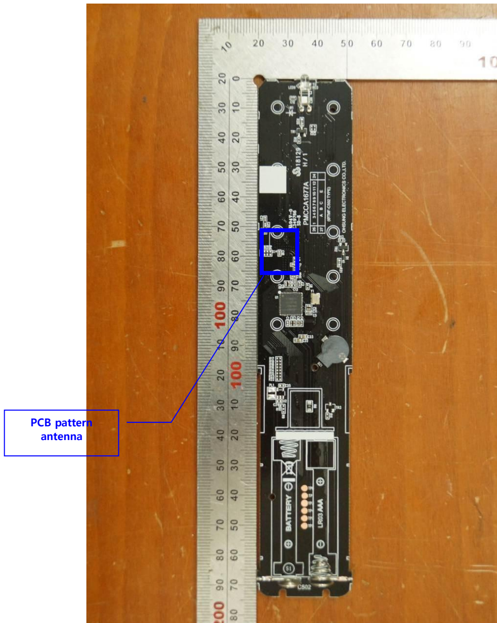
< Main board bottom view >
