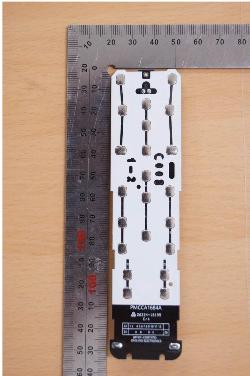
< Main board Top view #1 >
