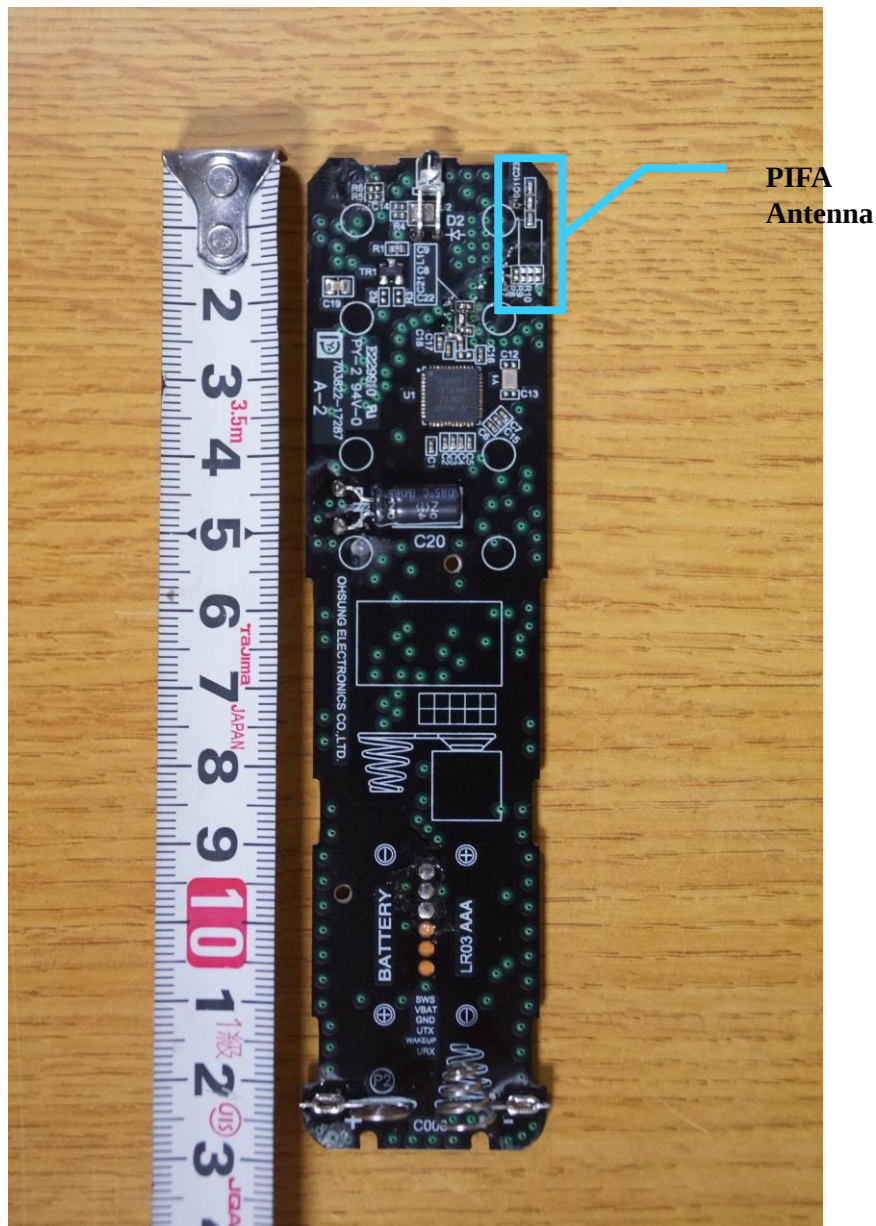
< Main board bottom view >
