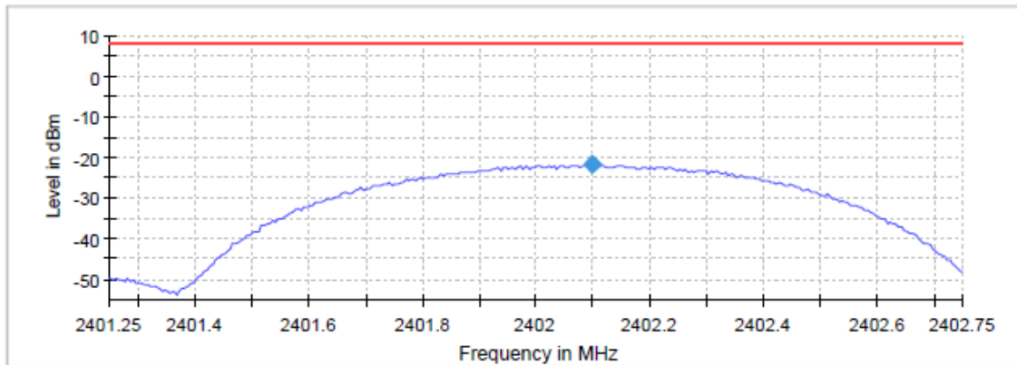
Power Density Plot on configuration : Lowest channel (2 402 MHz)
