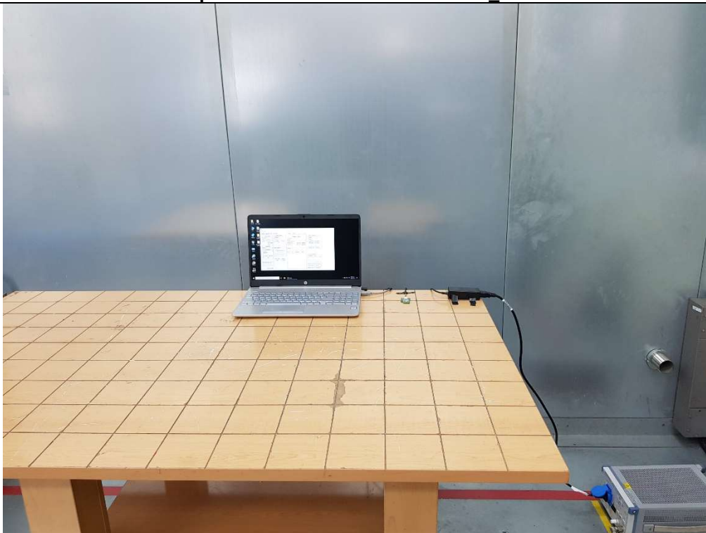
AC power line conducted emissions_Rear
