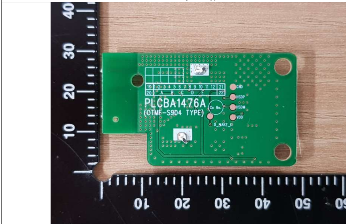
EUT – Rear
