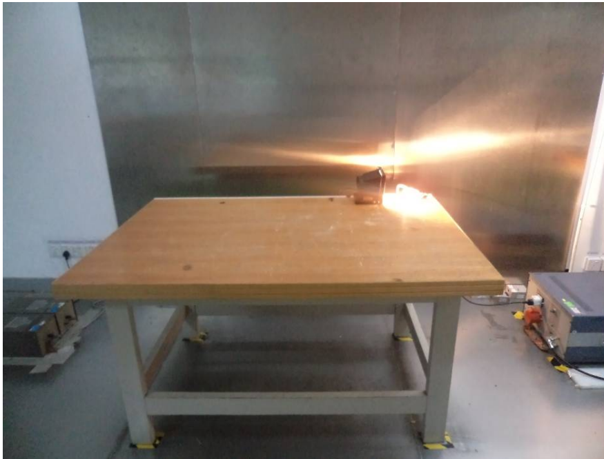
Conducted Emissions - Front View (Incandescent Lamp)
